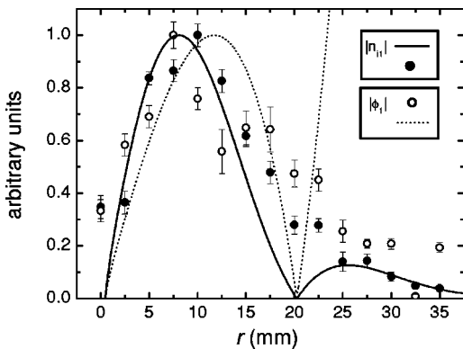
FIG. 11. Radial profiles of |\phi_1| and |n_{i1}| with B_z = 0.05 T. The lines are the predictions for the n = 1 centrifugal instability.
