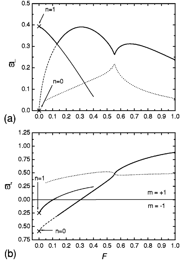
FIG. 3. Dispersion curves of (a) the normalized growth rate \varpi^i and (b) the normalized frequency in the frame of the ion fluid \varpi^r , for m=1 plotted against normalized axial wave number F . Plasma conditions are taken from Table I. The solid line is the most unstable mode envelope, and the crosses represent the eigenmodes of the centrifugal instability of an unbounded plasma column ( Y \rightarrow \infty ).
