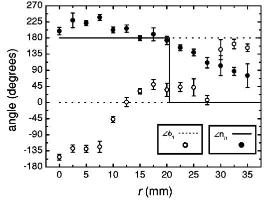
FIG. 8. Plot of the radial phase profile of the floating potential and ion density, fitted such that \angle n_i = 180^\circ at r = 15 mm. The lines are the predictions for the centrifugal instability ( k_z = 0 ) with m = 1 , n = 1 .
