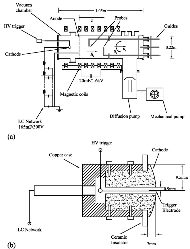
FIG. 1. (a) Schematic of the PCEN device and (b) schematic of the magnesium cathode.
