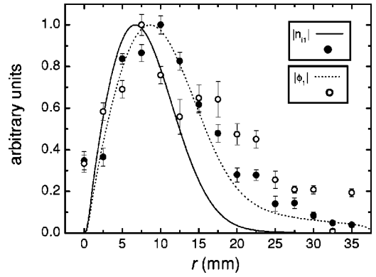
FIG. 12. Radial profiles of |\phi_1| and |n_{i1}| with B_z = 0.05 T. The lines are the predictions for the density-gradient driven instability.
