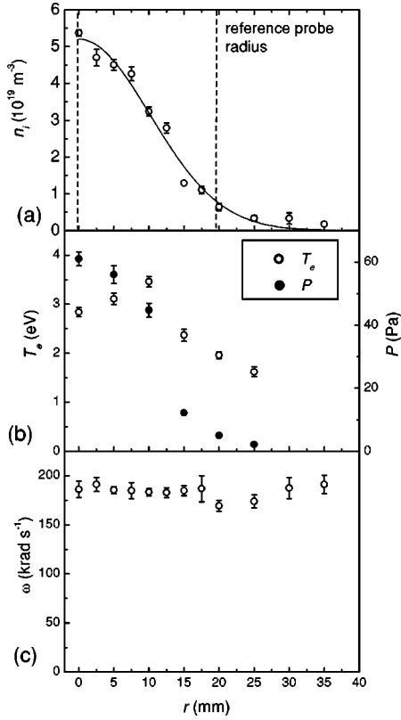
FIG. 7. Radial profiles of (a) ion density n_i , (b) electron temperature T_e (left axis) and total pressure P (right axis), and (c) instability frequency \omega with B_z = 0.05 T.
