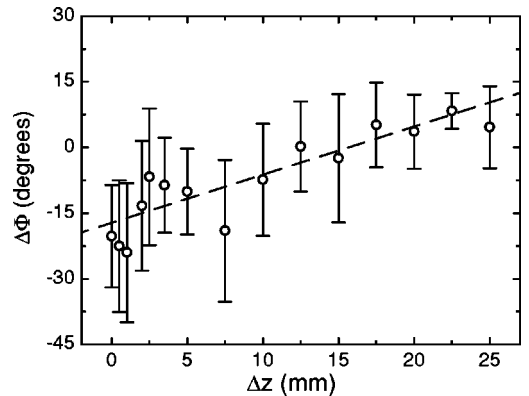
FIG. 13. Phase difference between the floating potential of probes separated by \Delta z and positioned 180^\circ apart in azimuth. A constant phase of 180^\circ has been subtracted from the phase measurements.
