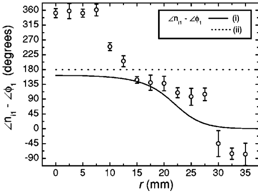
FIG. 10. Radial phase difference between the ion density and floating potential. The lines are the predictions of theory; case (i) is the density-gradient driven drift mode and case (ii) is for the n = 1 centrifugal instability.
