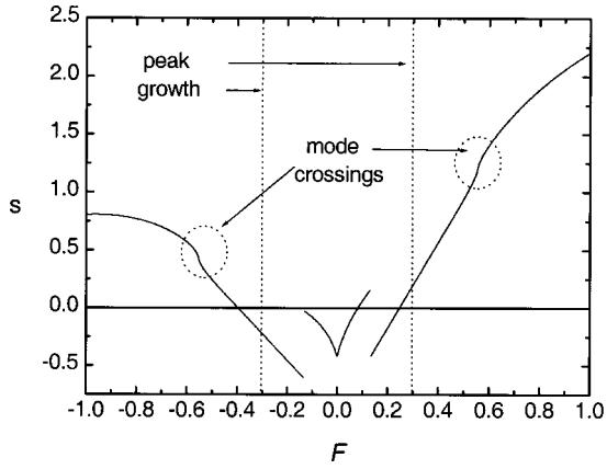
FIG. 4. Laboratory frame slip s = (\omega - \Omega_{i0})/\Omega_{i0} for the most unstable m=1 mode versus normalized axial wave number F .
