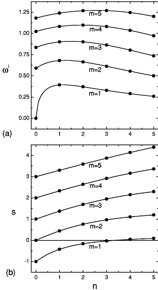
FIG. 2. Flute mode dispersion relation for different (m, n) modes as a function of radial eigenmode number n , for normalized plasma rotation frequency \Omega_{i0}=0.59 . (a) Plot of the normalized growth rate \omega^i and (b) plot of the slip in the laboratory frame s=(\omega-\Omega_{i0})/\Omega_{i0} .
