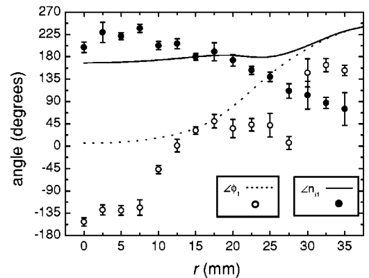
FIG. 9. Plot of the radial phase profile of the floating potential and ion density, fitted such that \angle n_i = 180^\circ at r = 15 mm. The lines are the predictions for the density-gradient driven drift mode ( k_z = 3.7 \text{ rad m}^{-1} ) with m = 1 .
