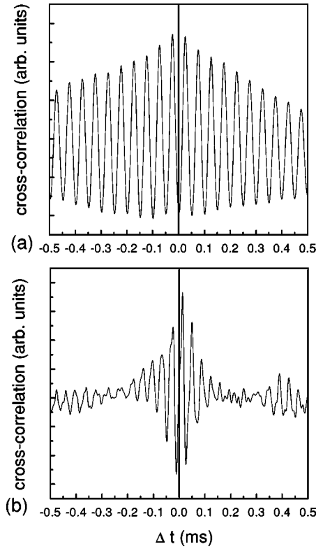
FIG. 6. Plots of the cross correlation of the floating potential measured from two probes located at the same axial position (150 mm from the anode mesh) and separated by 180^\circ in azimuth. In (a) the probes were located at a radial distance of r=22 mm from the geometric center. In (b) the probes were located at radial distances of r=5 and 35 mm.
