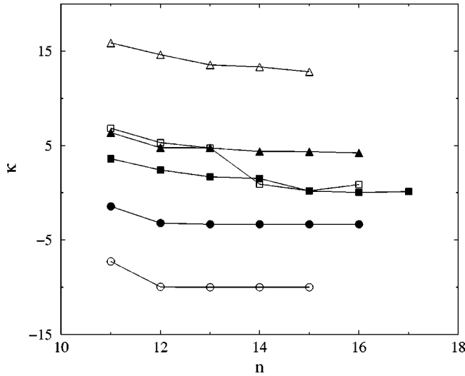
FIG. 2. Dependence of the constant \kappa on n when computed independently at each lattice site using Eq. (6). Symbols as in Fig. 1. Lines are connecting data and serve as guides to the eye.
