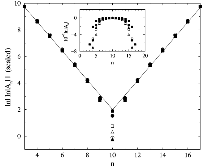
FIG. 1. Dependence of the double logarithm of the breather amplitude for different cases versus n . Note that curves are vertically shifted to observe a master curve in the tails. V_h , circles; V_m , squares; V_s , triangles. Open symbols, k=0.1 ; filled symbols, k=0.3 . The straight lines have slopes \pm \ln 3 . Inset: Dependence of the logarithm of the breather amplitude versus n for the same cases. Note the scale of the y axis.
