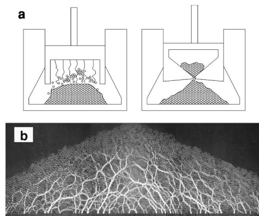
FIG. 1. Lower section: Setup of a two-dimensional pile (height \sim 30 cm and base length \sim 130 cm) of photoelastic disks created by a localized-source procedure. The pile is viewed between crossed polarizers, allowing one to see the underlying force structure. Bright regions correspond to the force chains. Upper section: Deposition procedures for triangular piles. Left picture shows raining technique, right shows the localized procedure. See text for more details.
