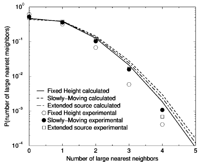
FIG. 4. Probability distributions for the number of large nearest neighbors for three different pouring techniques: fixed-height point source (FHPS), slowly-moving point source (SMPS), and extended source (ES). Points are experimental data and the curves are calculated as described in the text.
