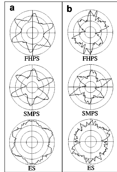
FIG. 2. (a) Comparison of mean-nearest-neighbor-angle distributions, \rho(\theta) , of all particles for three different pouring techniques: fixed-height point source (FHPS), slowly-moving point source (SMPS), and extended source (ES). The distributions are only for the left side of the sample typified by Fig. 1(b). The \rho(\theta) are given in radial plots and scaled in each plot such that the maximum value is 1 (the outmost circle). (b) Comparison of mean-nearest-neighbor-angle distributions for the particles on the force chains for three different pouring techniques. The distributions are for the left side of the sample too.
