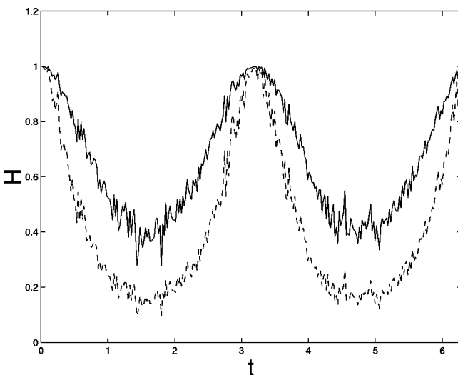
FIG. 2. Running one-word Rényi entropy I_{1;q}(t) [Eq. (14)] of the stochastic process [Eq. (15)] with different q values for an ensemble of N=500 simulated realizations with a SNR Q=1 , \omega=1 . Solid line: q=1 (Shannon entropy). Dashed line: q=4 .
