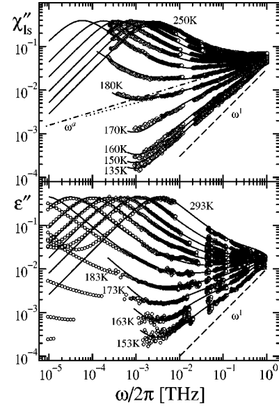
FIG. 1. Susceptibility spectra for propylene carbonate (PC, T_m \approx 218 K, T_g = 160 K) as measured by depolarized-light-scattering (upper panel, data from Ref. [1]), and dielectric-loss spectroscopy (lower panel, data from Ref. [6]), normalized with a temperature-independent static susceptibility. Temperatures are in steps of 10 K, unless indicated otherwise; in the dielectric measurement, T=243, 263, 273, 283 K are missing, for the light-scattering experiment, the highest temperature is 250 K (see text for details). The full lines are fits by solutions of the two-component schematic MCT model defined in Sec. II with parameters as described in the text. The dashed lines indicate a white-noise spectrum, \chi''_{\text{wh.n.}}(\omega) \propto \omega ; the dash-dotted line in the upper panel exhibits the asymptote of the critical spectrum \chi''(\omega) \propto \omega^a according to Eq. (15), with a = 0.30 corresponding to the value of \lambda = 0.75 . The dotted line shows the solution of the model for T = T_c and hopping terms neglected.
