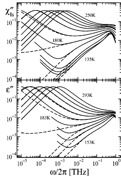
FIG. 7. The solid lines reproduce the susceptibility spectra \chi''_A(\omega) from Fig. 1 used for the fit to the light-scattering (upper panel) and the dielectric-loss spectra (lower panel), respectively. Dashed lines are solutions using the same model parameters, but with hopping effects ignored: \Delta = \Delta_{de}^s = 0 . Notice that the dashed lines for temperatures T below T_c exhibit a “knee” which is located between 10 and 100 GHz and moves to higher frequencies with decreasing T .
