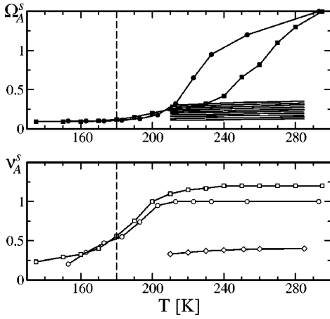
FIG. 5. Oscillator frequencies \Omega_A^s and damping constants \nu_A^s in THz specifying the transient motion for the second correlator as functions of temperature as used for the fits shown in Figs. 1 and 2. The squares refer to the light-scattering spectra, circles to the dielectric loss spectra; lines through the symbols are guides to the eye. For the neutron-scattering spectra, \nu_{ns}^s was taken q independent (diamonds in the lower panel), and the \Omega_{ns}^s exhibit the q \cdot \sqrt{T} -behavior shown in the upper panel (lines without symbols, q range as in Fig. 4). The vertical dashed lines indicate the critical temperature T_c .
