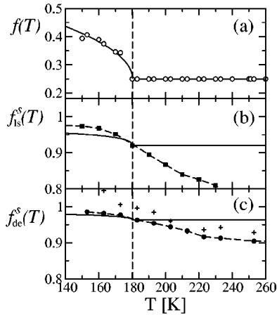
FIG. 10. Effective nonergodicity parameters determined from the calculated \phi_x -versus- \log t curves for the spectra shown in Fig. 1: f(T) for the first correlator \phi(t) (open circles), and f_A^s(T) for the correlators \phi_{ls}^s(t) and \phi_{de}^s(t) (filled squares and circles, respectively). The solid lines exhibit the leading-order-asymptotic laws for f_x from Eq. (17) for T \leq T_c and f_x^c for T \geq T_c . The vertical dashed line indicates the crossover temperature T_c = 180 K. The crosses in the lowest panel are estimations of f_{de}^s obtained in Ref. [6] by fitting the measured \varepsilon'(\omega) data with a Cole-Davidson function. The dashed lines through the solid symbols connect the values calculated from Eq. (18b) (see text for details).
