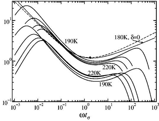
FIG. 13. Scaling-law analysis of the MCT solutions shown in Fig. 1 for the fit of the light-scattering spectra. The lower set of curves shows the rescaled spectra \chi''_{ls}(\omega)/h_{ls}\sqrt{|\sigma|} for T=220, 210, 200, 190 K (from top to bottom). The upper set of curves shows the same spectra, but now rescaled with h_{ls} replaced by the effective amplitude h_{ls}^{eff} from Eq. (18b). Notice that the order of the rescaled spectra is now inverted. The asymptotic result \hat{\chi} is plotted as a dashed line with the minimum position marked by a diamond. The result for T=180 K with hopping effects ignored is added to demonstrate the approach towards the scaling limit.
