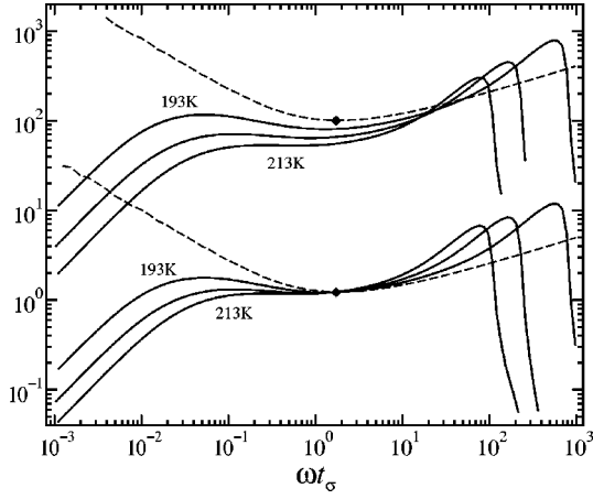
FIG. 14. Scaling-law analysis of the spectra for the memory kernel from the MCT solutions shown in Fig. 1 to interpret the dielectric function. The upper set of solid curves shows the unnormalized rescaled spectra, -\omega m_{\text{de}}''(\omega)/\sqrt{|\sigma|} , for temperatures T = 193, 203, 213 K. In the lower part of the figure, the scaling is shown for the normalized rescaled spectra -\omega \hat{m}_{\text{de}}''(\omega)/\sqrt{|\sigma|} (see text for details). The dashed lines are the master spectra, with the minimum positions marked by diamonds.
