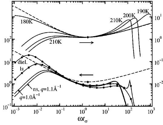
FIG. 11. The upper part of the figure (scale on right axis) shows the rescaled susceptibility spectra for four temperatures for the first correlator of the schematic model, \omega \phi''(\omega)/h\sqrt{|\sigma|} , as a function of \hat{\omega} = \omega t_\sigma . Hopping terms have been set to zero. The lower part (scale on the left axis) shows the \omega \phi_A^{s''}(\omega)/h_A \sqrt{|\sigma|} -versus- \hat{\omega} curves for T=210 K for the light-scattering (line with squares) and neutron-scattering correlators at q=1.0 and q=1.1 \text{ \AA}^{-1} (lines), and for T=213 K for the dielectric correlators (line with circles). The dashed lines indicate the master spectrum for \lambda=0.75 with the minimum position (\hat{\omega}_{\min}, \hat{\chi}_{\min}) marked by a diamond.
