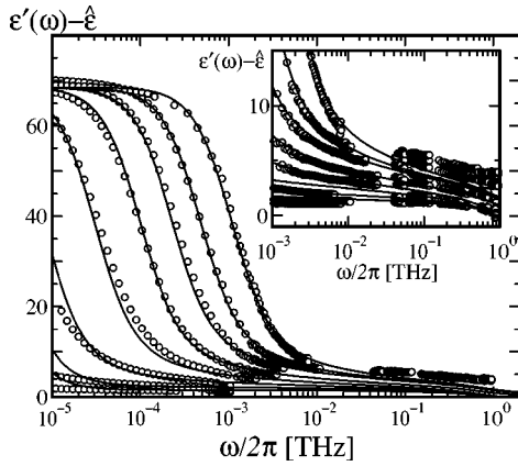
FIG. 8. Measured values for the real part \varepsilon'(\omega) of the dielectric function from Ref. [6] for T=173 K through T=233 K in steps of 10 K, and for T=253 K (from left to right). Experimental data have been shifted by \hat{\varepsilon} to account for an unknown background; see text for details. Temperatures T=163 K and below, and T=293 K are not shown in order to avoid overcrowding of the figure. For the same reason, the data points for frequencies above 1 GHz have been partially removed for all but the highest temperature and are only shown in the inset. The full lines are the real parts of the calculated susceptibilities for the same model parameters as used for the curves in Fig. 1.
