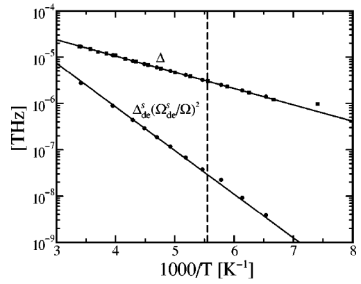
FIG. 6. In the upper part, the hopping coefficient \Delta entering Eq. (3a) for the first correlator used for the fits shown in Fig. 1 to the dielectric (circles) and light-scattering (squares) data is exhibited. The values follow an Arrhenius-type temperature dependence, indicated by a straight line. For the fit to the neutron-scattering data, the same values could be used, but show no influence on the fit curves in Fig. 2 (see text for details). For the fit to the dielectric data, an additional hopping coefficient \Delta_{de}^s for the second correlator had to be used, shown by the circles in the lower part of this figure; here, the values (\Omega_{de}^s/\Omega)^2 \Delta_{de}^s follow an Arrhenius law indicated by a straight line. The vertical dashed line indicates 1000/T_c with T_c = 180 K.
