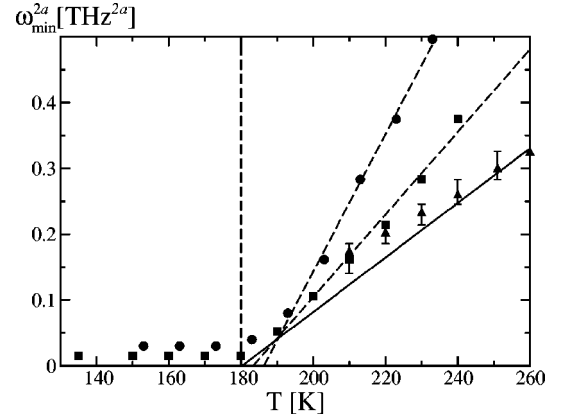
FIG. 12. Rectification diagram for the minimum positions \omega_{\min} of the dielectric-loss (circles), light-scattering (squares), and neutron-scattering (triangles) fit. The neutron-scattering data have been averaged over the investigated q range, and error bars indicate the smallest and highest values. The vertical dashed line marks the critical point T_c . The solid line is the asymptotic-formula result for the minimum positions calculated from the \beta -relaxation-scaling law for the fit parameters of the model used in Figs. 1 and 2. The dashed lines show the linear interpolation through the data points, restricted to the regime 190 \text{ K} \leq T \leq 250 \text{ K} , for the dielectric-loss and for the light-scattering data, respectively.
