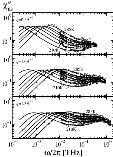
FIG. 2. Susceptibility spectra for PC as measured by incoherent neutron scattering for three wave vectors q , from Ref. [10]. Temperatures are T=210, 220, 230, 240, 251, 260, 285 K, where alternating open and filled symbols have been used to help distinguishing different data sets. For lower temperatures, data points below 10 GHz are seriously affected by the spectrometer's resolution function and therefore not shown. Full lines are fits as in Fig. 1.
