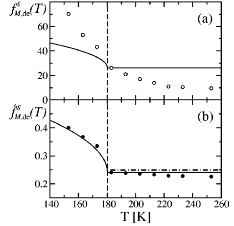
FIG. 15. (a) Unnormalized nonergodicity parameters f_{M,\text{de}}^s for the memory kernel from the fit to the dielectric spectra (open circles). The asymptotic prediction is plotted as a solid line, the vertical dashed line indicates T_c . (b) Same as in (a), but normalized values \hat{f}_{M,\text{de}}^s (filled circles). The dash-dotted line indicates the critical plateau value for the first correlator of the schematic model, f^c .
