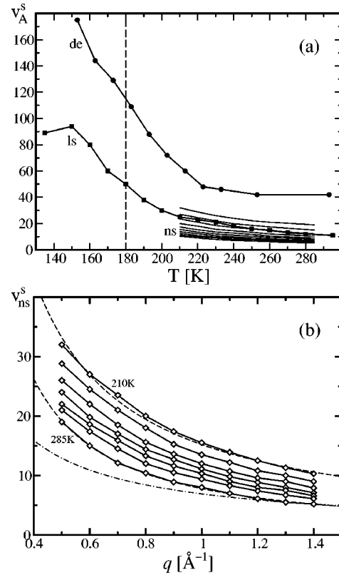
FIG. 4. (a) Coupling coefficients v_A^s for the second mode-coupling functional, Eq. (5b), used for the fits shown in Figs. 1 and 2 as functions of temperature. The squares refer to the light-scattering data and the circles to the dielectric-loss spectra; the lines through the symbols are guides to the eye. The lines without symbols connect the v_{ns}^s(q) used for the neutron-scattering data for 10 wave vectors q=0.5, 0.6, \dots, 1.4 \text{ \AA}^{-1} (from top to bottom). The vertical dashed line indicates the critical temperature T_c . (b) Coefficients v_{ns}^s(q, T) for the neutron-scattering data as functions of q for various fixed T . From top to bottom, the temperatures increase from T=210 to 285 K (as given in Fig. 2). The dashed lines indicate A/q + B/q^2 laws to visualize the difference to a 1/q -law behavior, which is shown as a dot-dashed line; see text for details.
