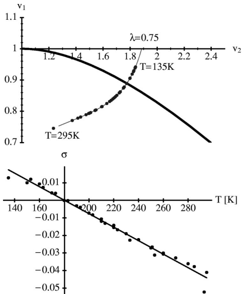
FIG. 3. Vertices v_1, v_2 for the first mode-coupling functional, Eq. (3b), used for the fits shown in Figs. 1 and 2. In the above diagram, the thick line represents the curve of glass-transition singularities, Eq. (4), while the thin line serves as a guide to the eye indicating the chosen path. Each dot corresponds to one temperature. The lower diagram shows the separation parameter \sigma , Eq. (8), as a function of T ; the critical temperature T_c \approx 180 K is determined from the zero of the shown regression line.
