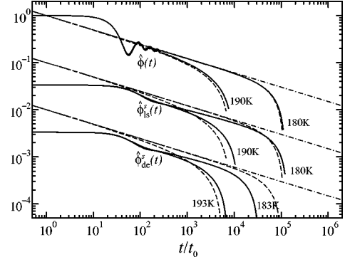
FIG. 9. The full lines show \hat{\phi}_x(t) = (\phi_x(t) - f_x^c)/h_x for times where \hat{\phi}_x(t) > 0 . The dash-dotted straight lines exhibit (t/t_0)^{-a} , with t_0 = 0.035 ps and a = 0.30 . The dashed lines show the \beta -correlators G(t) for the indicated temperatures (see text). The uppermost set of curves refers to the first correlator of the schematic model. The other two sets refer to the light-scattering and the dielectric response studied in Fig. 1. The sets are shifted vertically by one (light scattering), respectively two (dielectric response) decades for clarity.
