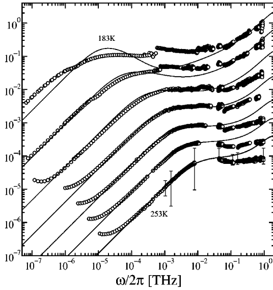
FIG. 16. The lines show the dielectric-modulus spectra defined by the right-hand side of Eq. (23b). The circles exhibit \text{Im}[(\hat{\epsilon} - \epsilon(\omega))^{-1}] calculated from the dielectric-function data of Ref. [6]. The curves and the data sets have been shifted vertically to avoid overlapping; temperatures and shift factors are (183 K, 1), (193 K, 0.316), (203 K, 0.1), (213 K, 0.0316), (223 K, 0.01), (233 K, 0.00316), (253 K, 0.001). For the highest temperature, an estimation of the uncertainty introduced by inverting the experimental data is given as error bars; see text for details.
