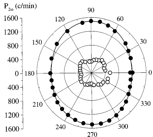
FIG. 7. Dependencies of the s - p second-harmonic power on the sample rotation angle \Phi for two subsequent linearly polarized UV irradiations with orthogonal polarization directions: first irradiation—40 min with \vec{E}_{UV} parallel to s polarization (solid circles), second irradiation—90 min with \vec{E}_{UV} parallel to the p -polarization plane (open circles). Solid line is fit to Eq. (7).
