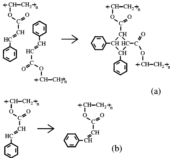
FIG. 1. Photochemical reactions in PVCN: (2+2) cycloaddition (a) and trans-cis isomerization (b) [6].
