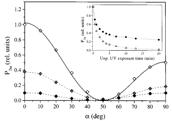
FIG. 2. Output power P_{2\omega} of the p -polarized second-harmonic radiation as a function of the polarization direction of the fundamental beam: before UV irradiation (open diamonds), after two minutes of unpolarized UV irradiation (crossed diamonds), and after five minutes of unpolarized UV irradiation (solid diamonds). \alpha=0^\circ corresponds to s input polarization. The solid line is a fit to Eq. (4). The dashed lines are guides to the eye. Inset: relative decrease of the second-harmonic power for s - p ( \alpha=0^\circ ) (triangles) and p - p ( \alpha=90^\circ ) (circles) polarization combinations as a function of the unpolarized UV irradiation time. The dashed lines are guides to the eye.
