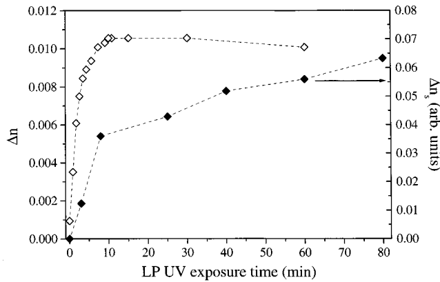
FIG. 9. Measured net birefringence of the sample (open diamonds) and calculated surface birefringence of the trans -cinnamoyl groups accordingly to the SSHG data (solid diamonds) as functions of the linearly polarized UV exposure time. The dashed lines are guides to the eye.
