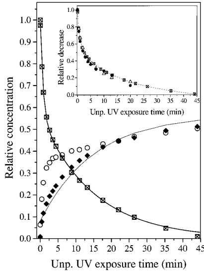
FIG. 3. Relative concentrations of various forms of the cinnamoyl side groups as a function of exposure time to unpolarized UV light: trans isomer (squares), cis isomer (circles), and dimerized groups (diamonds). The thick solid line is fit to a two exponential decay function. The thin solid line is fit to the dependence c_d(t) = a + b[1 - \exp(-t/\tau_2)] by using the fixed value of \tau_2 = 15 min. Inset: Relative decrease of the effective nonlinear susceptibilities corresponding to the s-p (triangles) and the p-p (circles) SSHG signal, and relative concentration of the trans -cinnamoyl groups (squares) during unpolarized UV irradiation. The dashed line is for guidance.
