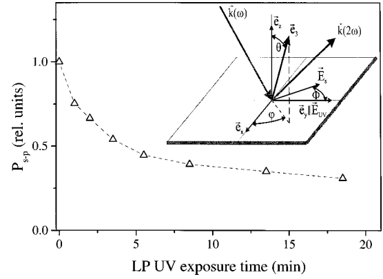
FIG. 4. Relative decrease of P_{2\omega} for the s-p polarization combination during exposure to linearly polarized UV light. The inset shows the orientation of various coordinate axes of the sample: absorption axis \vec{e}_3 , surface normal \vec{e}_z , photopolymerization axis \vec{e}_y (which is parallel to the direction of the UV polarization \vec{E}_{UV} ), and the direction of the s -polarized optical field \vec{E}_s . The measurement was performed at \vec{E}_s \parallel \vec{E}_{UV} , i.e., at \Phi = 0^\circ .
