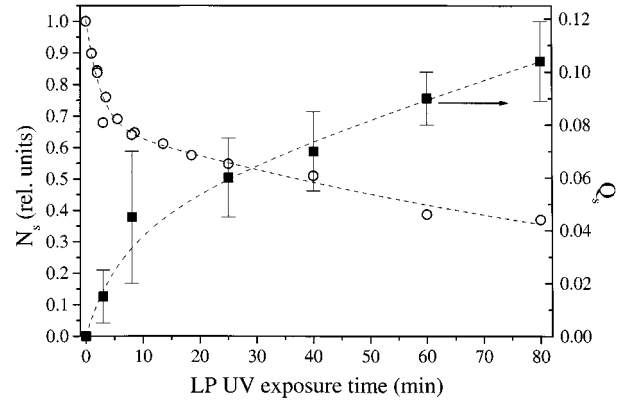
FIG. 8. Relative surface density (circles) and surface orientational order parameter (squares) of the trans -cinnamoyl side groups as functions of the linearly polarized UV exposure time. The dashed lines are guides to the eye.
