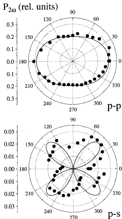
FIG. 6. Dependencies of the p - p and p - s second-harmonic power on the sample rotation angle \Phi measured after 40 min of exposure to linearly polarized UV light. The values are given relatively with respect to the P_{p-p}(\Phi) before the UV exposure. Solid lines are fits to Eq. (7).
