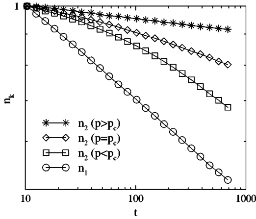
FIG. 15. Crossover effects near the multicritical point. The figure shows the particle densities n_k vs time in a two-level system starting from a fully occupied lattice, normalized at t=10 . Level A ( k=1 ) is always critical, while level B ( k=2 ) is either evolving in the active, critical, or inactive regime. Initially the decay of B particles is the same in all cases. Later the system crosses over to a different behavior where the B particles become independent or slaved to the A particles, respectively. (Time is measured in Monte Carlo steps.)
