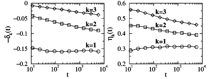
FIG. 13. Local slopes of the lines in Figs. 12(b) and 12(c). The slow drift of the slopes at higher levels indicates that the scaling regime is not yet reached in the present simulations. (Time is measured in Monte Carlo steps.)
