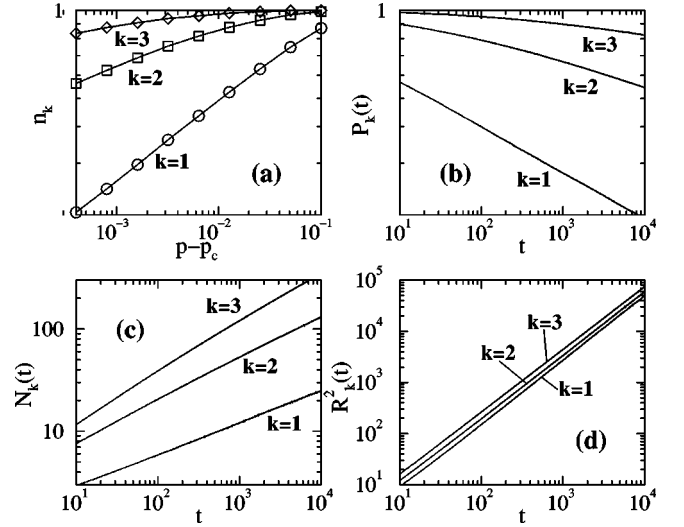
FIG. 12. Monte Carlo simulations of coupled DP in 1+1 dimensions. (a) Steady-state simulations in the active phase. (b)–(d) Dynamical simulations at criticality. Time is measured in Monte Carlo steps.
