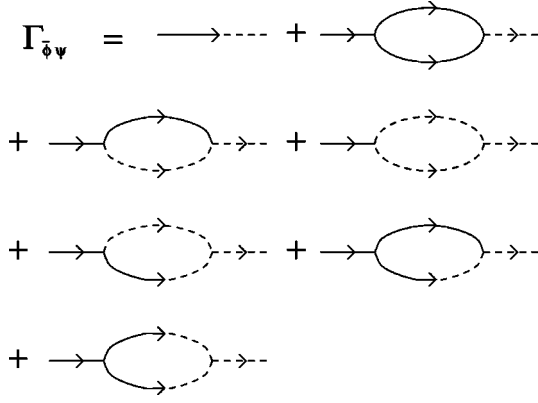
FIG. 4. “Mixed” two-point vertex function \Gamma_{\varphi\psi}^{-} to one-loop order for the coupled DP field theory.
