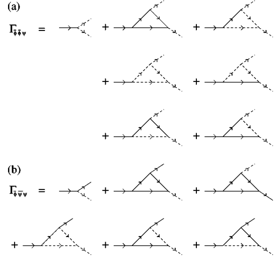
FIG. 5. The “mixed” three-point vertex functions (a) \Gamma_{\varphi\varphi\psi}^{-} and (b) \Gamma_{\varphi\psi\psi}^{-} to one-loop order.
