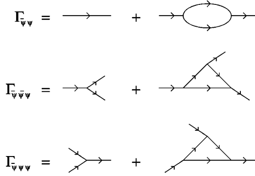
FIG. 2. Diagrams for the two- and three-point vertex functions to one-loop order for the pure DP field theory.
