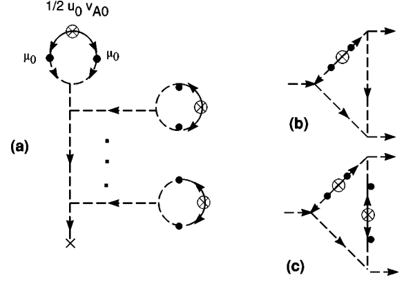
FIG. 10. (a) An IR-divergent diagram at higher loop order, contributing to the expectation value of \varphi . (b) IR-divergent diagram contributing to the three-point vertex function with one insertion of \bar{\psi}^2 . (c) IR-divergent diagram contributing to the three-point vertex function with two insertions of \bar{\psi}^2 .
