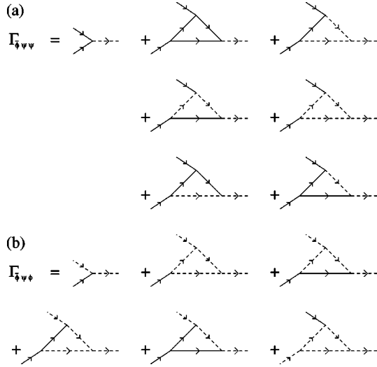
FIG. 6. The “mixed” three-point vertex functions (a) \Gamma_{\bar{\psi}\psi\psi} and (b) \Gamma_{\bar{\psi}\psi\phi} to one-loop order.
