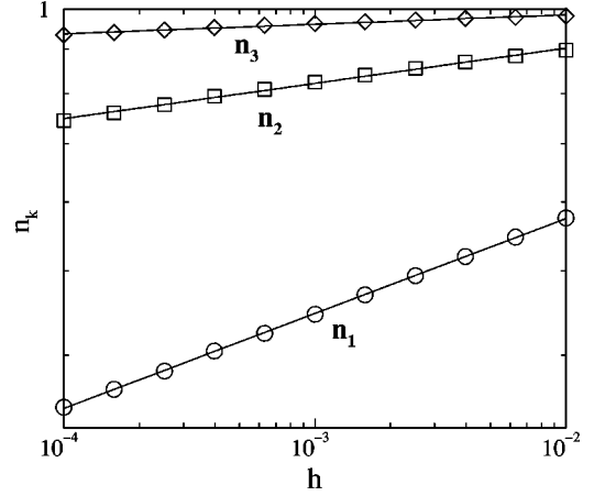
FIG. 14. Susceptibility of multicritical coupled DP to an external field. The figure shows the stationary particle densities n_k versus the rate h for spontaneous particle creation.
