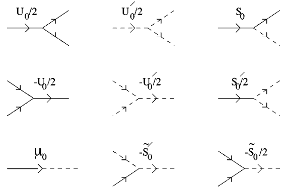
FIG. 3. The vertices of the full action S_{MC} .
