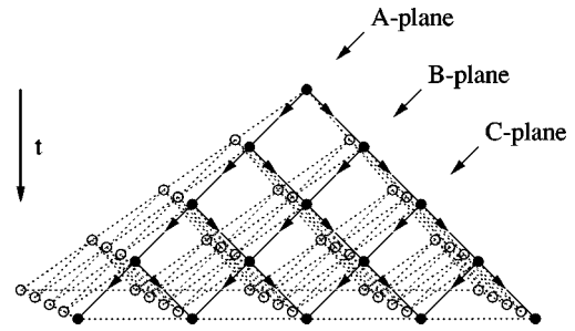
FIG. 17. Realization of a unidirectionally coupled hierarchy of (1+1) -dimensional DP processes in a (2+1) -dimensional directed bond percolation process with parallel updates. The figure shows the “light cone” starting from a single site. The subsystems A, B, C, ... correspond to tilted planes as indicated by the arrows.
