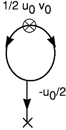
FIG. 7. One-loop diagram for \langle \psi_{c0} \rangle in the pure DP active phase calculation.
