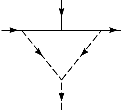
FIG. 18. Coupled annihilation: An IR-divergent diagram contributing to the aa\bar{b} vertex at one-loop order.
