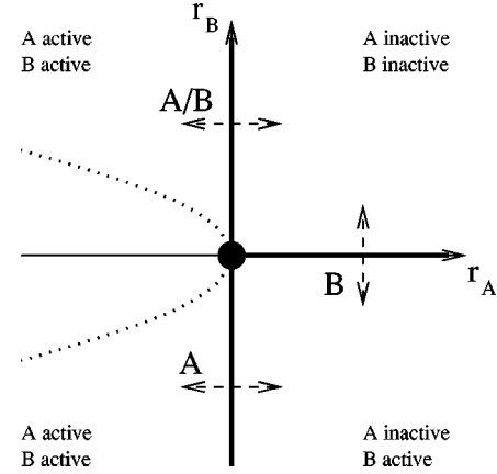
FIG. 1. Mean-field phase diagram for the two-level coupled DP process. The arrows mark DP active/absorbing transitions for the A and B particle species, respectively. The dotted parabola denotes the boundary of the multicritical regime, which includes |r_A| = |r_B| = |r| \rightarrow 0 .
