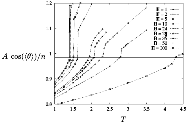
FIG. 10. Product of the cosine of the average tilt angle with the area per molecule, A \cos(\langle\theta\rangle)/n , in units of \sigma^2 , vs temperature T in units of \epsilon/k_B for different pressures \Pi (in units of \epsilon/\sigma^2 ) as indicated. The horizontal line indicates the position of a_c = 0.985\sigma^2 .
