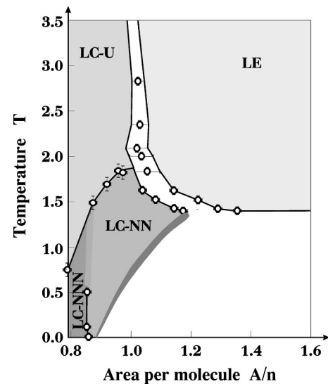
FIG. 15. Phase diagram in the area-temperature plane. Area per molecule A/n is given in units of \sigma^2 and temperature T is given in units of \epsilon/k_B . LE denotes disordered phase, LC-NN denotes ordered phase with tilt towards nearest neighbors, LC-NNN denotes ordered phase with tilt towards next nearest neighbors, and LC-U denotes untilted ordered phase. See text for more explanation.
