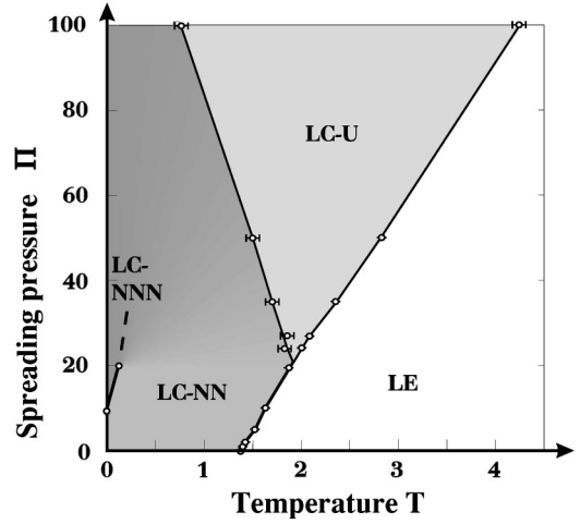
FIG. 14. Phase diagram in the pressure-temperature plane. Pressure \Pi is given in units of \epsilon/\sigma^2 and temperature T is given in units of \epsilon/k_B . LE denotes disordered phase, LC-NN denotes ordered phase with tilt towards nearest neighbors, LC-NNN denotes ordered phase with tilt towards next nearest neighbors, and LC-U denotes untilted ordered phase. The transition between LC-NN and LC-NNN could not be located at pressures above \Pi = 20\epsilon/\sigma^2 . See text for more explanation.
