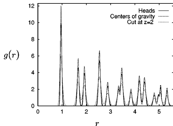
FIG. 3. Radial pair correlation functions g(r) vs r in units of \sigma at pressure \Pi = 100\epsilon/\sigma^2 and temperature T = 1\epsilon/k_B . Correlation functions are shown for the heads (solid line), for the points where the molecules cross the plane at z = 2\sigma above the surface (dotted line), and for the projection of the center of gravity onto the xy plane (dashed line). The values of g(r) for T = 0.1\epsilon/k_B are divided by a factor of 5 for clarity of presentation.
