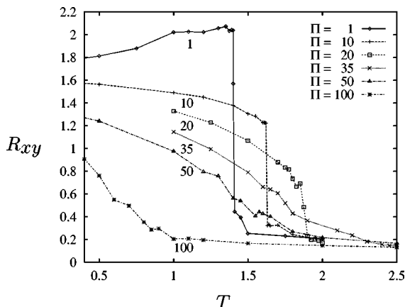
FIG. 8. Order parameter R_{xy} in units of \sigma^2 vs temperature T in units of \epsilon/k_B for different pressures \Pi (in units of \epsilon/\sigma^2 ) as indicated.
