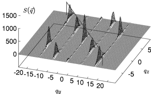
FIG. 6. Structure factor S(\vec{q}) in the yz plane ( q_x=0 ) for an ordered state with tilt towards next nearest neighbors. Parameters are \Pi=50\epsilon/\sigma^2 and T=0.1\epsilon/k_B .
