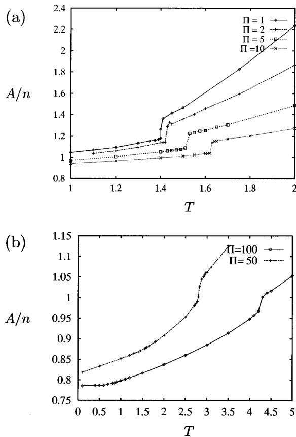
FIG. 2. Area per molecule A/n in units of \sigma^2 vs temperature T in units of \epsilon/k_B for a choice of low (a) and high (b) pressures \Pi (in units of \epsilon/\sigma^2 ) as indicated.
