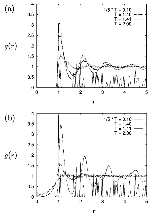
FIG. 4. Radial pair correlation functions g(r) vs r in units of \sigma at pressure \Pi = 1\epsilon/\sigma^2 and various temperatures as indicated. Correlation functions are shown for the heads (a) and for projections into the xy plane of the centers of gravity (b). Temperatures T are given in units of \epsilon . The correlation functions g(r) for the temperature T = 0.1\epsilon have been divided by a factor of 5.
