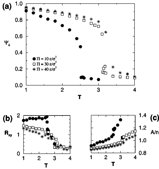
FIG. 13. Order parameters \Psi_6 and R_{xy} and area per molecule A/n vs temperature T in units of \epsilon/k_B for pressures \Pi = 10\epsilon/\sigma^2 (filled circles), 30\epsilon/\sigma^2 (open squares), 40\epsilon/\sigma^2 (stars) in systems of stiff chains ( k_A = 100\epsilon ).
