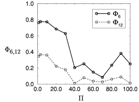
FIG. 12. Order parameters \Phi_6 and \Phi_{12} vs pressure \Pi in units of \epsilon/\sigma^2 at temperature T = 0.5\epsilon/k_B .
