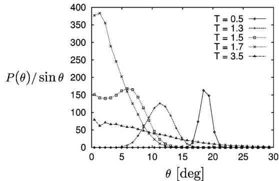
FIG. 11. Histogram P(\theta)/\sin\theta of the tilt angle \theta (in degrees) at pressure \Pi = 50\epsilon/\sigma^2 for different temperatures (in units of \epsilon/k_B ).
