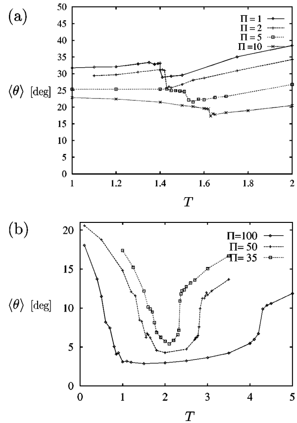
FIG. 9. Average tilt angle \langle\theta\rangle in degrees vs temperature T in units of \epsilon/k_B for different pressures \Pi (in units of \epsilon/\sigma^2 ) as indicated.
