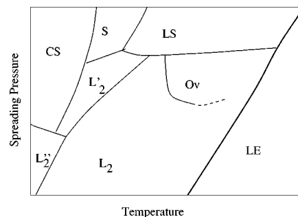
FIG. 1. Generic phase diagram for fatty acid monolayers. The phases LS , S , and CS are on average untilted, whereas Ov and L'_2 show tilt towards next nearest neighbors and L_2 and L''_2 show tilt towards nearest neighbors. In CS , S , L'_2 , and L''_2 , the backbones of the hydrocarbon chains are ordered. In CS and L''_2 , the molecules have crystalline order in addition.
