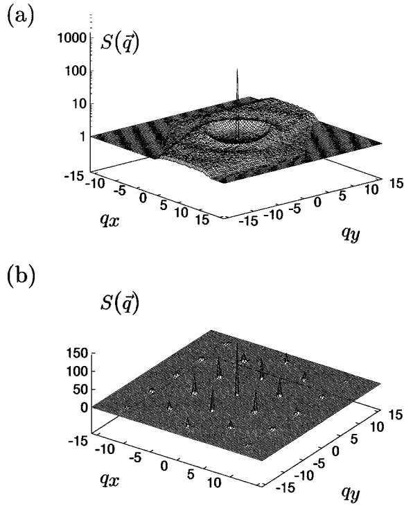
FIG. 5. Structure factor S(\vec{q}) in the xy plane ( q_z=0 ) for a disordered state (a) and an untilted ordered state (b). Parameters are \Pi=10\epsilon/\sigma^2, T=2.5\epsilon/k_B in (a) and \Pi=50\epsilon/\sigma^2, T=2.0\epsilon/k_B in (b).
