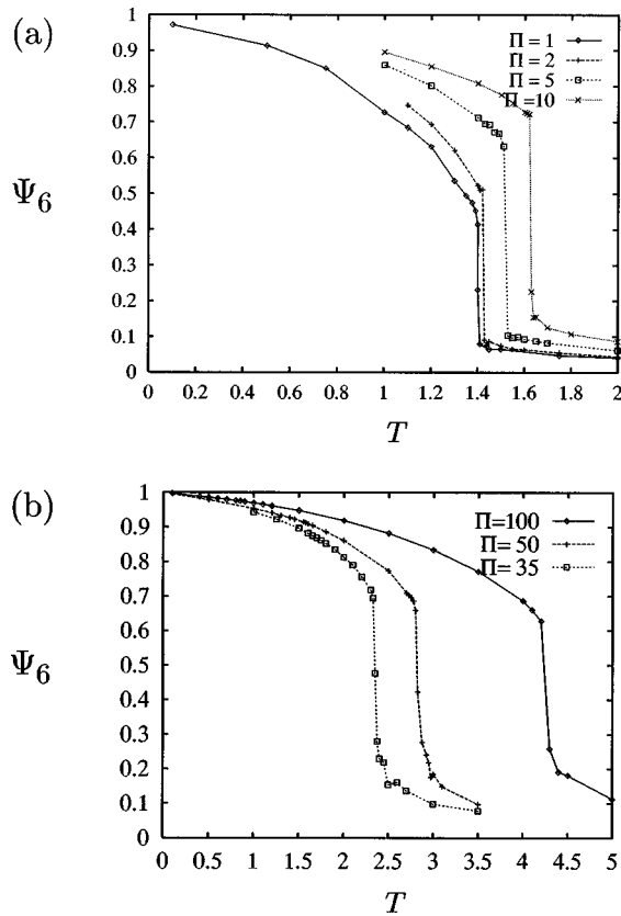
FIG. 7. Order parameter \Psi_6 vs temperature T in units of \epsilon/k_B for different pressures \Pi (in units of \epsilon/\sigma^2 ) as indicated.
