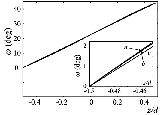
FIG. 3. \omega(z) profiles in a twisted and strongly anchored nematic slab with a delocalized variation of \phi . S_0=0.4 , while all other parameters are the same as in Fig. 1. In the inset \omega(z) in the subsurface region is shown. The deviation \delta\omega from the linear solution (11) spreads through the whole sample. Profiles for S_0=0.35 differ only negligibly from those plotted here.
