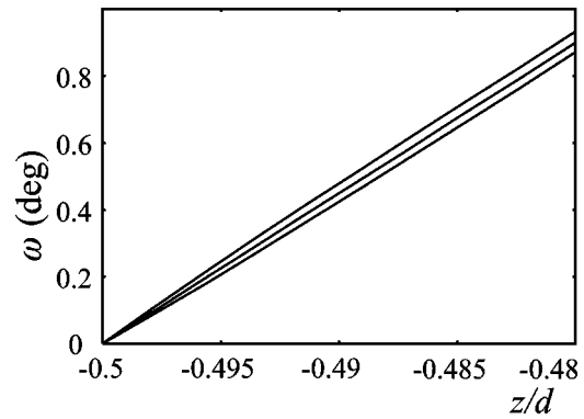
FIG. 4. \omega(z) profiles in the subsurface region of a twisted nematic slab with a localized variation of S ; \phi(\pm d/2) = 90^\circ , S_b \approx 0.375 , \Delta S \approx 0.025 , 0, and -0.025 (the top, middle, and bottom curves, respectively), \omega(-d/2) = 0^\circ , \omega(d/2) = 45^\circ , and L_2 = 0 [for \phi(\pm d/2) = 90^\circ the problem is degenerate with respect to the value of L_2 ]. The profiles cross in the middle of the sample and exhibit a similar behavior at the opposite side, the top curve, e.g., now corresponding to the negative value of \Delta S . The values for a , B , C , T - T^* , and L_1 are the same as in Fig. 1.
