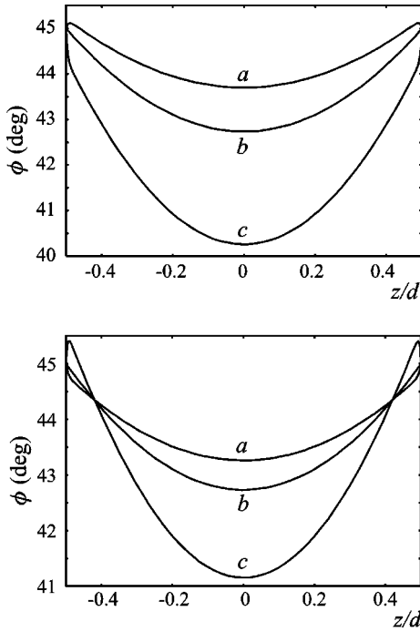
FIG. 2. \phi(z) profiles in a twisted nematic slab with strong anchoring. The same parameters as in Fig. 1 have been used. S_0=0.35 (top figure) and S_0=0.4 (bottom figure).
