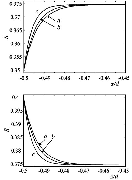
FIG. 1. S(z) profiles in a twisted nematic slab with strong anchoring. \phi(\pm d/2) = 45^\circ , \omega(-d/2) = 0^\circ , \omega(d/2) = 45^\circ , S_b \approx 0.375 , S_0 = 0.35 (top figure) or S_0 = 0.4 (bottom figure), and L_2 = L_1 , 0 , and -L_1 (curves a , b , and c , respectively). The sample thickness equals 1 \mu\text{m} , a = 0.13 \times 10^6 \text{ J/m}^3 \text{ K} , B = 1.6 \times 10^6 \text{ J/m}^3 , C = 3.9 \times 10^6 \text{ J/m}^3 , T - T^* = 0.4 \text{ K} , and L_1 = 10^{-11} \text{ N} .
