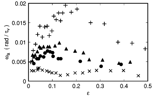
FIG. 12. The frequency \omega_a as a function of \epsilon for \Gamma=40 and \Omega=8.8 (crosses), 10.5 (circles), 11.0 (triangles), and 12.1 (pluses).
