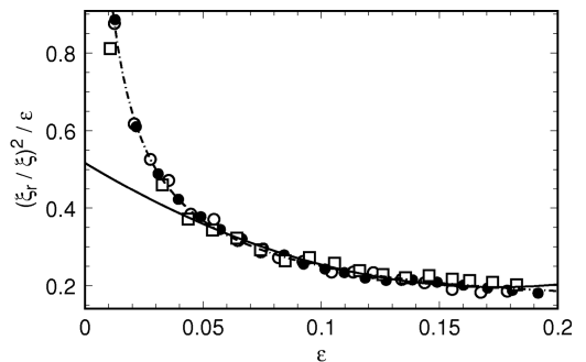
FIG. 19. The inverse square (1/\tilde{\xi})^2 of the reduced correlation length \tilde{\xi} = \xi / \xi_r , divided by \epsilon , as a function of \epsilon on linear scales. The data are for (\Omega, \xi_r) = (14.3, 1.00) (open circles), (16.5, 0.913) (solid circles), and (19.7, 0.839) (open squares). The dash-dotted line is a fit of the power law Eq. (8) to the data and corresponds to an exponent of 0.17. The solid line is a fit of Eq. (9) to the data.
