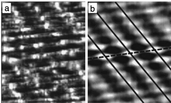
FIG. 2. An example of (a) F(\Theta, t) and (b) C(\delta\Theta, \delta t) for \Omega=15.4 and \epsilon=0.027 . For F(\Theta, t) the horizontal axis spans 0 < \Theta < \pi . The vertical axis for t covers an interval of 2080 \tau_v , with t increasing in the upward direction. For C(\delta\Theta, \delta t) the origin is in the center, with -\pi/2 < \delta\Theta < \pi/2 and -1040 < \delta t < 1040 \tau_v . Bright (dark) areas are high (low) values.
