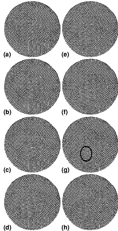
FIG. 7. Time sequence of images for \Gamma=40 with Küppers-Lortz domains and dislocation-defect motion at \epsilon=0.03 and \Omega=16.5 . The images are 6.7 \tau_v apart. The ellipse in (g) contains a pair of defects which formed by the pinching-off of a roll.
