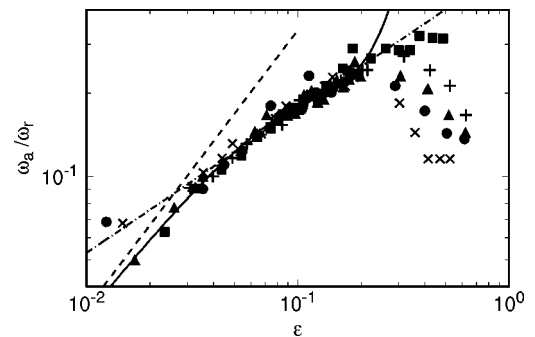
FIG. 16. The reduced frequency \tilde{\omega}_a = \omega_a/\omega_r as a function of \epsilon for \Gamma=40 on logarithmic scales. The data are for (\Omega, \omega_r) = (13.2, 0.152) (crosses), (14.3, 0.273) (circles), (15.3, 0.400) (triangles), (16.5, 0.541) (pluses), and (19.8, 1.000) (squares). The dashed line corresponds to an exponent of 1. The dash-dotted line is a fit of the power law Eq. (5) to the data and corresponds to an exponent of 0.52. The solid line is a fit of Eq. (6) to the data.
