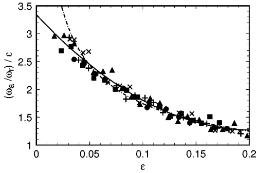
FIG. 17. The reduced frequency \tilde{\omega}_a = \omega_a / \omega_r divided by \epsilon as a function of \epsilon on linear scales. The data are for (\Omega, \omega_r) = (13.2, 0.152) (crosses), (14.3, 0.273) (circles), (15.3, 0.400) (triangles), (16.5, 0.541) (pluses), and (19.8, 1.000) (squares). The solid line is a fit of Eq. (6) to the data. The dash-dotted line is a fit of the power law Eq. (5) to the data and corresponds to an exponent of 0.52.
