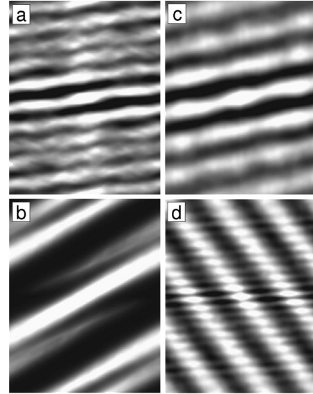
FIG. 9. Gray-scaled autocorrelations C(\delta\Theta, \delta t) for the angle-time plots in Fig. 8. (a) \Omega = 8.8 , \epsilon = 0.04 ; (b) \Omega = 8.8 , \epsilon = 0.16 ; (c) \Omega = 12.7 , \epsilon = 0.10 ; (d) \Omega = 16.5 , \epsilon = 0.03 . Bright (dark) areas correspond to large (small) values.
