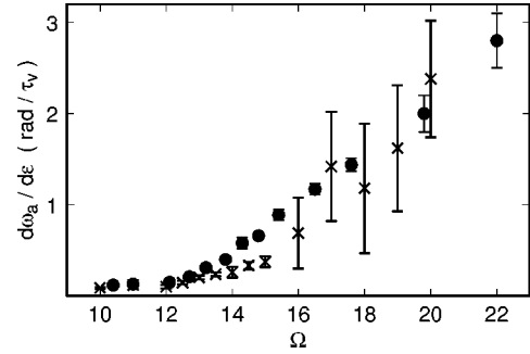
FIG. 15. The slope W = d\omega_a/d\epsilon for small \epsilon as a function of \Omega for \Gamma=40 , \sigma=0.93 (solid circles) and \Gamma=23 , \sigma=0.83 (crosses).
