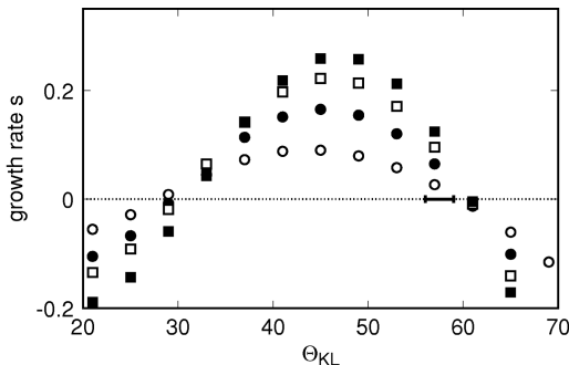
FIG. 11. Calculated growth rates s(\Theta_{\text{KL}}) as a function of \Theta_{\text{KL}} (units of degrees) for \Omega=15.4 and \epsilon=0.05 (open circles), 0.10 (solid circles), 0.15 (open squares), and 0.20 (solid squares). The small horizontal bar represents the experimental results for \Theta_s shown in Fig. 10.
