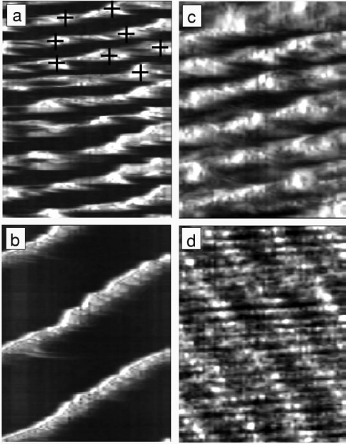
FIG. 8. Gray-scaled angle-time plots of F(\Theta, t) for \Gamma = 40 and (a) \Omega = 8.8 , \epsilon = 0.04 , 9600\tau_v ; (b) \Omega = 8.8 , \epsilon = 0.16 , 4800\tau_v ; (c) \Omega = 12.7 , \epsilon = 0.10 , 1133\tau_v ; and (d) \Omega = 16.5 , \epsilon = 0.03 , 1600\tau_v . Bright (dark) areas correspond to large (small) values.
