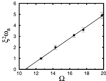
FIG. 21. The average diffusivity \langle \xi^2 \omega_a \rangle , averaged over the range 0.04 < \epsilon < 0.2 , as a function of \Omega .
