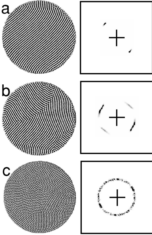
FIG. 1. Real-space images and their gray-scaled Fourier-transform moduli F(\mathbf{k}, t) for (a) \Omega=4.4 and \epsilon=0.05 , (b) \Omega=8.8 and \epsilon=0.05 , and (c) \Omega=17.6 and \epsilon=0.024 .
