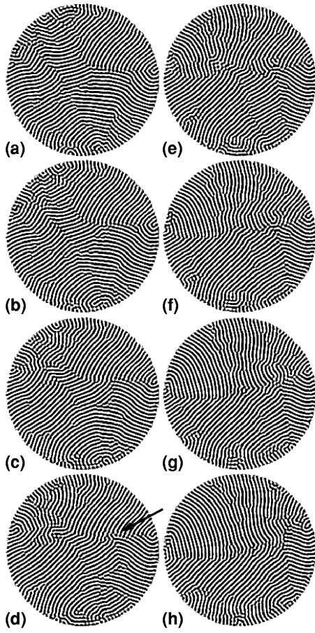
FIG. 6. Time sequence of images for \Gamma=40 with Küppers-Lortz domains and dislocation-defect motion at \epsilon=0.10 and \Omega=12.7 . The images are 8.9 \tau_v apart. The arrow in (d) points to a region away from the sidewall with a spontaneously nucleated domain.
