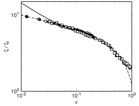
FIG. 18. The reduced correlation length \tilde{\xi} = \xi / \xi_r as a function of \epsilon on logarithmic scales. The data are for (\Omega, \xi_r) = (14.3, 1.00) (open circles), (16.5, 0.913) (solid circles), and (19.7, 0.839) (open squares). The dash-dotted line is a fit of the power law Eq. (8) to the data and corresponds to an exponent of 0.17. The solid line is a fit of Eq. (9) to the data.
