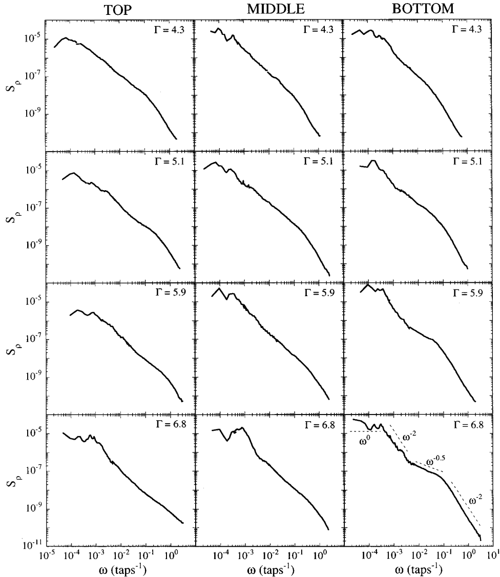
FIG. 5. The power spectral density S_\rho (taps) of the fluctuations as a function of frequency \omega in the steady state is shown for the three depths at various \Gamma . For most spectra, two characteristic corner frequencies, \omega_L and \omega_H , are discernible which shift to higher frequencies for increasing \Gamma and decreasing depth. The characteristic regimes of behavior are denoted by the dashed lines in the lower right hand panel, which are guides to the eye.
