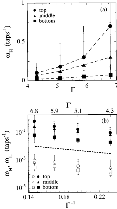
FIG. 6. The characteristic frequencies, \omega_L (open symbols) and \omega_H (solid symbols), in the power spectra plotted as a function of 1/\Gamma . The general trend is for both \omega_L and \omega_H to increase with increasing \Gamma and decreasing depth into the pile. The dashed line in (b) is a guide to the eye, indicating that the trend is consistent with an activated-like behavior \omega \propto \exp(-\Gamma_0/\Gamma) , with \Gamma_0 \approx 15 . For comparison, (a) shows the dependence of \omega_H on \Gamma .
