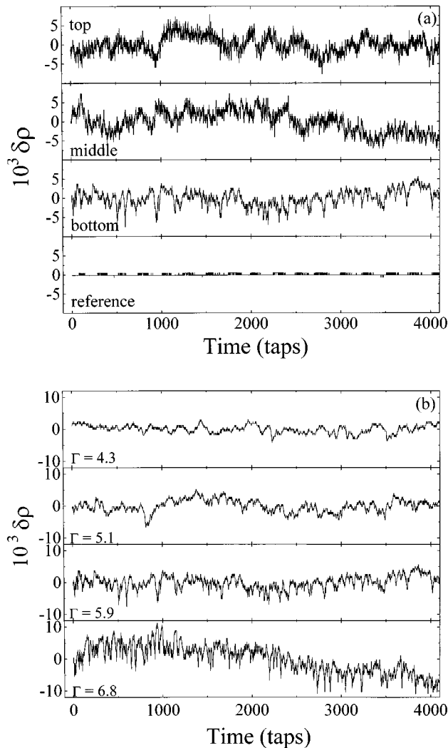
FIG. 3. Fluctuations in the volume density \delta\rho(t)=\rho(t)-\rho_{ss} after the system has had sufficient time to relax to a steady-state density \rho_{ss} . In (a) the fluctuations at three different depths are shown for \Gamma=5.9 . The reference capacitor is used to correct for any instrumental drift. The dependence of the fluctuations on \Gamma is shown in (b) for the beads near the bottom of the pile. Fluctuations over a broad range of time scales are evident.
