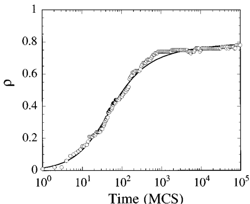
FIG. 8. The time evolution of the density in the simulation for k=10^3 ( \rho_{ss}=0.84 ). Time is in units of Monte Carlo steps (MCS). The solid line represents a fit to Eq. (1).
