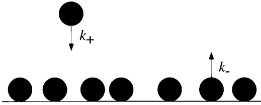
FIG. 7. The adsorption-desorption process. Adsorption is successful only in spaces large enough to accommodate a particle. Desorption of a particle, on the other hand, is unrestricted.
