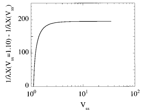
FIG. 12. The left hand side of Eq. (5) is numerically evaluated and plotted as a function of steady-state volume for the simulation data. As plotted, the difference in inverse compactivities between the highest density configuration ( V_{ss} = 1.1 ) and a low density configuration (higher V_{ss} ) can be read off directly.
