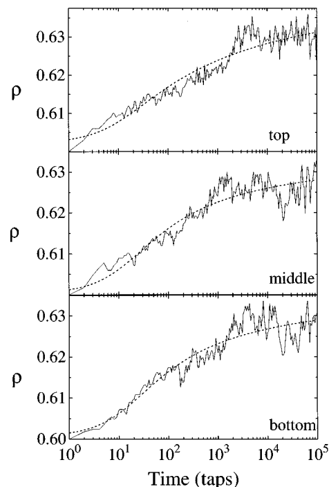
FIG. 1. The time evolution of the volume density \rho at three different depths near the top, middle, and bottom of the pile of beads. The curves represent a single run (no ensemble averaging) at a vibration intensity \Gamma = 6.8 . The pile settles slowly from its initial low density configuration towards a higher steady-state density at long times, t > 10^4 taps. The dashed lines are fits to Eq. (1) with typical values of parameters: 0.637 \leq \rho_\infty \leq 0.647 , 0.036 \leq \Delta\rho_\infty \leq 0.044 , 0.20 \leq B \leq 0.40 , 10 \leq \tau \leq 18 .
