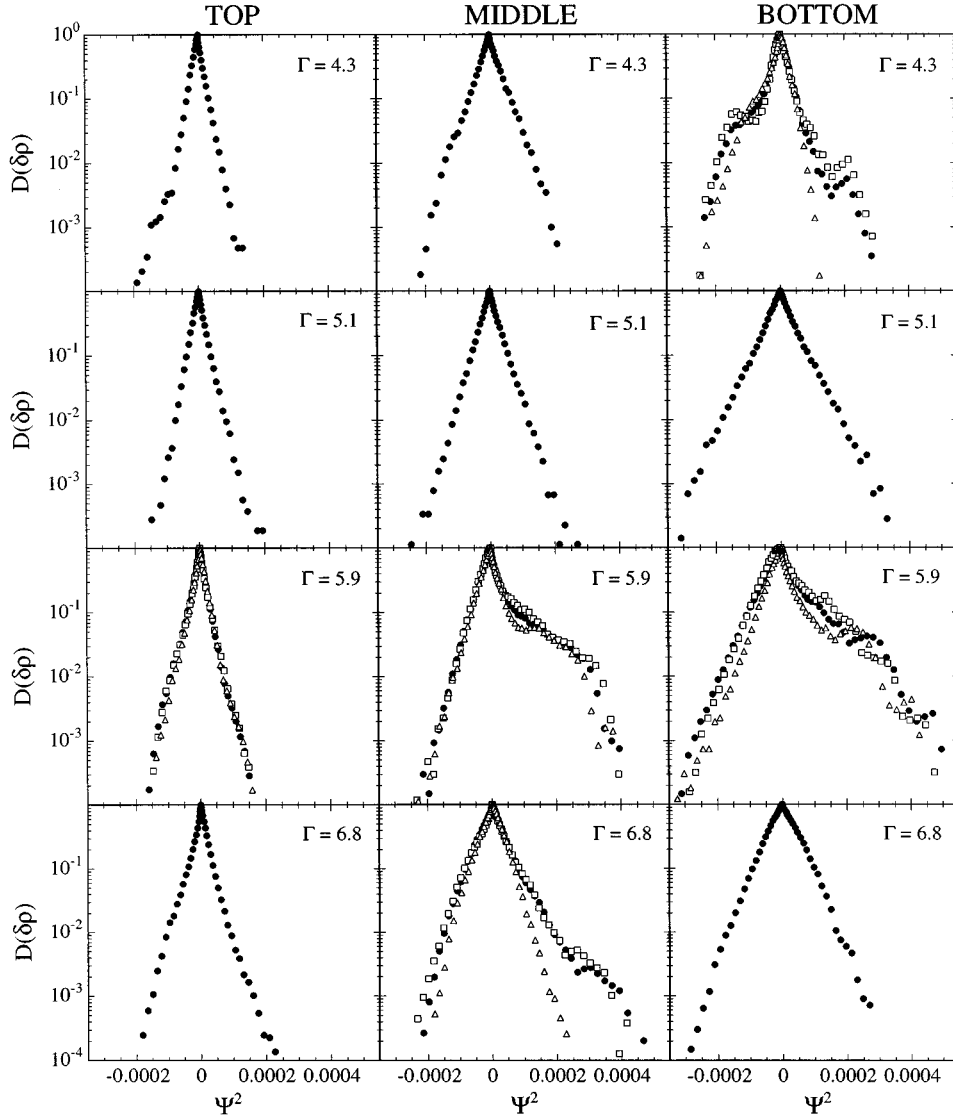
FIG. 4. The distribution functions D(\delta\rho) for the occurrence of fluctuation amplitudes in the steady state are shown (solid circles) for the three depths at various \Gamma . Plotted as a function of \Psi^2 = \delta\rho^2 \operatorname{sgn}(\delta\rho) a Gaussian distribution has a triangular shape. For selected panels, the time dependence of the distributions is shown by plotting the distribution functions for only the first (open squares) or second (open triangles) half of the time record. The majority of data appears stationary even when significant non-Gaussian deviations are observed, e.g., at \Gamma = 5.9 near the middle and bottom of the pile.
