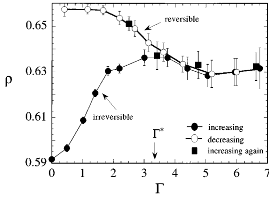
FIG. 2. The dependence of \rho on the vibration history. The beads were prepared in a low density initial configuration and then the acceleration amplitude \Gamma was slowly first increased (solid symbols) and then decreased (open symbols). At each value of \Gamma the system was tapped 10^5 times after which the density was recorded and \Gamma was subsequently incremented by \Delta\Gamma \approx 0.5 . The upper branch that has the higher density is reversible to changes in \Gamma , see square symbols. \Gamma^* denotes the irreversibility point (see text).
