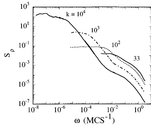
FIG. 9. Power spectra, S_\rho (MCS), of the density fluctuations in the simulation of the one-dimensional parking process. The evolution of the spectral dependence is shown for values of the ratio k=33, 10^2, 10^3, 10^4 , corresponding to final steady-state densities \rho_{ss}=0.72, 0.77, 0.84 , and 0.88 , respectively (see text). The strongest dependence on k is for \omega_L , which decreases rapidly as the density increases. Such spectra are similar to those found in the experiment, see Fig. 5.
