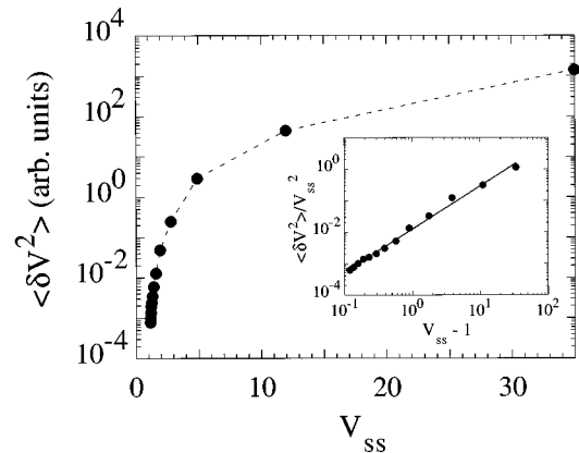
FIG. 11. The average variance of the volume fluctuations in the simulation as a function of the steady-state volume, V_{ss} . The fractional variance as a function of V_{ss} - 1 is plotted on logarithmic axes in the inset. The solid line is a power-law fit given by 0.0124(V_{ss} - 1)^{1.37} .
