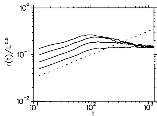
FIG. 12. Averaged wave-front roughness as a function of time in TLM lattices with p=0.85 and vertical heights L_y=30,60,120,240 ; the driving frequency is 0.314. The dashed line is given by r(t) \propto t^{1/2} .
