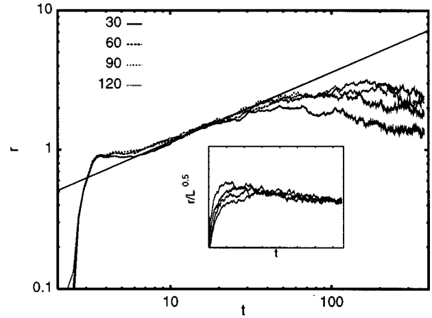
FIG. 11. Averaged wave-front roughness as a function of time in lattices with p=0.7 and vertical heights L_y=30,60,90,120 ; l=1 , m=1.0 , w=1.0 , E=1.0 , and the frequency is 0.125. The fitted line is given by r(t) \propto t^{1/2} . The inset shows the same data on a semilogarithmic scale, with the y axis rescaled by L^{-0.5} .
