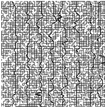
FIG. 8. Wave-front location (thick lines) at different times in lattices with (top) w=0.001 and p=0.98 , (middle) w=1.0 , and p=0.7 , and (bottom) w=20.0 and p=0.7 .
