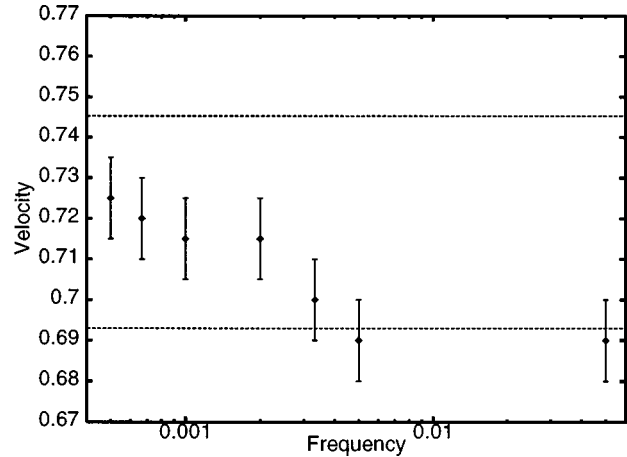
FIG. 3. Average velocity of a longitudinal wave front as a function of the driving frequency with l=1 , m=0.1 , w=0.3 , p=0.9 , and E=1.0 . The upper and the lower lines are the prediction by the effective-medium approximation and the model of one-dimensional paths, respectively.
