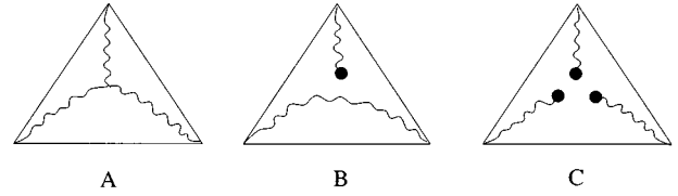
FIG. 2. Diagrams representing the generating functions for spanning trees on the Sierpinski gasket.
