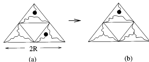
FIG. 3. Formation of a loop of perimeter of the order of R^z on addition of a bond.
