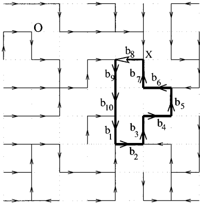
FIG. 1. A spanning tree T_N with the end point of walk at X . The loop \mathcal{L} (shown in bold) of ten directed bonds is formed if the bond b_8 , denoted by the white arrow, is added to T_N . In this case there is a directed path from the origin O to the head of b_8 .
