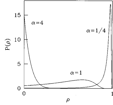
FIG. 1. Distribution of the phase rigidity \rho for \alpha=1/4, 1 , and 4 , computed from Eq. (9). The crossover from the orthogonal to unitary ensemble occurs when \alpha \approx 1 , and is associated with large fluctuations in \rho around its ensemble average.
