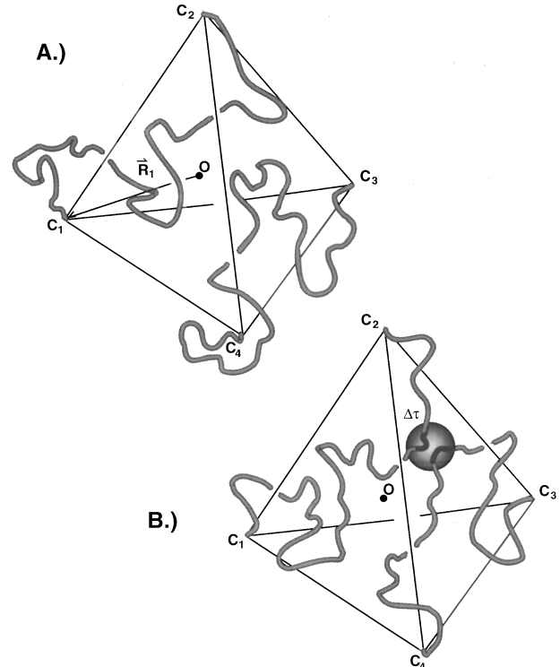
FIG. 21. Allowable configurations of polymer strands (a) before and (b) after bond formation. Each pair of bonded mers has four nearest cross-linked neighbors.
