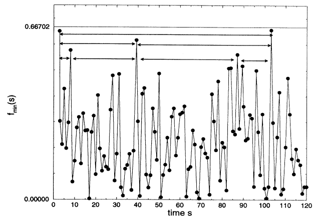
FIG. 5. Illustration of the hierarchical structure of the f_0 avalanches. The big avalanche is subdivided into smaller ones as the auxiliary parameter f_0 is lowered. The lines span f_0 avalanches for f_0 = 0.63, 0.59 , and 0.54 , respectively.
