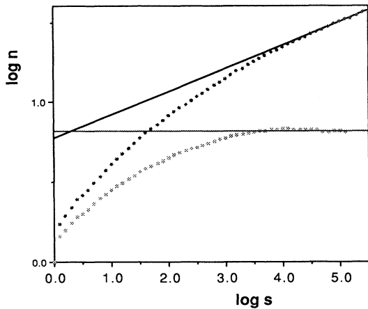
FIG. 20. \langle n(S) \rangle and n_{SURV}(S) for the one-dimensional Zaitsev model with L = 10^4 . d_s = 0.15 \pm 0.03 . The asymptotic value of the slope of \langle n(S) \rangle is \eta = 0.0 \pm 0.006 .
