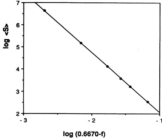
FIG. 12. The average size of avalanches \langle S \rangle vs (f_c - f) for the 1D evolution model. The asymptotic slope yields \gamma = 2.71 \pm 0.02 .
