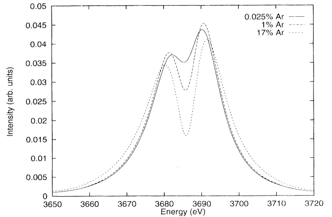
FIG. 1. Area-normalized dynamic Stark-broadened Ar He- \beta line shapes, calculated for 0.025% ( \nu=3.37 eV), 1% ( \nu=1.66 eV), and 17% Ar in D_2 ( \nu=0.621 eV); n_e=5 \times 10^{23} cm ^{-3} and kT=900 eV.
