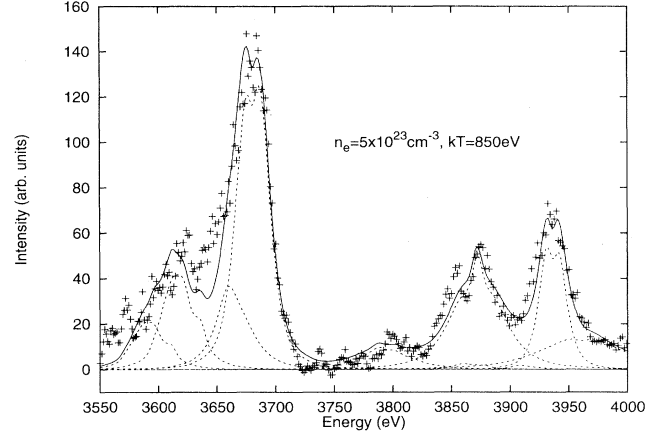
FIG. 10. Best fit to lineout B -3 (1% Ar in D_2 ), for n_e = 5 \times 10^{23} \text{ cm}^{-3} and kT = 850 \text{ eV} . The dashed traces are the individual line profiles that were added to produce the model spectrum.
