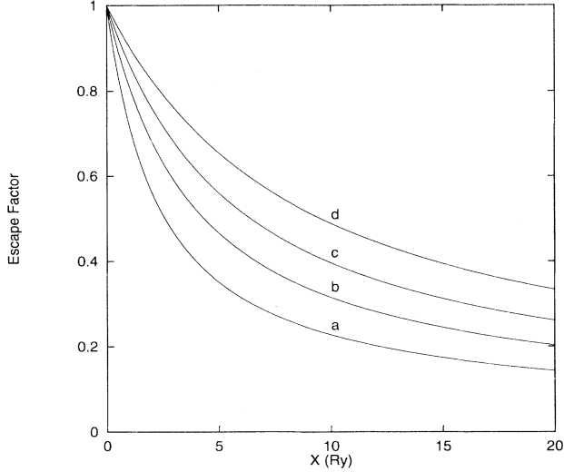
FIG. 3. Escape factors for the He- \beta line vs X = \tau_\omega / \phi(\omega) = \tau_0 / \phi_0 for several values of the electron density N_e : (a) 2 \times 10^{23} \text{ cm}^{-3} ( \phi_0 = 0.2454 \text{ Ry}^{-1} ), (b) 5 \times 10^{23} \text{ cm}^{-3} ( \phi_0 = 0.1392 \text{ Ry}^{-1} ), (c) 1 \times 10^{24} \text{ cm}^{-3} ( \phi_0 = 0.1041 \text{ Ry}^{-1} ), and (d) 2 \times 10^{24} \text{ cm}^{-3} ( \phi_0 = 0.0826 \text{ Ry}^{-1} ).
