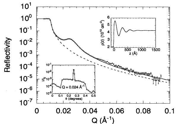
FIG. 2. Neutron reflectivity (circles) from the microemulsion at a hydrophobic silicon interface. The lower inset shows a rocking curve taken at Q=0.024 \text{ \AA}^{-1} . The dashed line is the calculated reflectivity if the microemulsion were structureless and the solid line displays the fit corresponding to the scattering length density profile shown in the upper inset ( d_s=270 \text{ \AA} and \xi_s=217 \text{ \AA} ).
