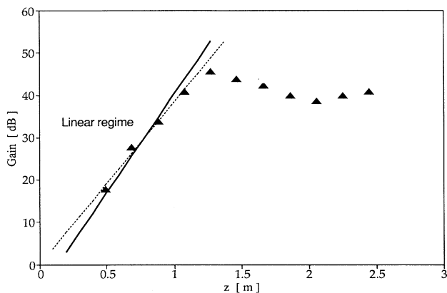
FIG. 2. Comparison of the coupled-mode growth rate calculation with data from the ELF experiments at LLNL.
