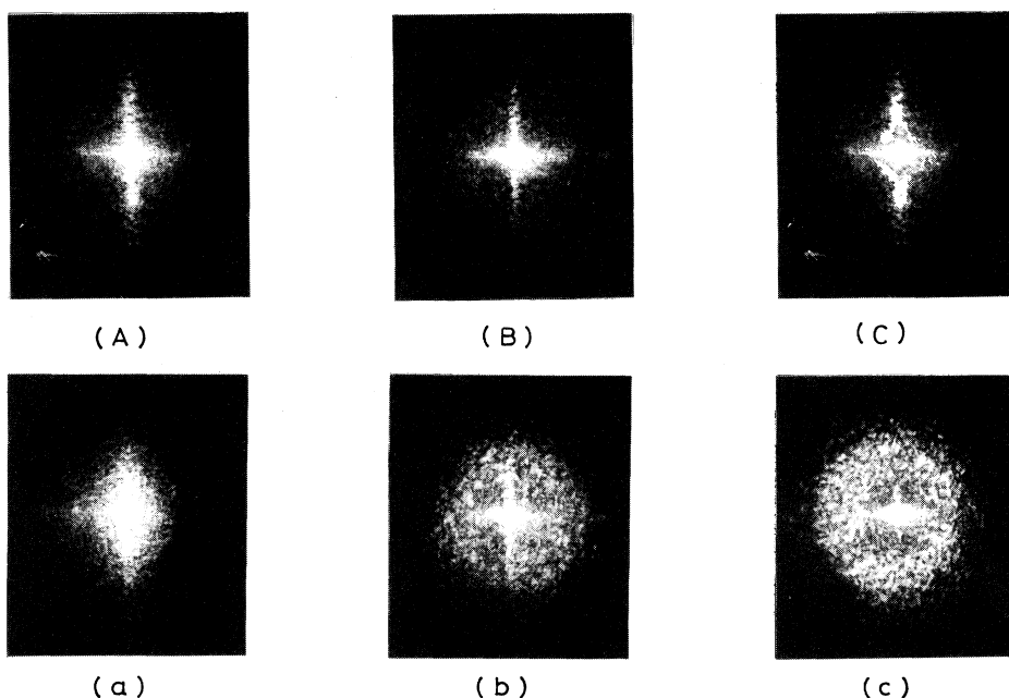
FIG. 3. Patterns of light scattered in the forward direction from the phase-separating critical mixture at T \simeq T_c + 18 mK after cessation of the shear from S \simeq 0.8 \text{ s}^{-1} to 0 [(A) at t \simeq 3 s and (a) at t \simeq 55 s], from S \simeq 7.6 \text{ s}^{-1} to 0 [(B) at t \simeq 10 s and (b) at t \simeq 36 s], and from S \simeq 42 \text{ s}^{-1} to 0 [(C) at t \simeq 3 s and (c) at t \simeq 35 s].
