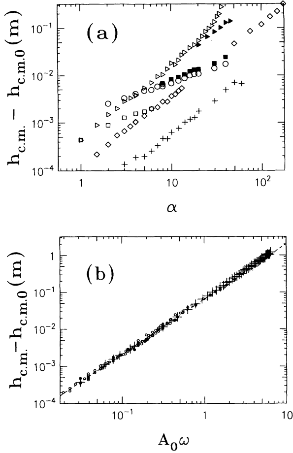
FIG. 2. (a) Log-log plot of h_{c.m.} - h_{c.m.0} as a function of \alpha = A_0 \omega^2 / g for N=50 and \epsilon=0.92 ; the parameters corresponding to the symbols are given in Table I. The averages are taken at phase zero. (b) Plotted are the values of (a) (small circles) and one series of ED simulations (crosses) as a function of A_0 \omega . The parameters used in ED are N=50 , f=100 \text{ s}^{-1} , \epsilon=0.92 , \epsilon_w=0.96 , and 2 \leq \alpha \leq 400 . The results of (a) scale and the dashed line has the slope 1.495.
