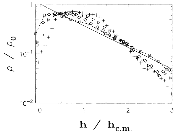
FIG. 5. Logarithmic-linear plot of the normalized number density \rho/\rho_0 for N = 50 , A_0 = 1.55d_0 , and f = 40 \text{ Hz} , such that \alpha = 10 . Here \epsilon equals 0.6 (crosses), 0.8 (triangles), 0.9 (diamonds), and 0.95 (squares, connected by dashed lines). These simulations correspond to the triangles of Fig. 4(a). The straight line corresponds to \exp(-h/h_{c.m.}) .
