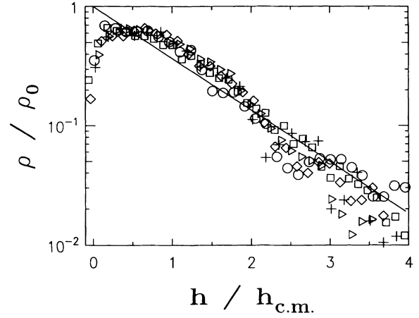
FIG. 3. Logarithmic-linear plot of the normalized number density \rho/\rho_0 for N=50 and \epsilon=0.92 and different f and A_0 values from Fig. 2. We use f=40 \text{ s}^{-1} with A_0/d_0=0.93 such that \alpha=6 (squares), A_0/d_0=2.17 such that \alpha=14 (diamonds), and A_0/d_0=4.7 such that \alpha=30 (circles). These values correspond to the triangles of Fig. 2(a). We also use f=100 \text{ s}^{-1} with A_0/d_0=0.5 such that \alpha=20 (triangles) and A_0/d_0=1.24 such that \alpha=50 (crosses). These values correspond to the diamonds of Fig. 2(a). The straight line corresponds to \exp(-h/h_{c.m.}) .
