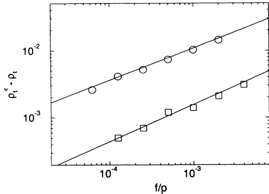
FIG. 5. \rho_i^c - \rho_t in d = 2 (o) and d = 3 ( \square ). The inverse slope yields the exponent \delta .
