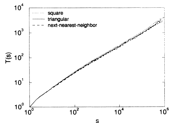
FIG. 9. Fire lifetime T(s) for various lattice symmetries. The inverse slope yields the chemical dimension \mu' .
