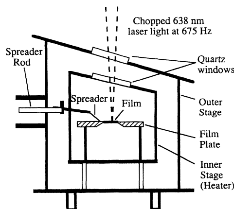
FIG. 1. Oven schematic.
