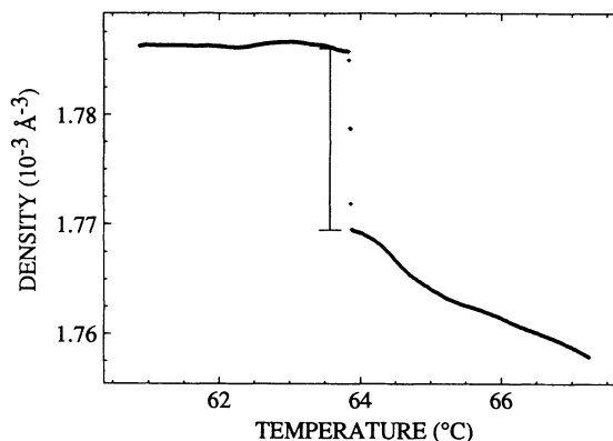
FIG. 6. Density calculated from the reflectivity data presented in Fig. 4. The Hex- B -Cry- E transition appears as a discontinuous jump in the density data. The I beam represents the jump expected based on densities determined from lattice parameters obtained through an x-ray diffraction experiment [15].
