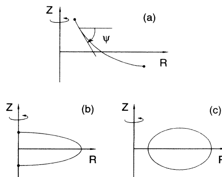
FIG. 1. Three different topologies for an axisymmetric membrane configuration: (a) membrane suspended between two rings, (b) vesicle of spherical topology, and (c) vesicle of toroidal topology. The contour is parametrized by R , Z , and the tilt angle \psi as a function of the contour length S .
