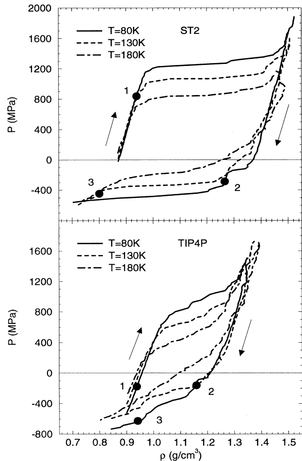
FIG. 2. Response of the density \rho during isothermal compression (up arrows) and decompression (down arrows) of amorphous solid water simulated with ST2 (top panel) and TIP4P (bottom panel), at several different T . The systems fracture at the points of lowest P and \rho shown along the decompression paths. The numbered points (●) identify the states for which the structure is given in Fig. 3.
