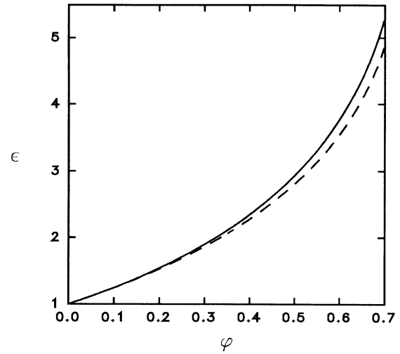
FIG. 2. The relative dielectric constants \epsilon_{\parallel} (solid line) and \epsilon_{\perp} (dashed line) as a function of the volume fraction \varphi for \alpha = \epsilon_p / \epsilon_f = 10 .
