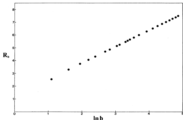
FIG. 3. Data for the electrical resistance R_b (of the fractal generators) plotted against \ln b . One can see that all data (except those for small b ) comprise a straight line. The least-squares fit to the data is given by Eq. (2.3).
