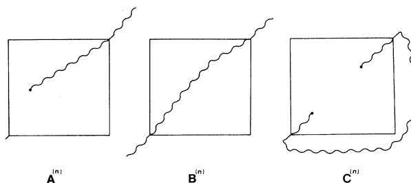
FIG. 4. A diagrammatic representation of the three restricted partition functions for an n th stage of the fractal construction of a member of the PF family. The fractal interior structure is not shown. Thus, for example, A^{(n)} represents the SAW path that starts somewhere within the n th stage fractal structure and leaves it at its upper right link to rest of fractal.
