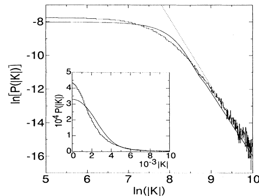
FIG. 3. Same as Fig. 1 but for the symplectic kicked top. The comparison is made with the distribution given by Eq. (3.22). For details see text.
