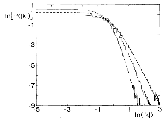
FIG. 8. Same as Fig. 7 but in the logarithmic scale showing agreement in the large- k limit.
