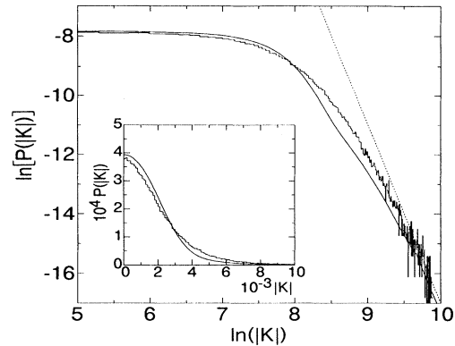
FIG. 2. Same as Fig. 1 but for the unitary kicked top. The comparison is made with the distribution given by Eq. (3.19). For details see text.
