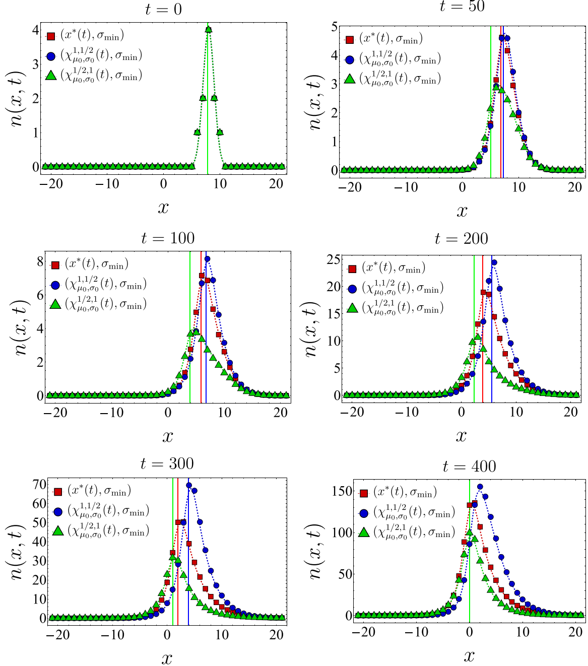
FIG. 9. Snapshots of the B cell population at different times, corresponding to the vaccination protocols of the left panel in Fig. 4. In each case, the dashed curves represent the mean-field numerical solution, while the solid data points depict the SSA sample averages taken over 1000 realizations. The vertical lines in different colors (red, blue, green) indicate the location of the (moving) vaccine center for the corresponding protocol.
