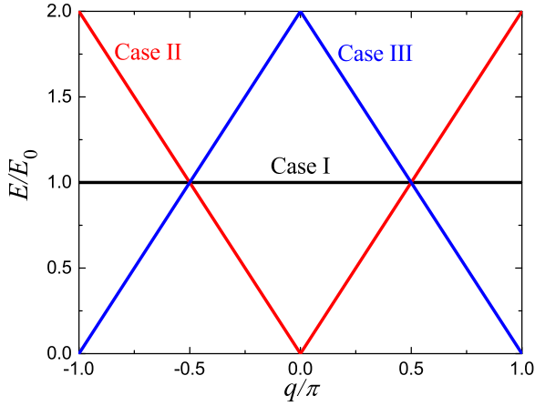
FIG. 2. Three types of energy distribution over phonon modes: case I, all modes have the same energy as in thermal equilibrium at high temperatures; case II, short-wavelength modes have higher energy than long-wavelength ones; case III is opposite to case II. Cases II and III describe nonequilibrium states.
