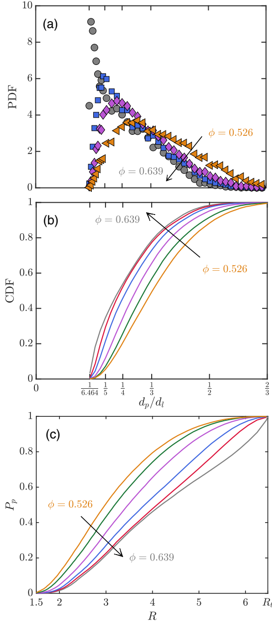
FIG. 12. (a) Pore-throat size distributions, (b) corresponding cumulative distribution functions (CDF), and (c) passing probabilities versus R = d_l/d_f for different \phi . Color and corresponding \phi values are as in Fig. 3, and only data for \phi = 0.526, 0.577, 0.607 , and 0.639 are shown in (a) for clarity.
