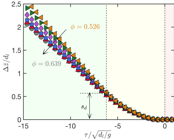
FIG. 4. Trapping regime: Conditionally averaged nondimensional mean vertical displacement versus nondimensional time interval with respect to trapping time for fine particles with R = 5 at different \phi . Symbols are defined in Fig. 3. The three regions show where fine particles percolate at a constant velocity (green), decelerate (yellow), and stop (red). Stopping distance, s_d , is the vertical distance over which fine particles slow to a stop.
