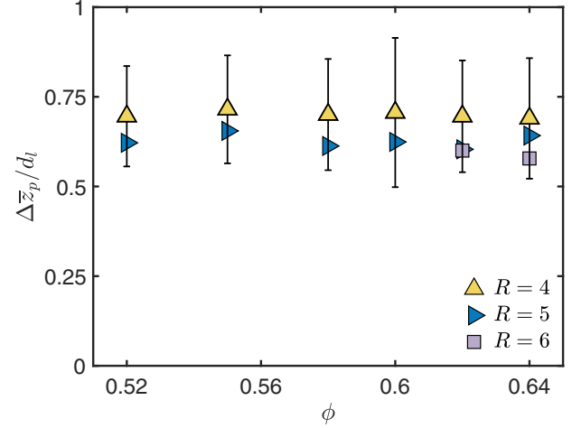
FIG. 13. Average vertical distance normalized by large particle diameter, \Delta\bar{z}_p/d_l , between passable pore throats on the paths of all fine particles for different particle size ratios R at different packing densities \phi . Uncertainty bar depicting the standard deviation of the measurement is only shown for R = 4 for clarity.
