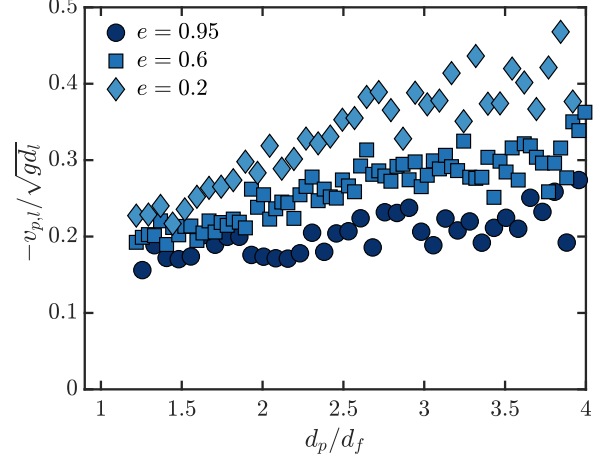
FIG. 15. Nondimensional local percolation velocity, v_{p,l}/\sqrt{gd_l} , versus pore throat to fine particle size ratio, d_p/d_f , for three restitution coefficients with R = 7 and \phi = 0.577 .
