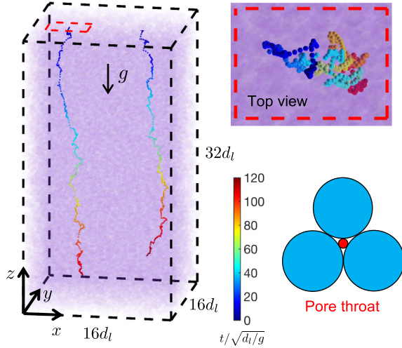
FIG. 1. Left: Perspective view of computational box and two representative fine-particle trajectories (sampled at 5 ms intervals) in the free sifting regime ( R = 6.5 ) for a static large-particle bed with \phi = 0.577 . Color map indicates dimensionless time, t/\sqrt{d_l/g} , during the trajectory. Upper right: Top view of the trajectory of one particle. Bottom right: Pore throat with a fine particle (red) at the geometrical trapping threshold limit.
