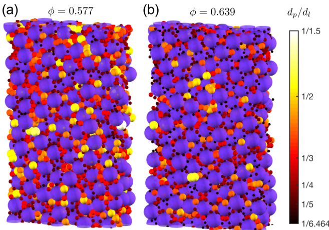
FIG. 11. Two randomly packed large particle beds (purple spheres) and corresponding pore-throat spheres (color map indicates pore-throat size) obtained using the L1 method [32] for (a) \phi = 0.577 and (b) \phi = 0.639 .
