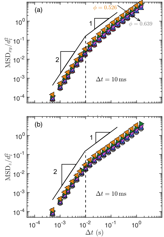
FIG. 6. Nondimensional mean squared displacement (MSD) of fine particles versus time interval \Delta t in the passing regime ( R = 7 ): (a) projected to the xy plane (horizontal) and (b) in the z direction (vertical). Results for various \phi are shown, and symbols are defined in Fig. 3.
