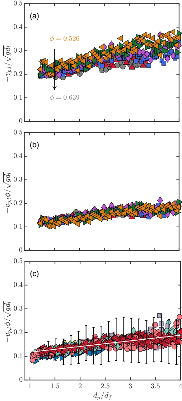
FIG. 14. (a) Nondimensional local percolation velocity, v_{p,l}/\sqrt{gd_l} , versus pore throat to fine particle size ratio, d_p/d_f , for R = 7.5 at various \phi . Symbols are defined in Fig. 3. (b) Multiplying v_{p,l}/\sqrt{gd_l} by \phi collapses the data. (c) Additional data for other size ratios, 4 \leq R \leq 7.5 , both in the trapping and passing regimes with symbols defined in Fig. 5(a), and the full range of packing densities (not differentiated by symbols) also collapse. Uncertainty bars indicate the standard deviation of the measurement for \phi = 0.577 and R = 7.5 . The white line is a linear fit through the data.
