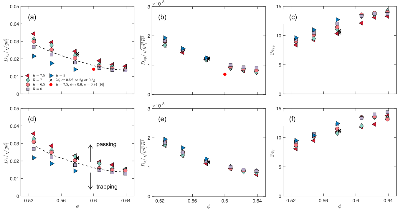
FIG. 7. Diffusion coefficient in the (a)–(c) xy plane projection (horizontal) and (d)–(f) z direction (vertical) scaled by (a), (d) large particle diameter, \sqrt{gd_l^3} ; (b), (e) \sqrt{gd_l^3 R^3} ; and (c), (f) expressed as Péclet numbers versus packing density for various R in the passing and trapping regimes for restitution coefficient e = 0.8 . Data symbols for R = 7 and \phi = 0.577 at different simulation conditions, as indicated in (a), are offset slightly to the right to make them more visible. Dashed curves in (a), (d) approximate the boundary between passing (above) and trapping (below) regimes.
