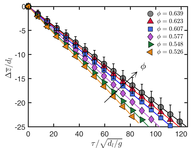
FIG. 3. Passing regime: Nondimensional mean vertical displacement versus nondimensional time interval for fine particles with R = 7 at various \phi .
