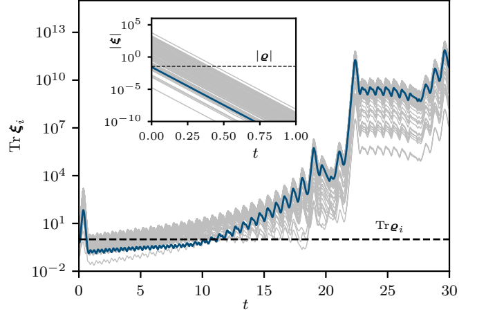
FIG. 2. For the Lorenz-Fetter model, the trace of the unnormalized density matrix, \xi_i(t) [see Eq. (2) for k = 1 ], as a function of time for i = 1, \dots, 100 tangent vectors. Each vector is a local perturbation with elements sampled from a uniform distribution. The inset shows the evolution of |\xi_i(t)| . For each tangent vector, we express \xi_i in terms of its complete set of linearly independent basis vectors. The determinant in each case decays at rate given by instantaneous Lyapunov exponent \langle \mathbf{A}_+ \rangle . An example of a normalized tangent vector evolving on the Lorenz attractor in Fig. 1 is shown in blue. The trace and determinant of the normalized density matrix \rho (inset) are time invariant (dashed).
