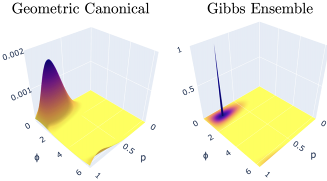
FIG. 1. Alternate ensembles in the geometric and standard settings: differences are plainly evident. Canonical probability distributions on a qubit's state manifold \mathbb{C}P^1 with coordinates Z = (Z^0, Z^1) = (\sqrt{1-q}, \sqrt{q}e^{i\chi}) where q \in [0, 1] and \chi \in [-\pi, \pi] . \mathbb{C}P^1 discretized using a 100 \times 100 grid on the (q, \chi) coordinates exploiting the fact that, with these coordinates, the Fubini-Study measure is directly proportional to the Cartesian volume element dV_{\text{FS}} = dq d\chi/2 . The Hamiltonian is H = \sigma_x + \sigma_y + \sigma_z , with \hbar = 1 and inverse temperature \beta = 5 ( k_B = 1 ). (Right) Gibbs ensemble, where the measure is concentrated around coordinates of the respective eigenvectors (q(|E_0\rangle), \chi(|E_0\rangle)) = (0.789, -2.356) and (q(|E_1\rangle), \chi(|E_1\rangle)) = (0.211, 0.785) . (Left) Geometric canonical ensemble. Notice the difference in scale, due to the fact that the geometric canonical ensemble has continuous support on the quantum state space, not just on single points (energy eigenstates).
