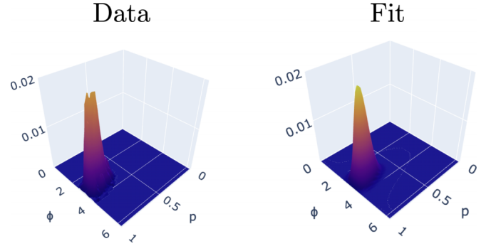
FIG. 2. Comparing time-aggregated data of a single trajectory generated by Eq. (15)’s stochastic model (left) to the fit to a geometric canonical ensemble with functional form as in Eq. (9) (right). Here, h(Z) = E(p, \phi) = \delta \langle \sigma_x \rangle + \epsilon \langle \sigma_z \rangle = \delta 2\sqrt{p(1-p)} \cos \phi + \epsilon(1-2p) , with \delta = \epsilon = 1 . The excellent agreement is visually clear, and it is quantified by a total variation distance between the two distributions of f \approx 5.6 \times 10^{-4} .
