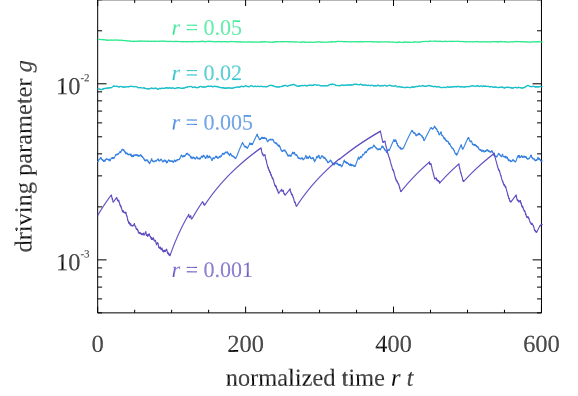
FIG. 8. The value of the simulation driving parameter g as a function of time. Time is normalized by the rate r such that on average one droplet should exit per unit normalized time. Stretches of data where g increases are due to periods where the system is clogged. The values of the rate r are as indicated.
