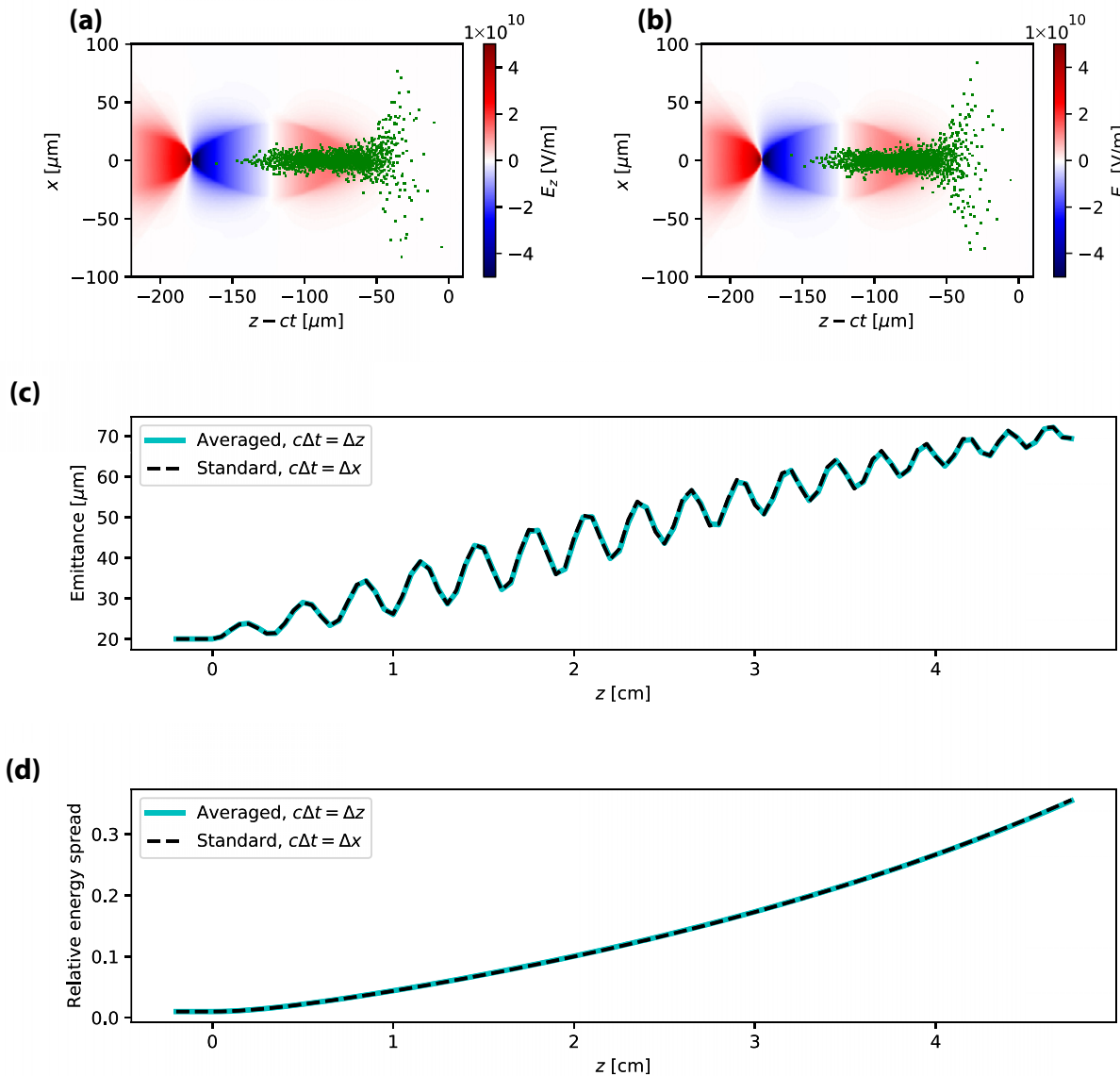
FIG. 6. Algorithm comparison for a 3D plasma-wakefield simulation. (a), (b) Snapshot of the E_z field ( \langle E_z \rangle ) in the case of the averaged Galilean PSATD in the laboratory frame, for the small-timestep ( c\Delta t = \Delta x ) standard Galilean PSATD simulation (a) and large-timestep ( c\Delta t = \Delta z ) averaged Galilean PSATD simulation (b) with fixed \Delta z = 6.4\Delta x . The green dots are representative random samples of the macroparticles in the beam driver. (c), (d) Evolution of the emittance and relative energy spread of the beam, in the laboratory frame.
