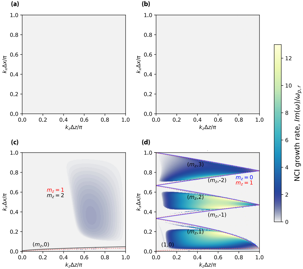
FIG. 1. NCI growth rate of the Galilean PSATD scheme. Normalized NCI growth rate \text{Im}(\omega)/\omega_{p,r} in spectral (k_x, k_z) space, calculated from the analytical stability analysis for different Galilean velocities v_{\text{gal}} = v_0 (a), (b) and v_{\text{gal}} = 0.99 v_0 (c), (d), and for different timesteps c\Delta t = \Delta x (left) and c\Delta t = 6\Delta x (right). The solid and dotted lines correspond to well-known aliased NCI resonant modes, with alias number (m_z, n) , as given by Eq. (1). In this simulation, a uniform plasma drifts at a velocity v_0 = c(1 - 1/\gamma_b^2)^{1/2} with \gamma_b = 130 , and the transverse and longitudinal cell sizes are \Delta x = 6.4 \times 10^{-2} k_{p,r}^{-1} and \Delta z = 6\Delta x , respectively (where k_{p,r}^2 = n_0 e^2 / (m_e \epsilon_0 c^2 \gamma_0) , and where n_0 is the plasma density).
