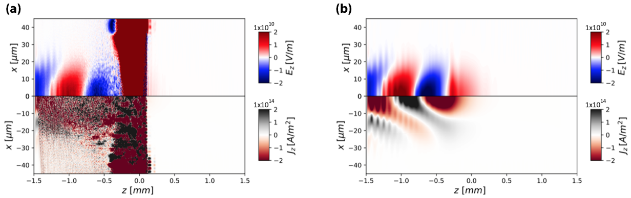
FIG. 5. Instability mitigation in a 3D laser-wakefield simulation with large timestep. The upper half of each subplot shows the E_z field seen by the macroparticles, i.e., the regular E_z field for the standard Galilean PSATD (a), and the averaged \langle E_z \rangle field for the averaged Galilean PSATD (b). The lower half of each subplot shows the longitudinal current density J_z of the plasma. All the fields are shown in the boosted frame with c\Delta t = \Delta z = 10\Delta x .
