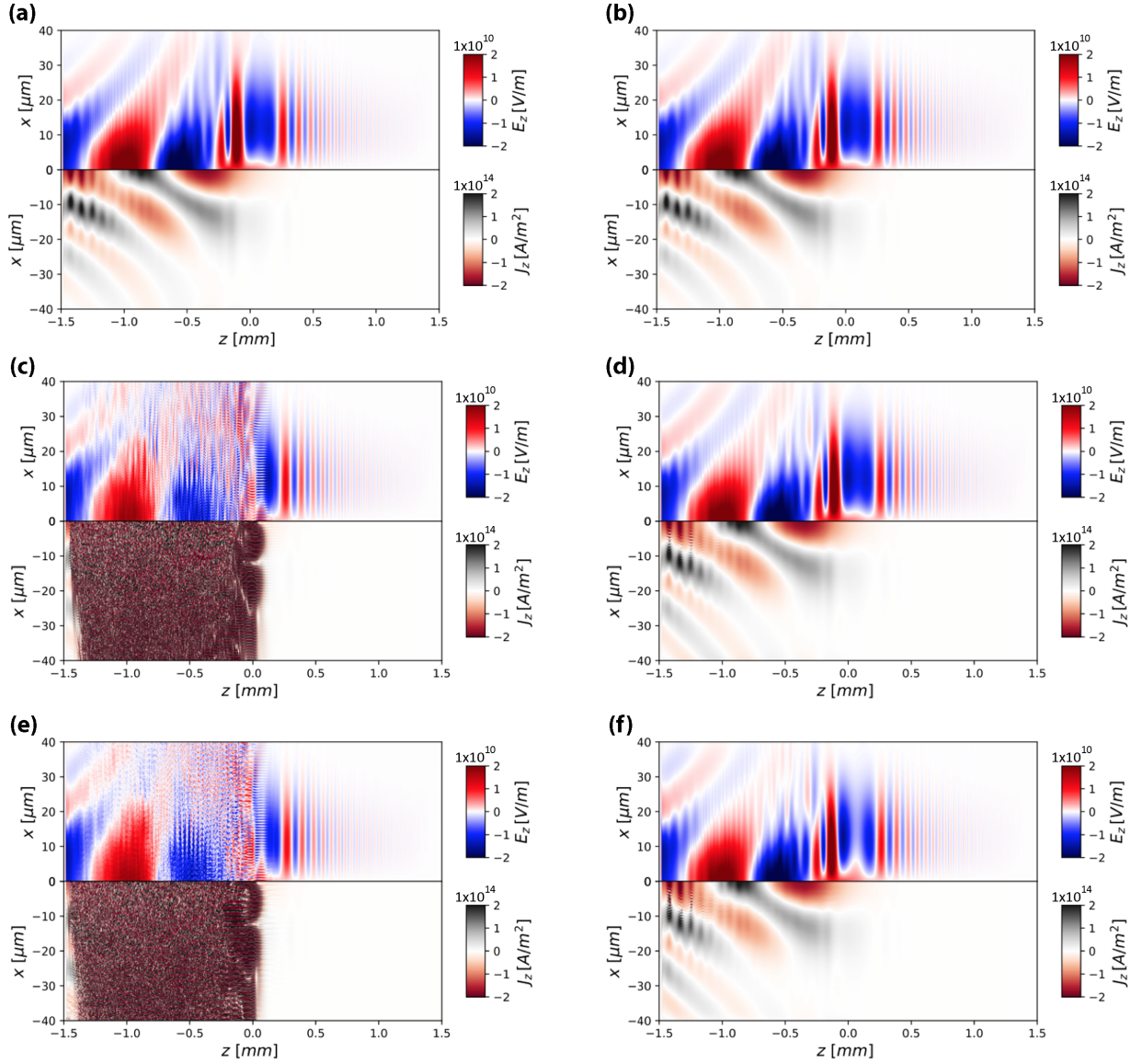
FIG. 4. Instability mitigation in a 2D laser-wakefield simulation with large timestep. The upper half of each subplot shows the E_z field seen by the macroparticles (i.e., the regular E_z field for the standard Galilean PSATD, and the averaged ( E_z ) field for the averaged Galilean PSATD). The lower half of each subplot shows the longitudinal current density J_z of the plasma. All the fields are shown in the boosted frame. The different subplots correspond to the standard Galilean PSATD (a), (c), (e) and averaged Galilean PSATD (b), (d), (f), with c\Delta t = 0.1\Delta z = \Delta x (a), (b), c\Delta t = 0.5\Delta z = 5\Delta x (c), (d), and c\Delta t = \Delta z = 10\Delta x (e), (f).
