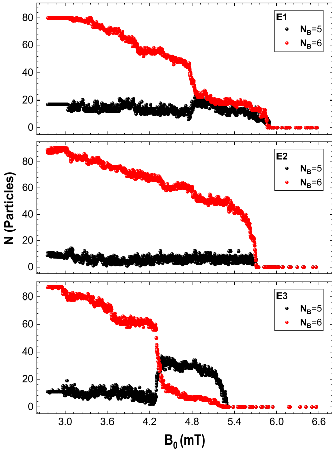
FIG. 11. Number of particles in the aggregate with five and six bonds as a function of the magnetic field, for the three experiments studied here.
