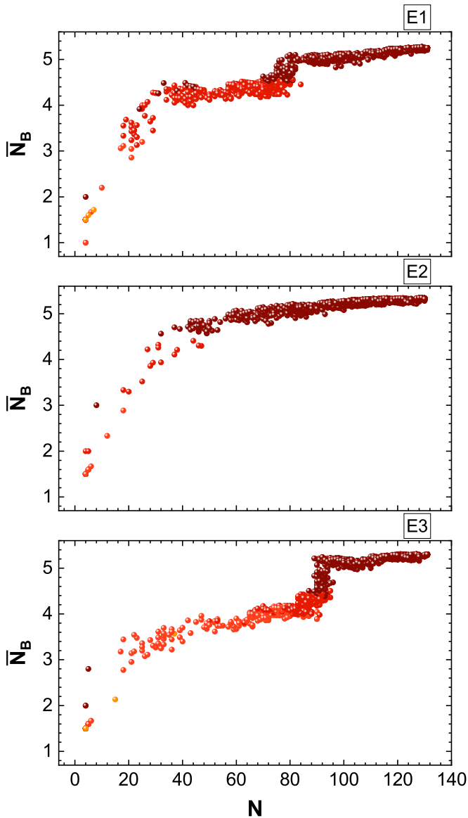
FIG. 9. Average number of bonds N_B as function of the number of particles N in the aggregate. The color indicates the mean value of \psi'_6 , matching the color key of Fig. 3(f).
