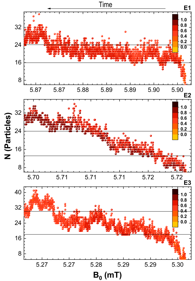
FIG. 12. Number of particles in the aggregate as a function of the magnetic field amplitude with a time resolution of 1/60 s. The horizontal lines separate out the early stage, middle stage, and late stage of growth. The color indicates the value of \psi'_6 as indicated in the legend.
