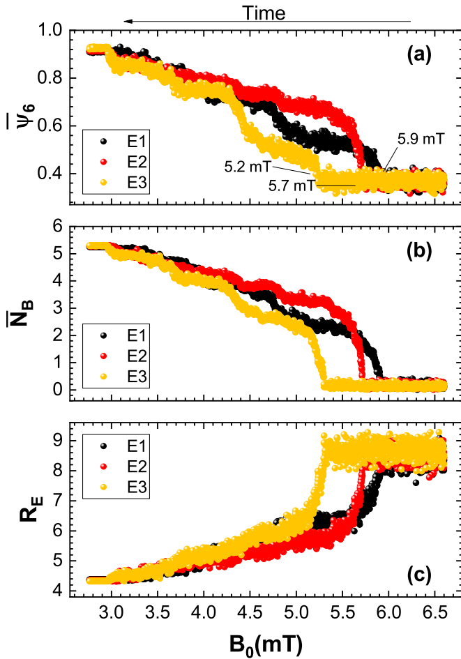
FIG. 5. (a) Average of the configurational order parameter \psi_6 for each frame as a function of magnetic field. (b) Average of the number of bonded neighbors of particles for each frame as a function of magnetic field. (c) Effective system radius in each frame as a function of magnetic field, in units of the particle diameter \sigma .
