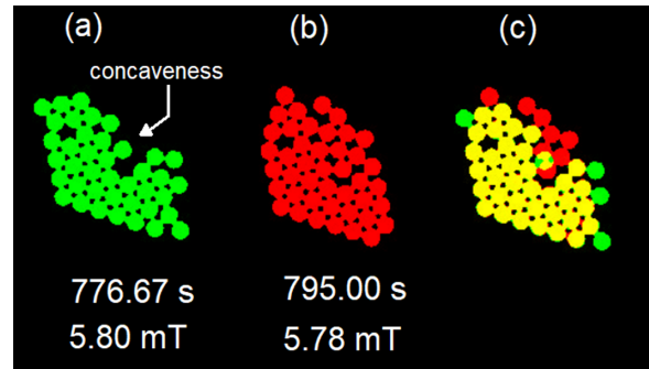
FIG. 15. Comparison between the stable aggregate at two different times from experiment E1. The growth suggests particles are added at concave regions where the new particles can contact more neighbors that help stabilize their presence in the aggregate, and particles with only tenuous connections to the aggregate are easier to “evaporate.”
