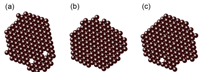
FIG. 4. Final configurations of experiments E1, E2, and E3. The three aggregates have an ordered configuration corresponding to the highest level in the color code of the sixth bond configurational order parameter \psi'_6 , depicted in Fig. 3(f).
