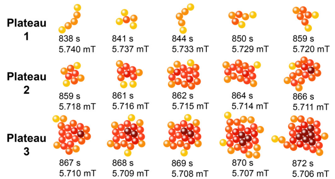
FIG. 13. Sequence of particle configurations in the early formation of a nucleus, corresponding to the data in Fig. 12(E2). The earliest stage has N < 16 particles in the aggregate and corresponds to B_0 \geq 5.716 mT. The second stage has 16 \leq N \leq 24 and corresponds to 5.710 mT \leq B_0 < 5.716 mT. The third stage has N > 24 and B_0 < 5.710 mT. The color of each particle indicates \psi'_6 matching the color key of Fig. 3(f).
