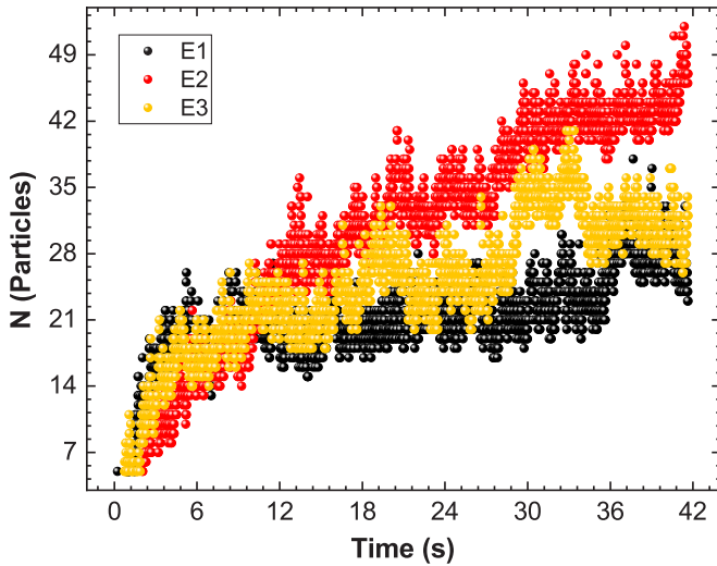
FIG. 14. Comparison of the behavior of the aggregate size as a function of the time elapsed from its formation. Recall the magnetic field amplitude decreases by 0.1 mT in 50 s.
