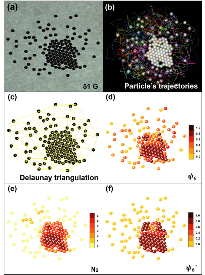
FIG. 3. (a) A typical photo at a certain stage of the experiment, (b) trajectories of particles over 1.66 s (0.83 s before and 0.83 s after the position shown), (c) Delaunay triangulation, (d) \psi_6 order parameter, (e) number of bonded neighbors N_B , and (f) the bond order parameter \psi'_6 , which is calculated based only on touching neighbors (those counted by N_B ). This configuration is the same as shown in Fig. 2(c).
