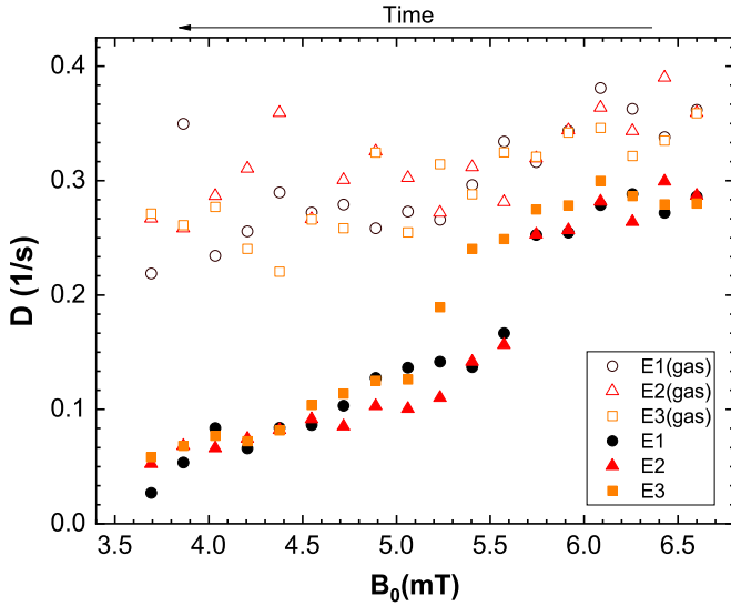
FIG. 7. Effective diffusion coefficient measured in time windows of 4.16 s every 166.66 s. The open symbols correspond to gaseous particles and the filled symbols are averaged over all particles (both gaseous and aggregated). The units are \sigma^2/s in terms of the particle diameter \sigma .
