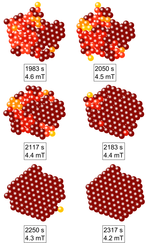
FIG. 10. Sequence of images showing a notable change of structural characteristics. The data are from experiment E3 and the color indicates \psi'_6 of each particle, matching the color key of Fig. 3(f).
