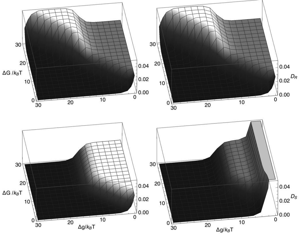
FIG. 6. Diffusivities, D_R (top row) and D_S (bottom row) of the remodeling complex and the SMC complex, respectively, plotted versus \Delta G/(k_B T) and \Delta g/(k_B T) , according to model 1 [Eqs. (16) and (17)] for k_+ = 0.05 per time step, k_- = 5.0 \times 10^{-7} per time step, m_+ = 0.3 per time step, and m_- = 0.0003 per time step (left column) or m_- = 0.3 per time step (right column).
