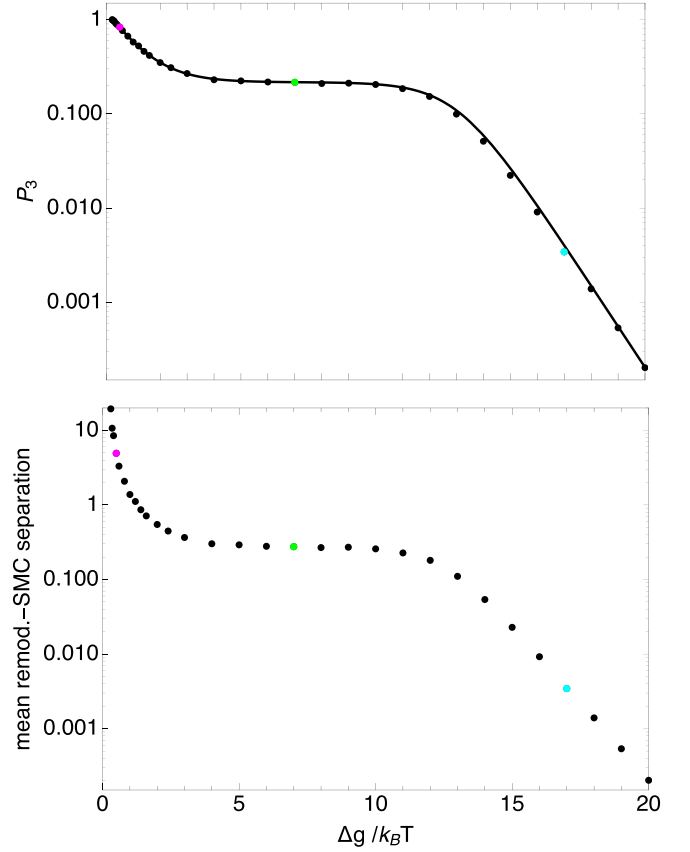
FIG. 4. Probability, P_3 , that the remodeler and SMC are not next to each other (top) and the mean remodeler-SMC separation (bottom), plotted versus nucleosome binding energy, \frac{\Delta g}{k_B T} . The circles correspond to results determined from model-2 Gillespie simulations, each containing 2^{20} transitions. The solid line corresponds to Eq. (30). The parameter values used were k_+ = 0.05 per time step, k_- = 5 \times 10^{-7} per time step, m_+ = m_- = 0.3 per time step, \Delta G = 18.0 k_B T , \alpha = 1 per time step, and \beta = \alpha e^{-\frac{\Delta g}{k_B T}} . These parameters correspond to those for Fig. 2. The cyan, green, and magenta points at \frac{\Delta g}{k_B T} = 0.5, 8.0 , and 18 , respectively, correspond to the bottom, middle, and top traces of Fig. 2.
