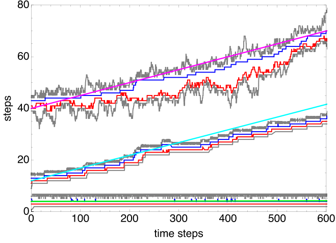
FIG. 2. Three example composite LEF trajectories from model 2 simulations. In each case, the positions versus time of the nucleosome junctions are shown gray, the remodeling complex is shown blue, and the SMC complex is shown red. When tracking together, each such group of four traces constitutes a composite LEF. The model parameters are k_+ = 0.05 per time step, k_- = 5 \times 10^{-7} per time step, m_+ = m_- = 0.3 per time step, \Delta G = 18.0k_B T , \alpha = 1 per time step, and \beta - \alpha e^{\frac{-\Delta g}{k_B T}} for all three composite LEFs, but \Delta g = 18.0k_B T for the bottom group of traces, \Delta g = 9.0k_B T for the middle group of traces, and \Delta g = 0.5k_B T for the top group of traces. The cyan, green, and magenta lines each have a slope given by the theoretical composite LEF velocity for the parameters of each simulation.
