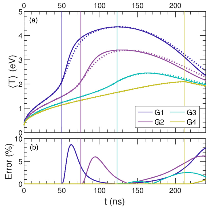
FIG. 7. (a) Comparison of the average temperature \langle T \rangle evolution calculated by the zero-order Taylor series truncation (solid lines), and by including the full radial variation (dotted lines), for the simulation conditions G1–G4 in Table I. The vertical lines indicate the transition time between uniform and quasistatic regimes. (b) Relative error (%) in average temperature \langle T \rangle between the two methods in (a).
