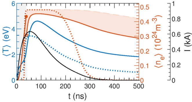
FIG. 5. Comparison of QUEST simulation results and those from Ref. [42] for average electron temperature \langle T \rangle and electron density \langle n_e \rangle as a function of time. The simulation conditions are given by “C” in Table I. Solid lines indicate the QUEST method results, while dotted lines indicate the (digitized) simulation results from Ref. [42].
