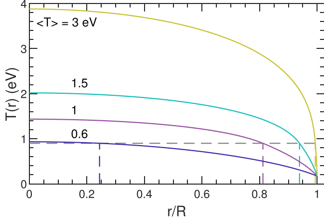
FIG. 1. Radial temperature profiles T(r) , as defined in Eq. (5), for four average temperatures \langle T \rangle . The dashed vertical lines mark the boundary R_b between the plasma-dominated region ( \kappa \propto T^{5/2} ) and the neutral-dominated region ( \kappa \propto T^{1/2} ) which occur at T_b = 0.9 eV, represented by the dashed horizontal line.
