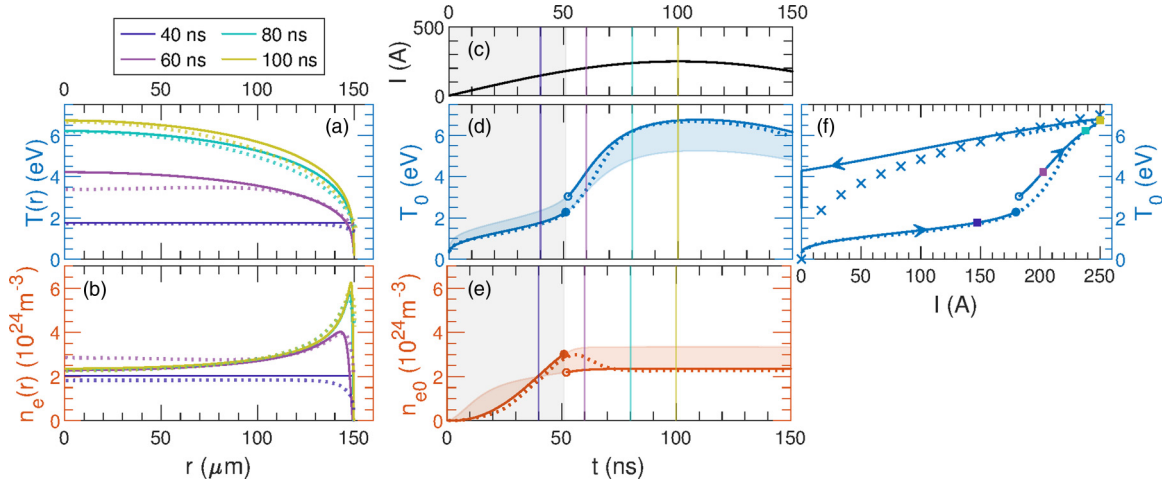
FIG. 3. Comparison of QUEST simulation and 1D MHD simulation [8] results for electron temperature and electron density. The simulation conditions are given by “B” in Table I. (a) Radial electron temperature profiles T(r) for select times corresponding to the vertical lines in (d) and colored square markers in (f). (b) Radial electron density profiles n_e(r) for select times corresponding to the vertical lines in (e). (c) Discharge current profile I . (d) On-axis electron temperature T_0 . (e) On-axis electron density n_{e0} . (f) Variation of the on-axis electron temperature T_0 with current amplitude I . Solid lines indicate QUEST method results, while dotted lines indicate the (digitized) simulation results from Ref. [8] and blue crosses represent calculations using the simplified equilibrium model in Ref. [8]. The colored shaded bands in (d) and (e) represent the range of values between assuming the uniform regime and the quasistatic regime. The shaded grey region indicates the times at which the QUEST algorithm assumes uniform conditions, and marks the transition between the uniform and quasistatic regimes corresponding to the discrete jump in the electron temperature and density profiles.
