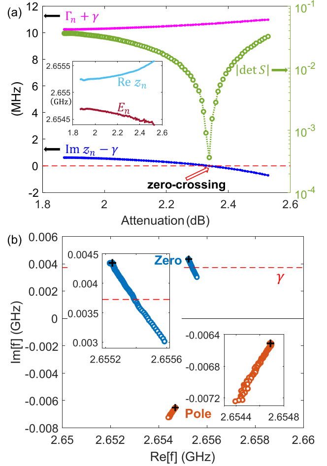
FIG. 2. (a) Fitted parameters \text{Im} z_n - \gamma and \Gamma_n + \gamma for the complex Wigner time delay from graph experimental data. Also shown is the evolution of |\det(S)| at the specific frequency of interest, f_{\text{CPA}} , which reaches its minimum at the zero-crossing point. The inset shows the evolution of \text{Re} z_n and E_n = \text{Re} E_n with attenuation. (b) Evolution of complex zero and pole of a single mode of the graph in the complex frequency plane as a function of \Gamma_A . The black crosses are the initial state of the zero and pole at the minimum attenuation setting. The insets show the details of the complex zero and pole migrations.
