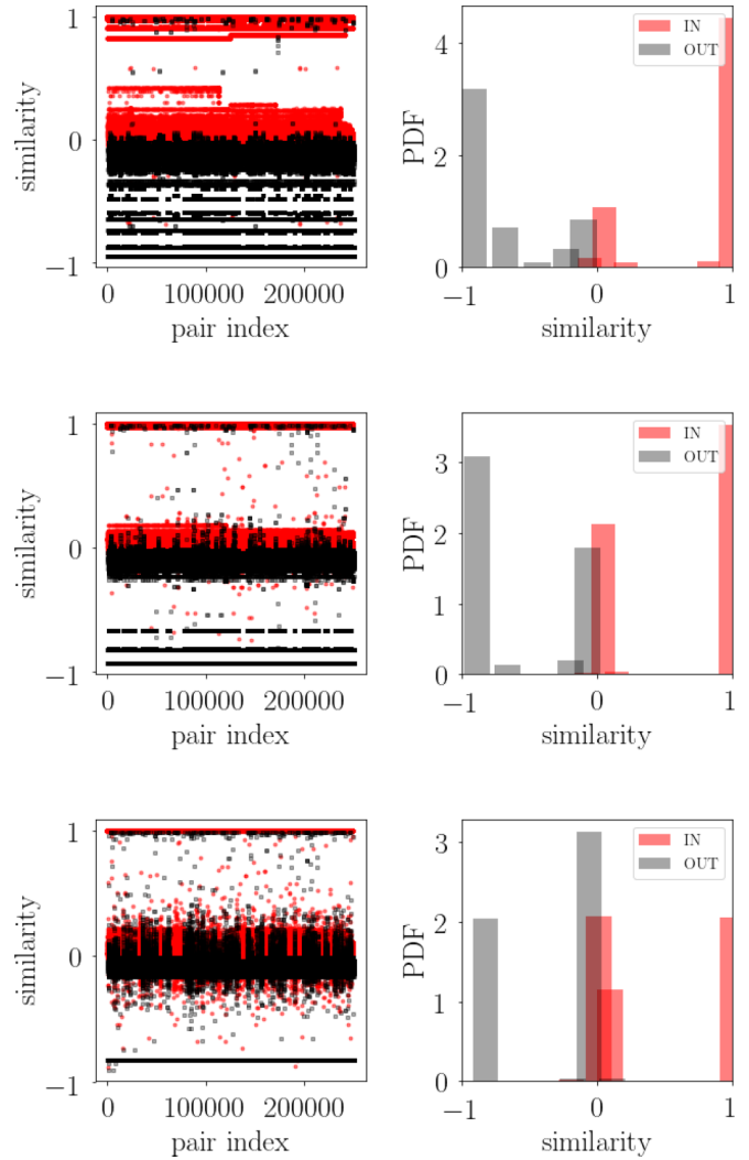
FIG. 12. Problem of spectral embeddings for well-separated communities. The network is generated by an SBM with two blocks, p_{in} = 1 and p_{out} = 0.001 , and N = 500 in each block. Laplacian eigenmap is applied for dimensions d = 20, 50, 100 (top to bottom). The cosine similarity for within cluster node pairs has limited overlap with that of the node pairs across clusters for higher embedding dimension, making the identification of the clusters easier.
