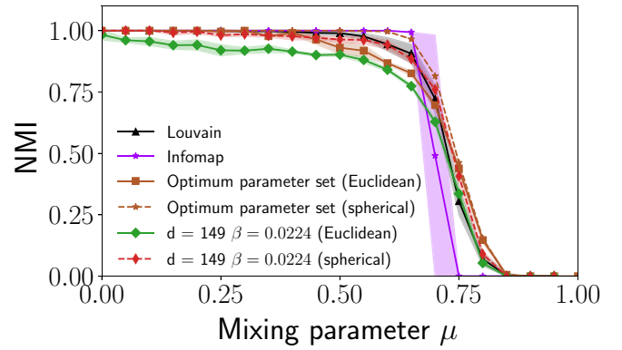
FIG. 3. Performance of higher-order preserving embedding on LFR networks with 1000 nodes. The baseline performances are those of Infomap (star) and Louvain (filled triangle). For each value of the mixing parameter \mu , the average NMI over 10 configurations is reported. The best parameters are found by employing a genetic optimization in two different ways: finding the best parameters for each configuration separately (brown) and finding the optimum parameter set across all values of \mu (green and red, the optimal parameters are indicated) by optimizing the area under the curve. The spherical distance metric (dashed) performs better than the Euclidean metric (solid lines).
