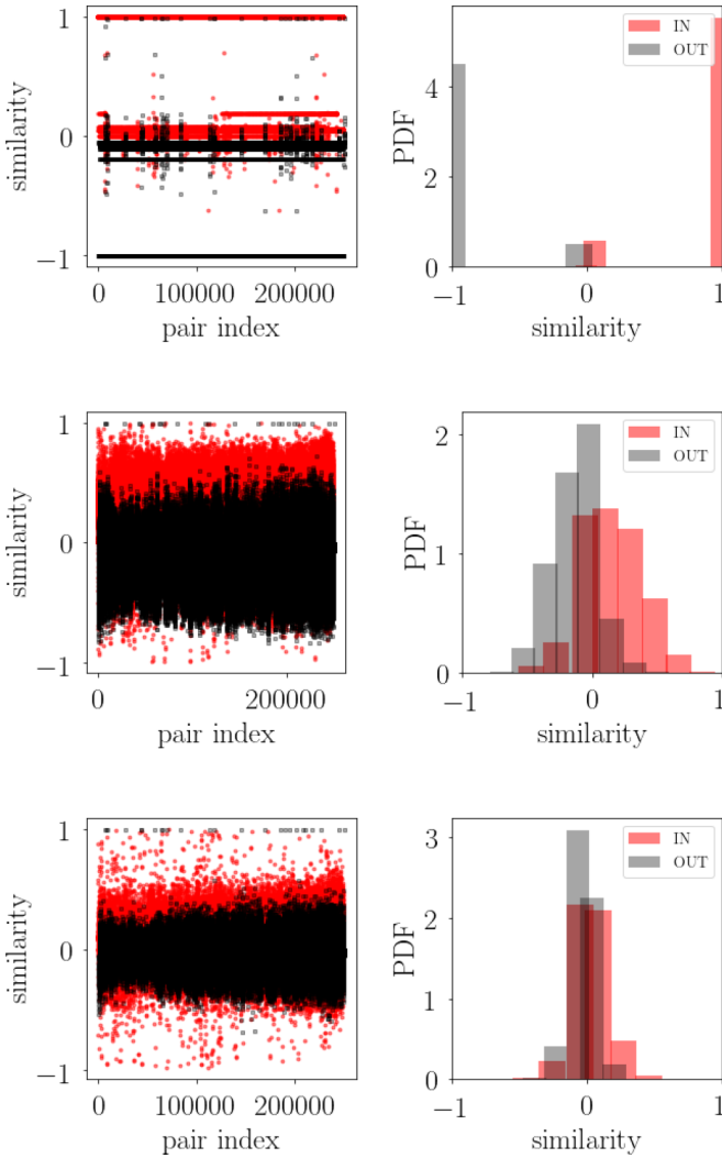
FIG. 11. Problem of spectral embeddings for well-separated communities. The network is generated by an SBM with two blocks, p_{in} = 1 and p_{out} = 0.0001 , and N = 500 in each block. Laplacian eigenmap is applied for dimensions d = 20, 50, 100 (top to bottom). The cosine similarity for within cluster node pairs overlaps with that of the node pairs across clusters for higher embedding dimension, making the identification of the clusters hard even for this straightforward example.
