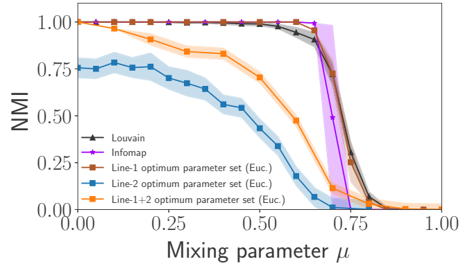
FIG. 7. Performance of large-scale information network embedding on LFR benchmark graphs for 1000 nodes. The baseline performances are those of Infomap (star) and Louvain (filled triangle). The curves show the optimal performance of the three implementations of the method. The first implementation, LINE-1, is clearly the best and outperforms Infomap, albeit by a small margin.
