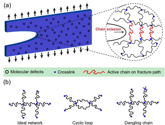
FIG. 1. (a) Schematic illustration of crack propagation in a polymer network with topological defects by fracturing active polymer chains. (b) Cyclic loops and dangling chains are the two most representative types of topological defects in polymer networks.
