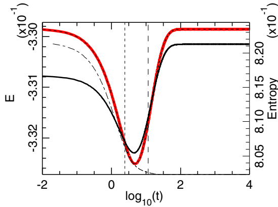
FIG. 11. Reverse-Kovacs effect observed with the three-state model with T'_0 = 0.02 , T'_1 = 0.22 , and T'_2 = 0.17852 . The red curve (numerical result) superimposed on the short-dash black line (theoretical calculation) shows the variation of the energy (left scale) versus time (in log scale) during the time evolution at temperature T'_2 after annealing for 10.12 t.u. at temperature T'_1 . The full black line shows the time evolution of the entropy (right scale) and the thin dash-dot line shows the variation of the entropy production (its scale, not shown on the graph, varies from 0 to 3.0 \cdot 10^{-3} )
