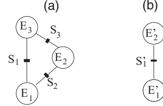
FIG. 1. Picture of the three-state model (a) and its simplified version, the two-state model (b). The circles schematize the metastable states with energies E_i , and the thick lines the barriers that separate them, with energies S_i .
