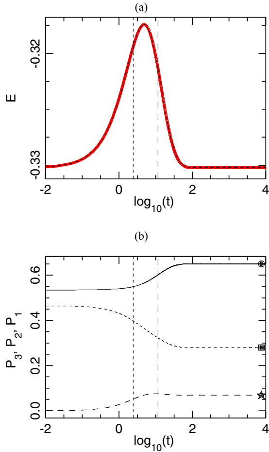
FIG. 3. Energy (a) and probabilities P_1, P_2, P_3 (b) versus time (in log scale) during the time evolution at constant temperature T_2 = 0.17856 after aging for 1.8 \cdot 10^7 t.u. at temperature T_1 = 0.02 in the study of the Kovacs effects. In plot (a), the thick red line shows the numerical result and the short-dash line shows the result of the theoretical calculation (Sec. IV). Plot (b): full line P_1 , short-dash line P_2 , long-dash line P_3 . The points at the right side of the graph show the values of the equilibrium probabilities at T_2 : circle P_1^{\text{eq}} , square P_2^{\text{eq}} , star P_3^{\text{eq}} . In both plots, the vertical lines mark the relaxation times (short-dash line \tau_1 , long-dash line \tau_2 ).
