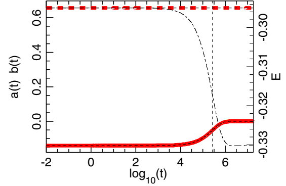
FIG. 5. Amplitudes of the eigenmodes a(t) and b(t) during the aging stage at temperature T_1 in the protocol to observe the Kovacs effect. The thick red lines show the results of the numerical integration with a full line for a(t) and a dash line for b(t) . The short-dash black lines are the results of the analytical calculation. The vertical short-dash line marks the value of \tau_1(T_1) . The thin dash-dot line shows the variation of the energy (right scale).
