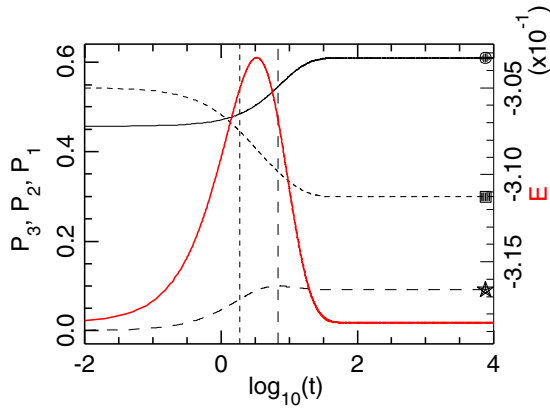
FIG. 10. Energy (red curve, right scale) and probabilities P_1 , P_2 , P_3 (black curves, left scale) versus time (in log scale) during the time evolution at constant temperature T_2 = 0.2110 after aging for 1.8 \cdot 10^7 t.u. at temperature T_1 = 0.02 in the study of the Kovacs effects. The conditions are very similar to the case shown in Fig. 3 except that the aging started from an equilibrium temperature T^{\text{ini}} = 0.50 instead of 0.30 so that the cooling rate was faster. Full black line P_1 , short-dash black line P_2 , long-dash black line P_3 . The points at the right side of the graph show the values of the equilibrium probabilities at T_2 : circle P_1^{\text{eq}} , square P_2^{\text{eq}} , star P_3^{\text{eq}} .
