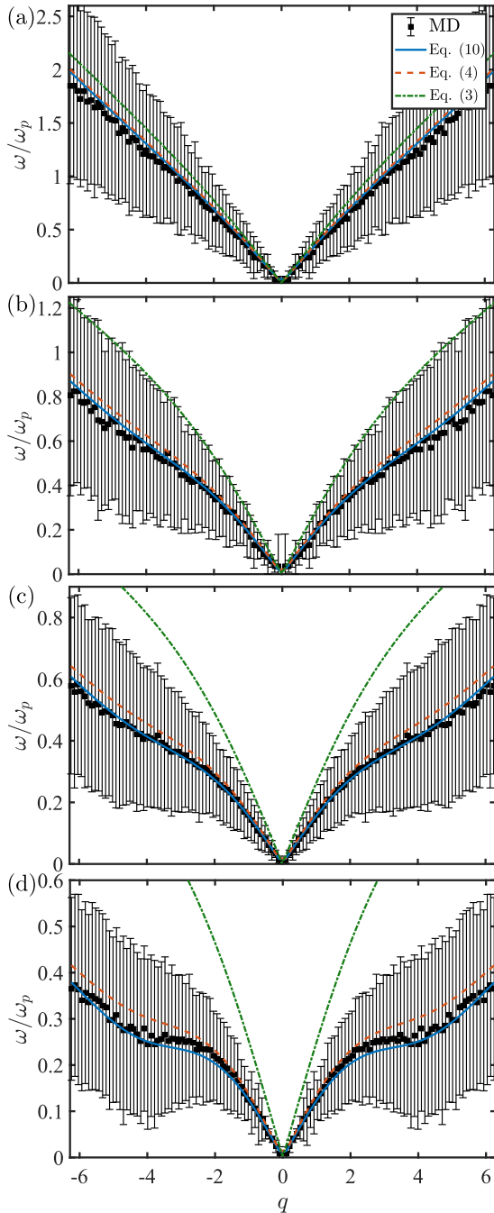
FIG. 6. Dispersion relations in Yukawa fluids with \kappa = 4 . Notation is the same as in Fig. 3. (a) \Gamma = 10 , (b) \Gamma = 50 , (c) \Gamma = 100 , (d) \Gamma = 250 .
