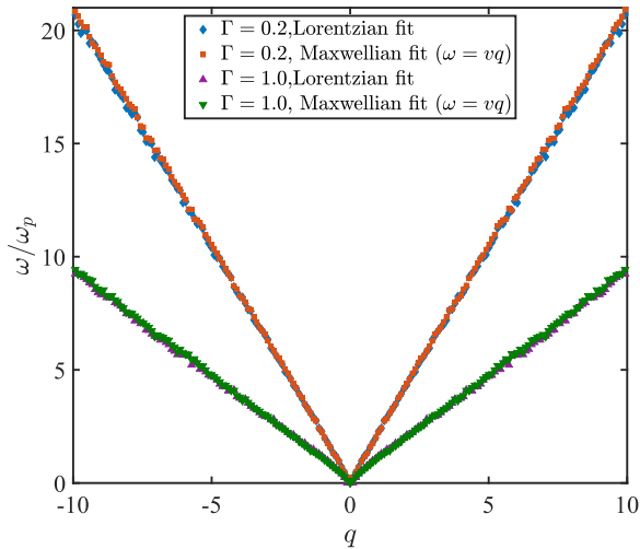
FIG. 8. Reduced frequency \omega/\omega_p versus the reduced wave number q = ka for the two weakly coupled state points, ( \kappa = 1 , \Gamma = 0.2 ) and ( \kappa = 1 , \Gamma = 1 ). The results of analysis using double-Lorentzian and Maxwellian fits are almost indistinguishable.
