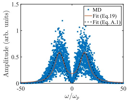
FIG. 7. Example of fitting the MD data by the double-Lorentzian and Maxwellian functions. MD data correspond to the state point with \kappa = 1 and \Gamma = 1 , and the reduced wavelengths is q = 13 . There is some observable difference between the fits, the Maxwellian fit being more appropriate at low frequencies. However, the maximum position is about the same for both fits.
