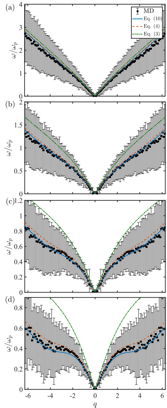
FIG. 5. Dispersion relations in Yukawa fluids with \kappa = 3 . Notation is the same as in Fig. 3. (a) \Gamma = 5.0 , (b) \Gamma = 20 , (c) \Gamma = 50 , (d) \Gamma = 100 .
