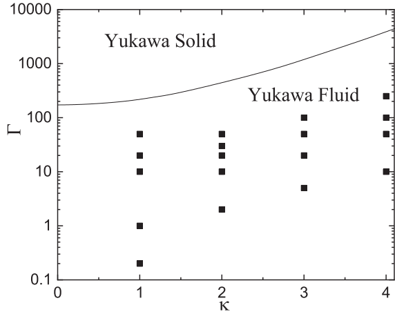
FIG. 1. Phase diagram of Yukawa systems in a (\kappa, \Gamma) plane. The solid curve corresponds to the fluid-solid (melting) phase transition according to the data from Ref. [25]. Symbols correspond to the phase state points investigated in this work.
