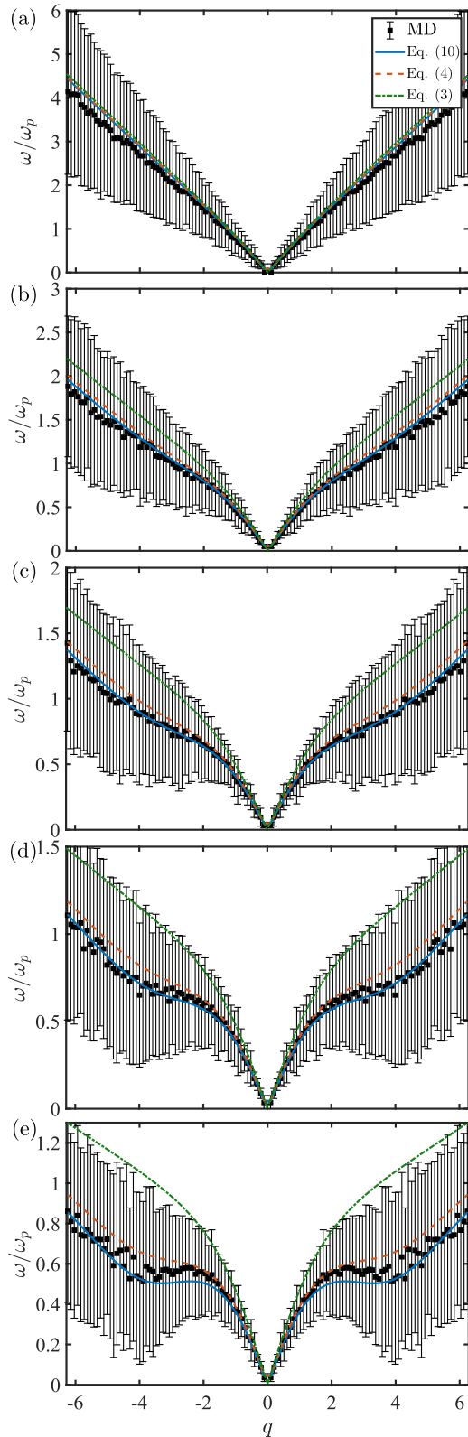
FIG. 4. Dispersion relations in Yukawa fluids with \kappa = 2 . Notation is the same as in Fig. 3. (a) \Gamma = 2.0 , (b) \Gamma = 10 , (c) \Gamma = 20 , (d) \Gamma = 30 , (e) \Gamma = 50 .
