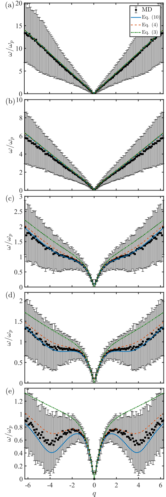
FIG. 3. Dispersion relations in Yukawa fluids with \kappa = 1 . Symbols correspond to numerical results. Curves denote theoretical approximations compared in this work (see the legend). (a) \Gamma = 0.2 , (b) \Gamma = 1.0 , (c) \Gamma = 10 , (d) \Gamma = 20 , (e) \Gamma = 50 .
