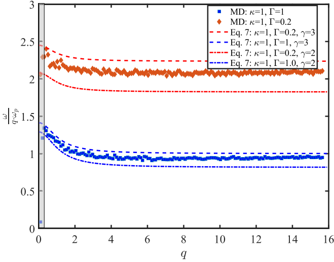
FIG. 2. Ratio \omega/q\omega_p versus the reduced wave number q = ka for the two weakly coupled state points ( \kappa = 1 , \Gamma = 0.2 ) and ( \kappa = 1 , \Gamma = 1 ). The shaded area corresponds to the regime of insufficient statistics due to finite simulation volume [this approximately corresponds to q \lesssim 2\pi/(L/2) \simeq 0.2 , where L is the size of the simulation box]. The dashed (dotted) curves correspond to Eq. (3) with \gamma = 3 ( \gamma = 2 ).
