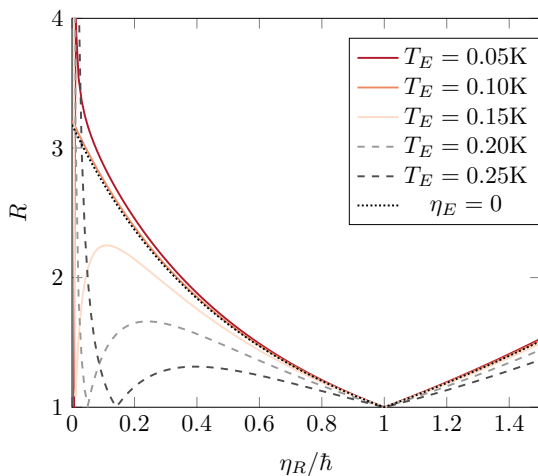
FIG. 5. Influence of a third bath on the rectification index R , as defined in (60). The coupling to the third bath is \eta_E = 0.1\hbar , T_L = 0.1 K, and T_R = 0.2 K. The other parameters are given in the caption of Fig. 3.
