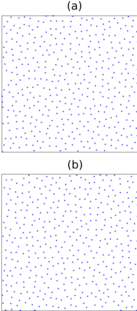
FIG. 27. (a) Two-dimensional configuration of 400 particles drawn from ensembles in which the target function S_0(k) is taken to be equal to the numerically measured S(k) of a perfect-glass system at \rho = 0.003\,906\,25 . (b) Actual perfect-glass configuration with the same pair statistics g_2(r) and S(k) .
