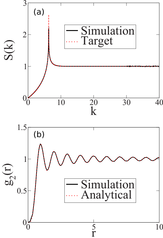
FIG. 4. (a) Structure factor obtained by sampling ensembles of 1D configurations in which the target function S_0(k) is taken to be Eq. (50) at \rho = 1 . (b) Corresponding pair correlation function sampled from simulations and the analytical formula (53).
