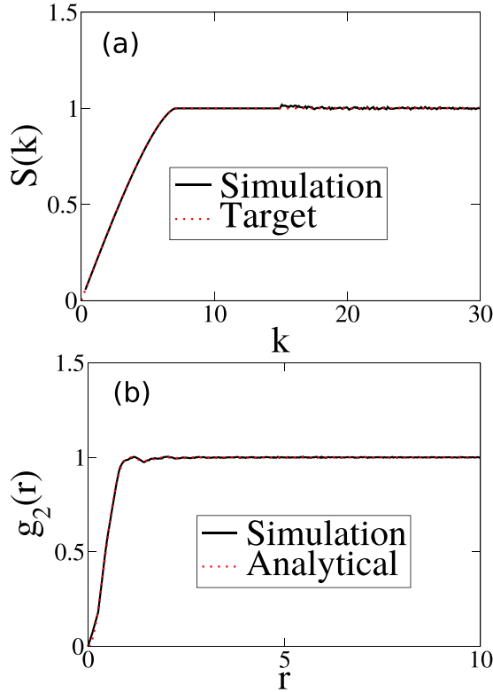
FIG. 6. (a) Structure factor obtained by sampling ensembles of 2D configurations in which the target function S_0(k) is taken to be Eq. (56) at \rho = 1 . (b) Corresponding pair correlation function sampled from simulations and the analytical formula (57).
