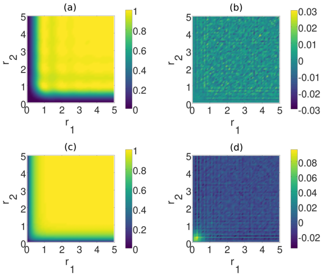
FIG. 30. (a) Analytical three-body correlation function g_3(r_1, r_2) of the 1D Fermi-sphere system. (b) Difference in g_3 between the targeted system and the 1D Fermi-sphere system \Delta g_3(r_1, r_2) = g_3^{\text{fermionic}}(r_1, r_2) - g_3^{\text{targeted}}(r_1, r_2) . (c) and (d) Same as (a) and (b) but for the 1D Lorentzian target.
