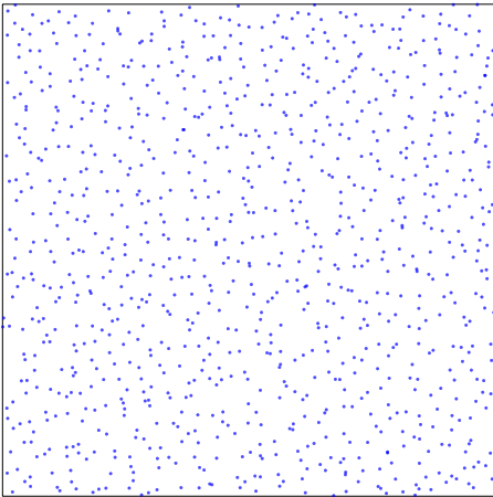
FIG. 22. Two-dimensional 1000-particle hyposurficial configuration drawn from ensembles in which the target function S_0(k) is numerically computed from Eqs. (2) and (75) at \rho = 0.5 .
