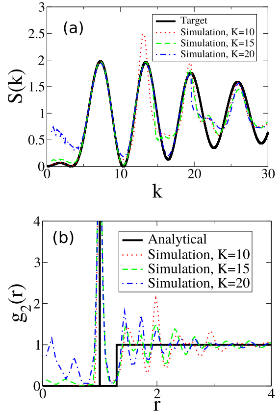
FIG. 11. (a) Structure factor obtained by sampling ensembles of 1D configurations in which the target function S_0(k) is taken to be Eq. (61) at \rho = 1 . (b) Corresponding pair correlation function sampled from simulations and the analytical formula (60).
