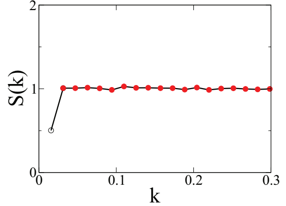
FIG. 28. Structure factor for the 1D system with energy E = S(q)(1/S_0 - 1) , where q is the smallest wave vector and S_0 = 0.5 , at temperature k_B T = 1 . As discussed in the text, the effect of this energy is to constrain the structure factor at q to S_0 = 0.5 (open circle) and leave the structure factor at other wave vectors unconstrained (closed red circles).
