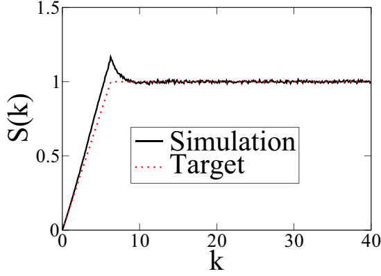
FIG. 29. Structure factor for the 1D system with energy given in Eq. (A1), in which S_0(\mathbf{k}) is given in Eq. (49), at temperature k_B T = 1 .
