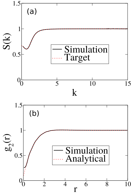
FIG. 21. (a) Structure factor obtained by sampling ensembles of 3D configurations, in which the target function S_0(k) is taken to be Eq. (77), at \rho = \frac{1}{4\pi} . (b) Corresponding pair correlation function sampled from simulations and the analytical formula (76).
