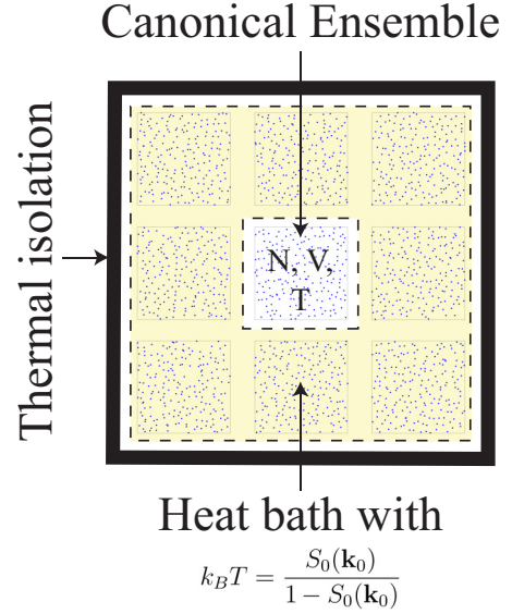
FIG. 1. When a large number of systems can exchange heat with each other but not with the environment, one can focus on one system (central one indicated with a white background) and treat the rest as a heat bath (systems having yellow background). The central system with fixed N , V , and T follows the distribution function of a classical canonical ensemble with a temperature T determined by the total energy of the systems and degeneracy of the heat bath. For the problem at hand, we show that the temperature is determined by the target structure factor S_0(\mathbf{k}) , as specified by the relation k_B T = S_0(\mathbf{q})/[1 - S_0(\mathbf{q})] .
