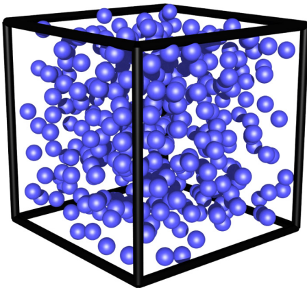
FIG. 19. Three-dimensional 400-particle configuration drawn from ensembles in which the target function S_0(k) is taken to be Eq. (69) at \rho = 1 .
