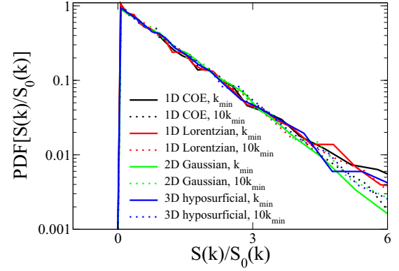
FIG. 31. Probability density function of the structure factor, normalized by the target, at two different wave vectors for four different targets. The two wave vectors are k_{\min} , the minimum wave vector in the x direction, and 10k_{\min} . The targets are 1D COE [Eq. (48)], 1D Lorentzian [Eq. (55)], 2D Gaussian [Eq. (59)], and 3D hyposurficial [Eq. (77)]. Since the structure factor is always exponentially distributed, the normalized plot for different cases falls on a single straight line on a plot on a semilogarithmic scale.
