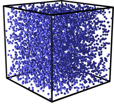
FIG. 23. Three-dimensional 4000-particle hyposurficial configuration drawn from ensembles in which the target function S_0(k) is taken to be Eq. (77) at \rho = \frac{1}{4\pi} .
