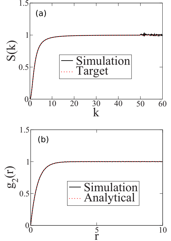
FIG. 5. (a) Structure factor obtained by sampling ensembles of 1D configurations in which the target function S_0(k) is taken to be Eq. (55) with \lambda = 2 at \rho = 1 . (b) Corresponding pair correlation function sampled from simulations and the analytical formula as obtained from (54) [ g_2(r) = 1 - \exp(-2r) ]. Here it turns out that our usual reciprocal-space cutoff of K = 30 is not large enough and so we use K = 50 instead.
