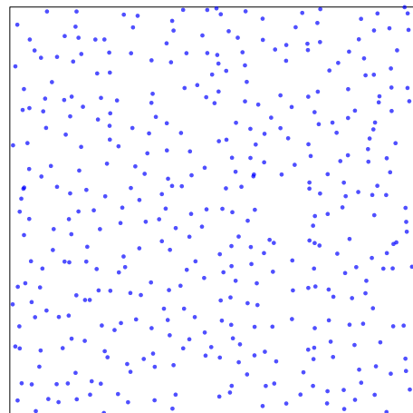
FIG. 8. Two-dimensional 400-particle Fermi-sphere configuration drawn from ensembles in which the target function S_0(k) is taken to be Eq. (56) at \rho = 1 .
