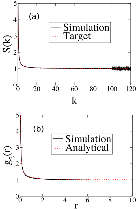
FIG. 24. (a) Structure factor obtained by sampling ensembles of 2D configurations, in which the target function S_0(k) is taken to be Eq. (78) at \rho = 1 and \kappa = 0 . (b) Corresponding pair correlation function sampled from simulations and the analytical formula (79).
