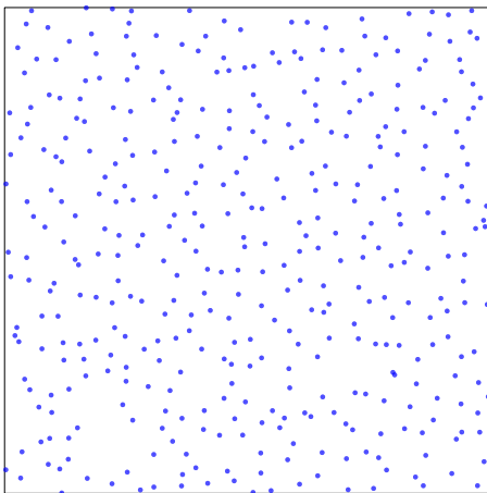
FIG. 10. Two-dimensional 400-particle OCP configuration drawn from ensembles in which the target function S_0(k) is taken to be Eq. (59) at \rho = 1 .
