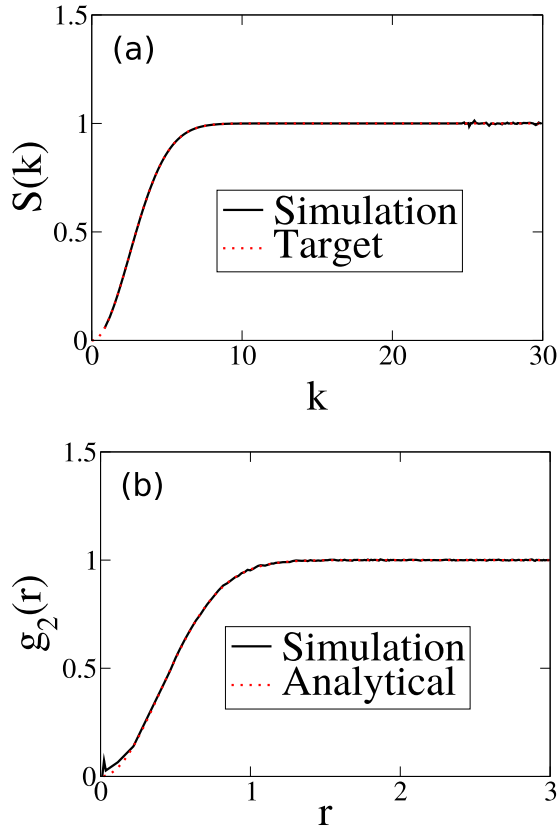
FIG. 13. (a) Structure factor obtained by sampling ensembles of 3D configurations in which the target function S_0(k) is taken to be Eq. (63) with a = 1/\sqrt{\pi} at \rho = 1 . (b) Corresponding pair correlation function sampled from simulations and the analytical formula (62). Here it turns out that our usual reciprocal-space cutoff of K = 15 is not large enough and so we use K = 25 instead.
