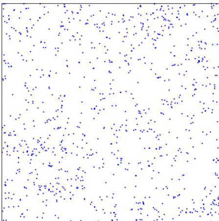
FIG. 25. Two-dimensional 1000-particle antihyperuniform configuration drawn from ensembles in which the target function S_0(k) is taken to be Eq. (78) at \rho = 1 and \kappa = 0 .
