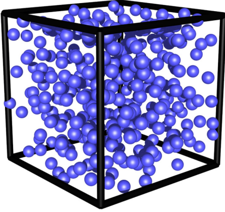
FIG. 16. Three-dimensional 400-particle configuration drawn from ensembles in which the target function S_0(k) is taken to be Eq. (65) at \rho = 1 .
