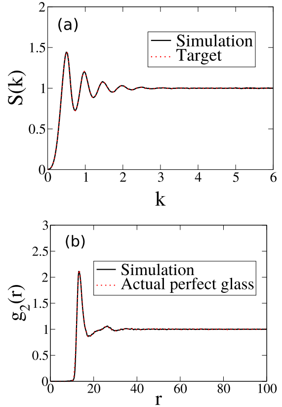
FIG. 26. (a) Structure factor obtained by sampling ensembles of 2D configurations in which the target function S_0(k) is taken to be equal to the numerically measured S(k) of a perfect-glass system at \rho = 0.003\,906\,25 . (b) Corresponding pair correlation function sampled from targeted configurations, compared with that of an actual perfect glass.
