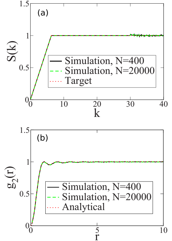
FIG. 3. (a) Structure factor obtained by sampling ensembles of 1D configurations in which the target function S_0(k) is taken to be Eq. (49) at \rho = 1 . We use two different system sizes and show here that their pair statistics are indistinguishable. For N = 20\,000 , we generate 100 configurations instead of the usual 5000 configurations. (b) Corresponding pair correlation function sampled from simulations and the analytical formula (52).
