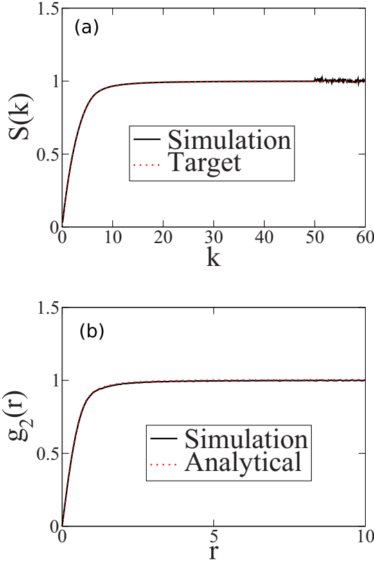
FIG. 2. (a) Structure factor obtained by sampling ensembles of 1D configurations in which the target function S_0(k) is taken to be Eq. (48) at \rho = 1 . (b) Corresponding pair correlation function sampled from simulations and the analytical formula (51). Here it turns out that our usual reciprocal-space cutoff of K = 30 is not large enough and so we use K = 50 instead.
