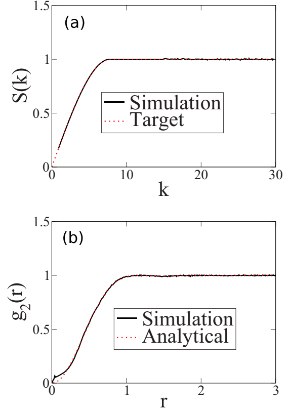
FIG. 7. (a) Structure factor obtained by sampling ensembles of 3D configurations in which the target function S_0(k) is taken to be Eq. (56) at \rho = 1 . (b) Corresponding pair correlation function sampled from simulations and the analytical formula (57).
