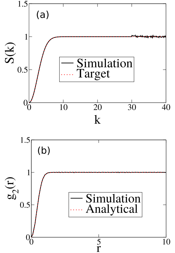
FIG. 12. (a) Structure factor obtained by sampling ensembles of 1D configurations in which the target function S_0(k) is taken to be Eq. (63) with a = 1/\sqrt{\pi} at \rho = 1 . (b) Corresponding pair correlation function sampled from simulations and the analytical formula (62).
