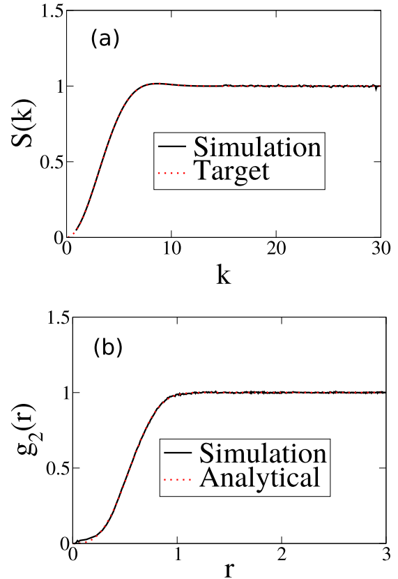
FIG. 15. (a) Structure factor obtained by sampling ensembles of 3D configurations in which the target function S_0(k) is taken to be Eq. (65) at \rho = 1 . (b) Corresponding pair correlation function sampled from simulations and the analytical formula (64).
