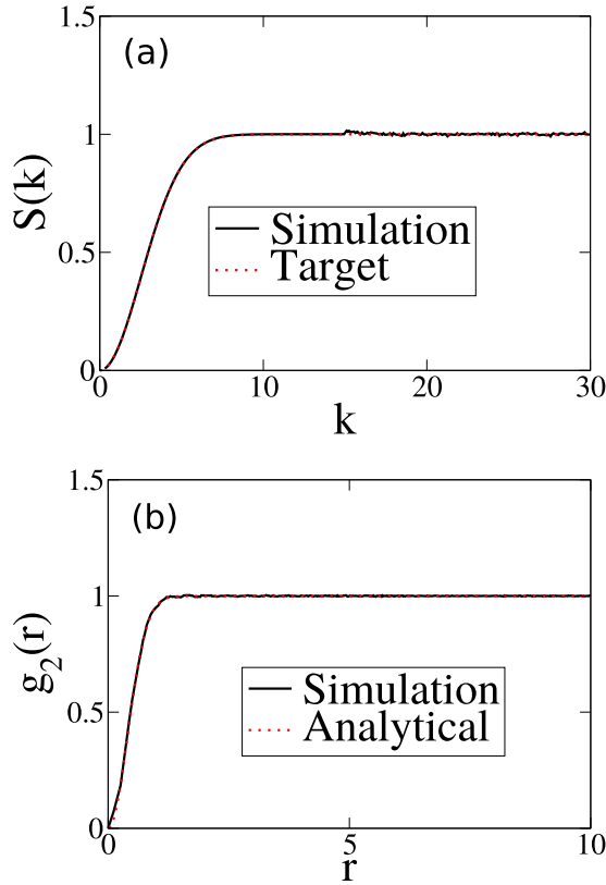
FIG. 9. (a) Structure factor obtained by sampling ensembles of 2D configurations in which the target function S_0(k) is taken to be Eq. (59) at \rho = 1 . (b) Corresponding pair correlation function sampled from simulations and the analytical formula (58).
