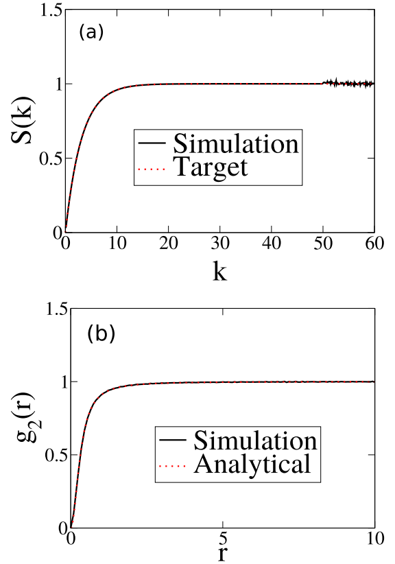
FIG. 17. (a) Structure factor obtained by sampling ensembles of 1D configurations in which the target function S_0(k) is taken to be Eq. (69) at \rho = 1 . (b) Corresponding pair correlation function sampled from simulations and the analytical formula (71). Here it turns out that our usual reciprocal-space cutoff of K = 30 is not large enough and so we use K = 50 instead.
