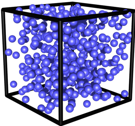
FIG. 14. Three-dimensional 400-particle configuration drawn from ensembles in which the target function S_0(k) is taken to be Eq. (63) at \rho = 1 .
