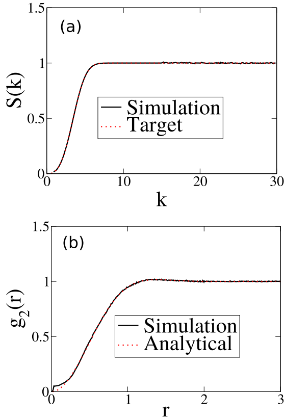
FIG. 18. (a) Structure factor obtained by sampling ensembles of 3D configurations in which the target function S_0(k) is taken to be Eq. (69) at \rho = 1 . (b) Corresponding pair correlation function sampled from simulations and the analytical formula (73).
