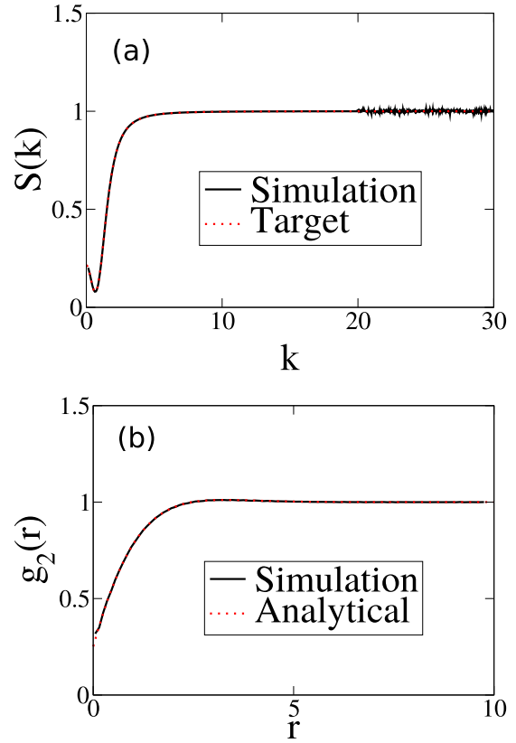
FIG. 20. (a) Structure factor obtained by sampling ensembles of 2D configurations, in which the target function S_0(k) is numerically computed from Eqs. (2) and (75), at \rho = 0.5 . (b) Corresponding pair correlation function sampled from simulations and the analytical formula (75).
