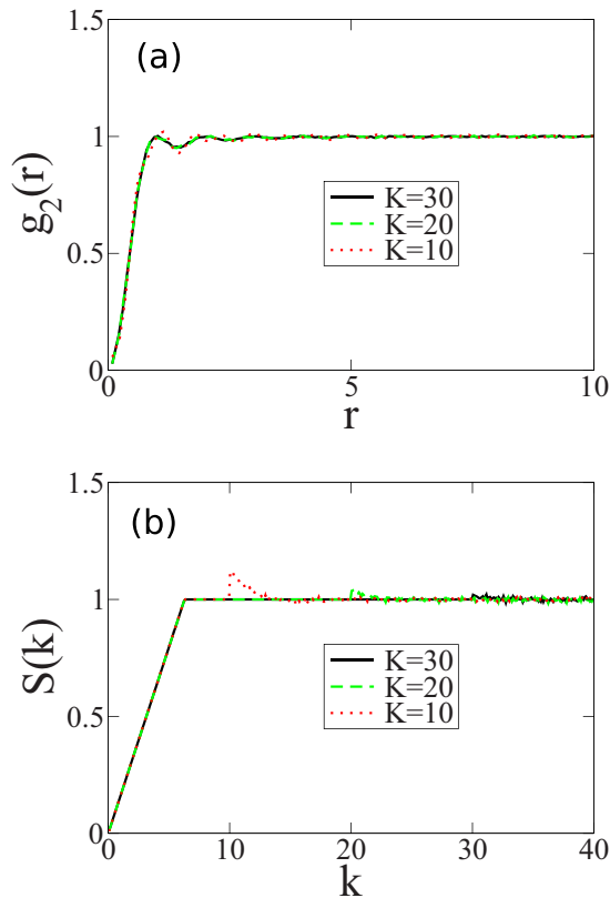
FIG. 32. Pair correlation function and structure factor obtained by targeting Eq. (49) at various values of K .
