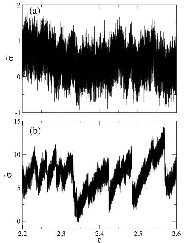
FIG. 3. (a) Section of the stress-strain curve for the lowest-density state point on the higher-temperature isomorph ( \rho = 1.265 , T = 0.550 ) at the lowest nominal strain rate 10^{-5} . (b) Section of the stress-strain curve for a state point on the lower-temperature isomorph ( \rho = 1.324 , T = 0.100 ) at the lowest strain rate 10^{-5} . The abrupt drops can be identified with avalanches of plastic activity. The difference in vertical scale between (a) and (b) can be attributed partly to the definition of reduced units for stress.
