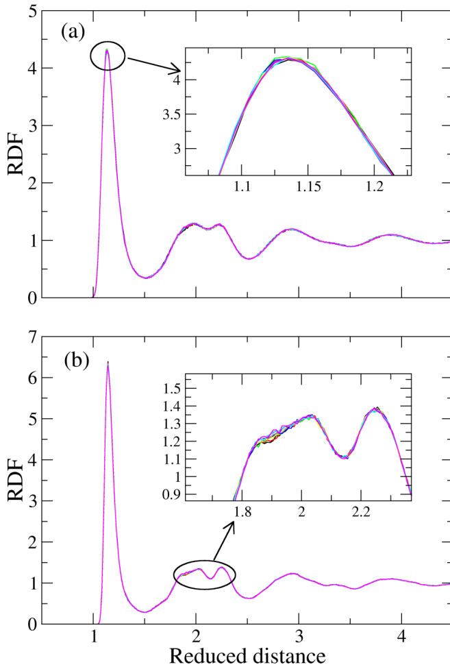
FIG. 2. Radial distribution function (RDF) for the large ( A ) particles in reduced units along glassy isomorphs starting at (a) T = 0.55 and (b) T = 0.1 . Each figure shows ten curves, where the density is increased by 1% for each state point, giving a 9.4% change in density overall; the temperature increases by 54% overall. The insets show close-ups of (a) the first peak and (b) the second peak, where very small deviations are discernible.
