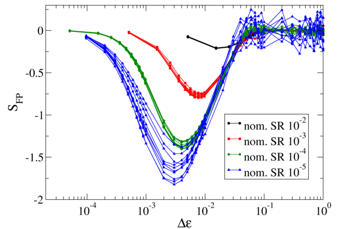
FIG. 9. Fisher-Pearson skewness S_{\text{FP}} of (reduced) stress drop distributions as a function of strain interval for different strain rates for the low-temperature isomorph. Different curves of the same color correspond to different points on the isomorph.
