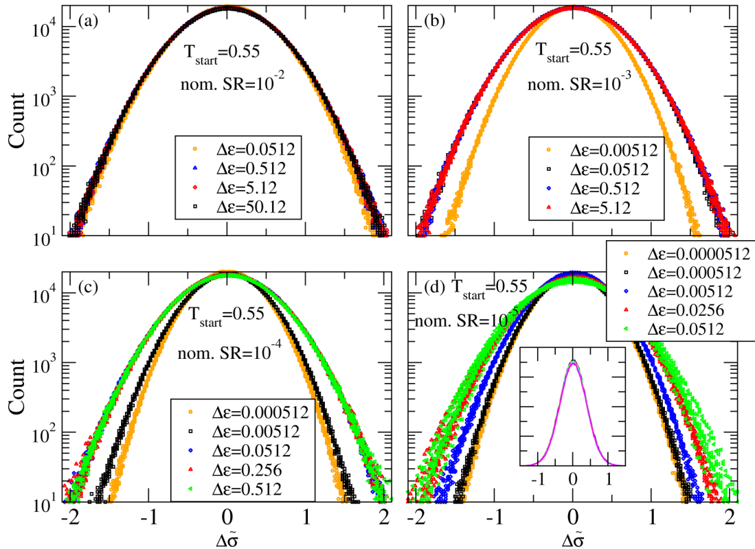
FIG. 7. Histograms of stress changes of intervals as indicated for the high-temperature isomorph for different strain rates. For each strain rate and \Delta\varepsilon , distributions from the ten members of the isomorph are plotted in the same color. The fact that they appear as one curve for each color, apart from broadening due to statistical noise at the lowest strain rates, indicates a high degree of collapse. The distributions are essentially Gaussian for all strain rates and strain intervals \Delta\varepsilon , and their widths are relative insensitive to \Delta\varepsilon even at the lowest strain rates, indicating that most of the fluctuations are thermal rather than strain driven. The inset in (d) shows an alternative way of exhibiting isomorph invariance for \Delta\varepsilon = 0.000512 , by coloring different members of the isomorph differently, and on a linear scale.
