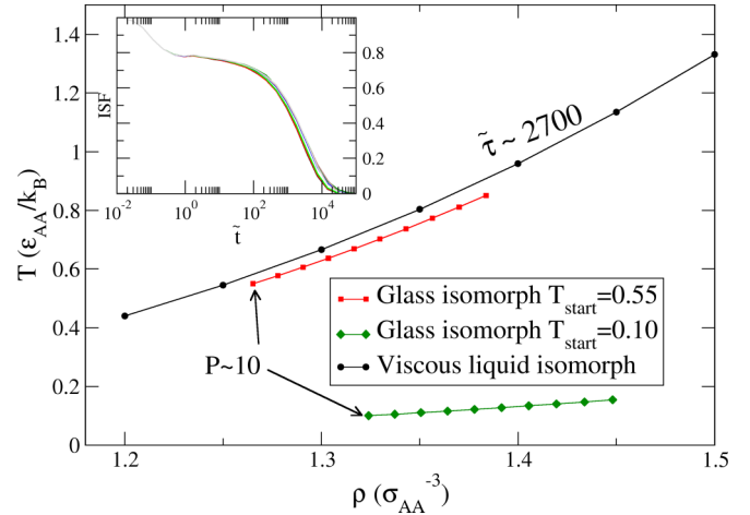
FIG. 1. Black symbols indicate an isomorph in the supercooled liquid which includes the point (\rho = 1.2, T = 0.44) . We use this as a guide to locating the glass transition; its relaxation time is about 2700 in reduced units, corresponding to 3850 in LJ units at the lowest density 1.2. The inset shows the intermediate scattering function for the different state points, lying almost on top of each other. The red and green symbols indicate isomorphs generated in the glass which we use for studying deformation, referred to as those starting at temperatures T = 0.55 and 0.1 , respectively. Note that the starting densities are not the same, since these are taken from a cooling run at fixed pressure P = 10 .
