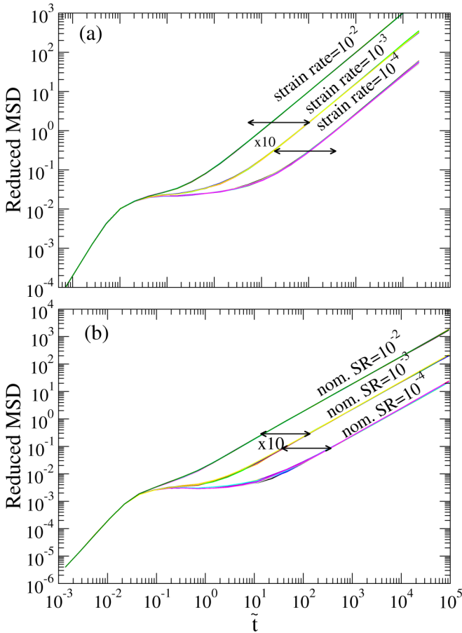
FIG. 12. Mean-square transverse displacement plotted in reduced units for (a) the high-temperature isomorph and (b) the low-temperature isomorph. The horizontal arrows indicate a factor of 10 in the time axis and can be used to judge by what factor the curves can be shifted onto each other in time.
