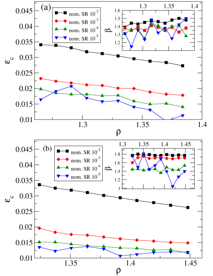
FIG. 6. Fits of shear stress autocorrelation to Eq. (6) shown as functions of density along the (a) high- and (b) low-temperature isomorphs. The characteristic strain over which decays occurs, \varepsilon_c , decreases approximately linearly as density increases.
