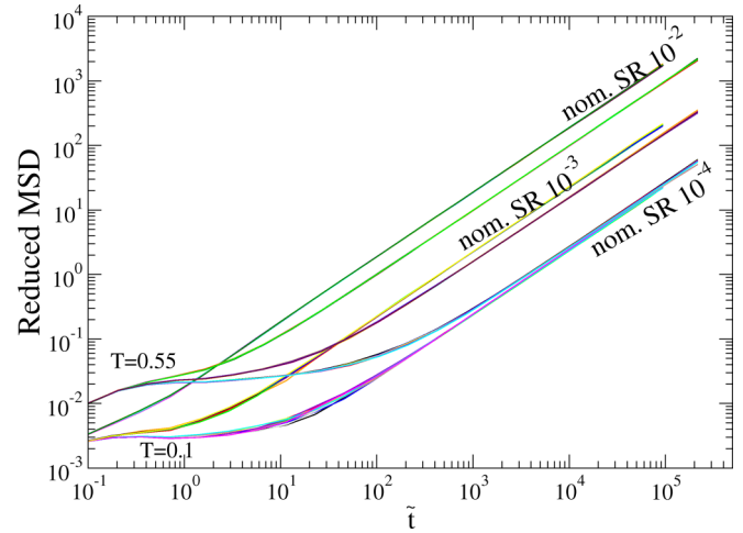
FIG. 13. The MSD curves from Figs. 12(a) and 12(b) plotted together, though without the short-time parts. At low strain rates the MSD appears to become independent of the isomorph, as well as which point on the isomorph. The definition of reduced units means that the curves for the different isomorphs are plotted in terms of different timescales, so caution is required when drawing conclusions from the apparent collapse.
