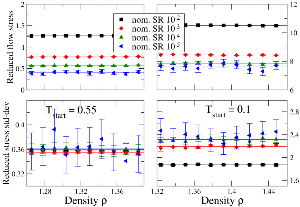
FIG. 4. Flow stress and standard deviation during the steady-state regime as a function of density along high-temperature isomorphs (left panels) and low-temperature isomorphs (right panels) for different strain rates. The legend indicates the nominal strain rates, that is, the real strain rates at the first point on each isomorph; for other state points in each data set, the reduced unit strain rate is the same. Error bars have been calculated as the error of the mean and of the standard deviation, assuming the data are normally distributed [see Eq. (4.14) and Appendix E of Ref. [40]]. We choose the effective number of data points to be the total steady-state strain divided by 0.05; we believe data points are statistically independent for strain increments of 0.05. The horizontal lines indicate the mean value for the isomorph.
