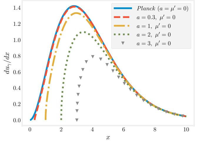
FIG. 1. Photon energy density in the units of T^4/\pi^2\hbar^3c^3 versus normalized frequency x = \hbar\omega/T for different values of parameter a and \mu' = 0 . Blackbody Planck density corresponding to a = \mu' = 0 is also shown for comparison.
