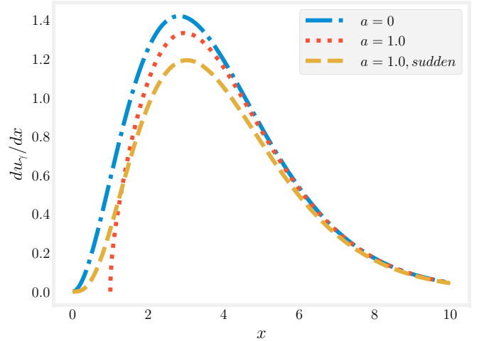
FIG. 4. Photon spectral energy density in the units of T^4/\pi^2\hbar^3c^3 versus normalized frequency x = \hbar\omega/T for a = 1 , \mu = 0 before and after sudden recombination and for a blackbody of the same temperature with a = 0 , \mu = 0 .
