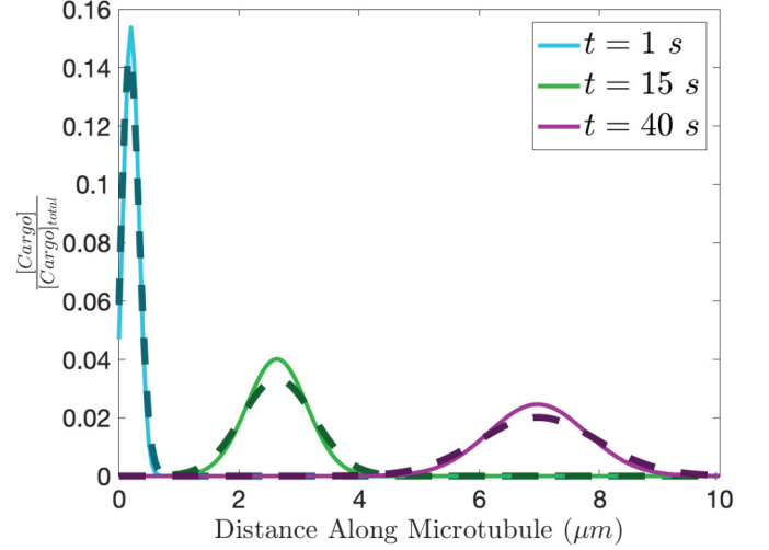
FIG. 5. Comparison of steady-state computational scheme (dashed line) and analytic scheme (solid line) defined by Eq. (14). Constants used: N = 10 , L = 10 \mu\text{m} , v_{\text{trans}} = 1 \mu\text{m s}^{-1} , \delta_R = 0.9 , k_{\text{on}} = 0.2 \text{ s}^{-1} , k_{\text{off}} = 1 \text{ s}^{-1} , D_{\text{cargo}} = 0.01 \mu\text{m}^2 \text{ s}^{-1} , and D_{\text{motor}} = 10 \mu\text{m}^2 \text{ s}^{-1} .
