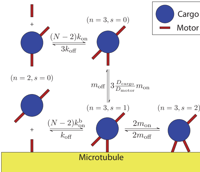
FIG. 1. Binding diagram for reactions considered. See Eqs. (A2)–(A5) for general reaction rates.
