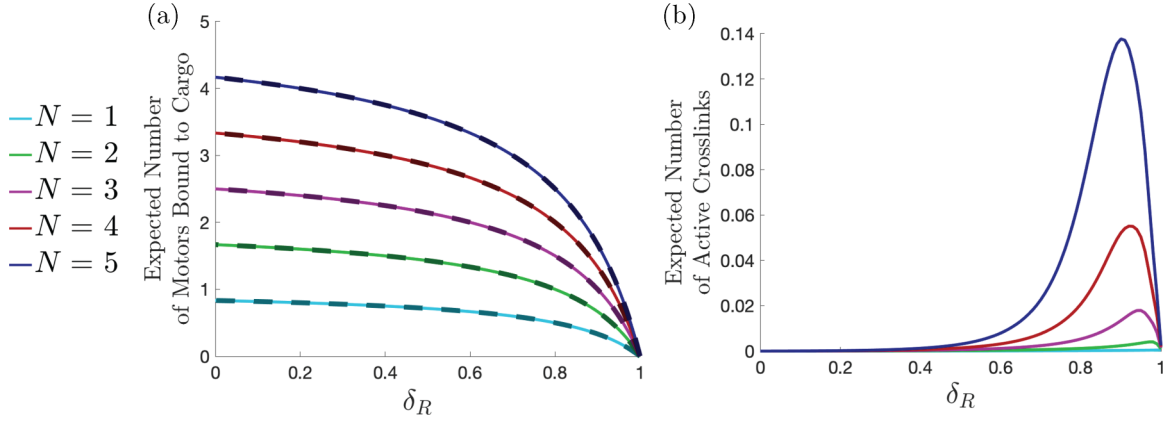
FIG. 4. The average number of motors and average number of engaged motors at steady state. Solid lines denote the QSS solution and dashed lines denote the computational solution. (a) Expected number of motors on cargo. (b) Expected number of motors bound to both cargo and MT. Same parameter values as used in Fig. 2.
