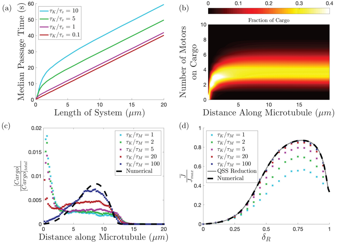
FIG. 3. The effect of timescale separation on transport efficiency. (a) The median time to reach the end of the system. (b) The distribution of motors on the cargo n (at the median time) as a function of distance along the MT. (c), (d) Convergence between the Monte Carlo simulation and computational PDE solution as quasi-steady-state assumption is taken. Constants used are N = 10 , D_{cargo} = 0.014 \mu\text{m}^2 \text{s}^{-1} , D_{motor} = 1.4 \mu\text{m}^2 \text{s}^{-1} , v_{trans} = 0.5 \mu\text{m s}^{-1} , \delta_R = 0.9 , k_{on} = 0.5 \text{s}^{-1} , k_{off} = 0.1 \text{s}^{-1} .
