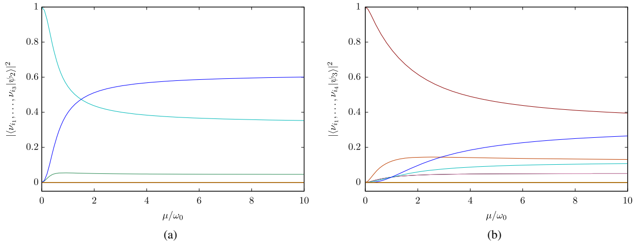
FIG. 4. Overlaps, |\langle \nu_{i_1}, \dots, \nu_{i_N} | \psi_n \rangle|^2 , of an excited state |\psi_n\rangle with the mass basis states (with i_1, \dots, i_N = 1, 2 ), for systems with different sizes N . Here, the n th energy eigenstate |\psi_n\rangle ( n = 0, \dots, 2^N - 1 ) is connected to the mass eigenstate |\nu_{j_1}, \dots, \nu_{j_N}\rangle in the limit \mu \rightarrow 0 , where j_{N-k+1} = 1 + (k th digit of n in binary representation). Observe that a state with a given \kappa has {}^N C_\kappa nontrivial components for \mu > 0 . (a) Mass-basis decomposition for the state |\psi_2\rangle in the N = M = 3 system, as a function of \mu ; this state has \kappa = 1 . (b) Mass-basis decomposition of the state |\psi_3\rangle in the N = M = 4 system, as a function of \mu ; this state has \kappa = 2 . Two of the six nontrivial overlaps are numerically indistinguishable in (b).
