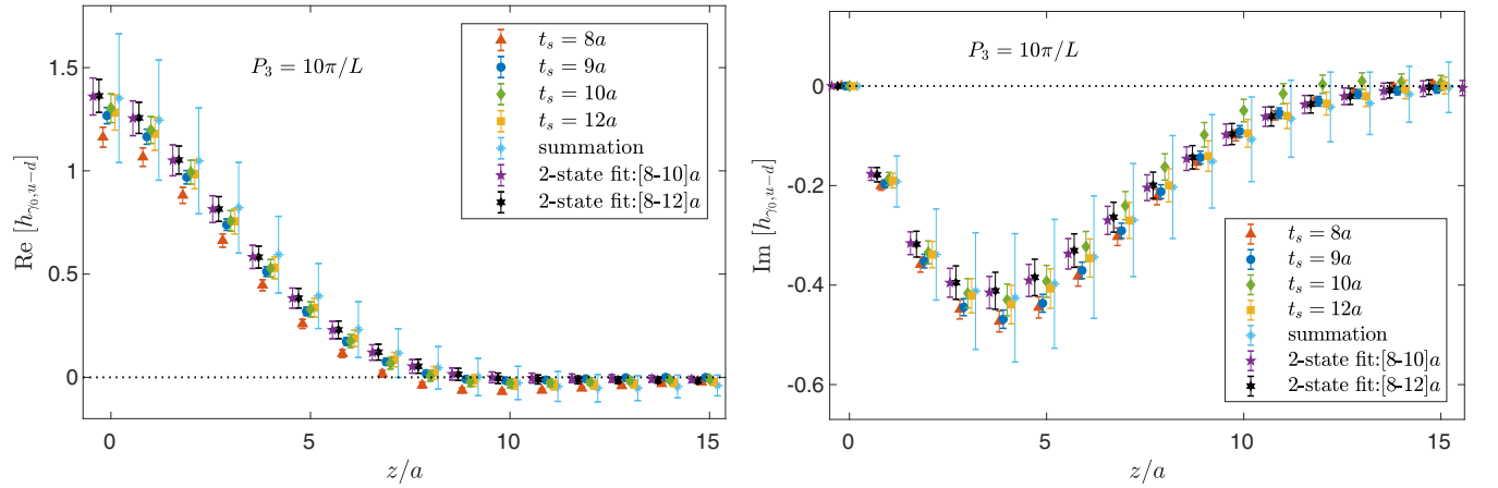
FIG. 13. Real (left) and imaginary (right) parts of the matrix element for the unpolarized PDF from the plateau method (points labeled with appropriate t_s ), the summation method (using t_s \geq 9a ) and sequential two-state fits (to t_s = 8a, 9a, 10a and to all t_s ). The nucleon is boosted with 10\pi/L \simeq 1.38 GeV.
