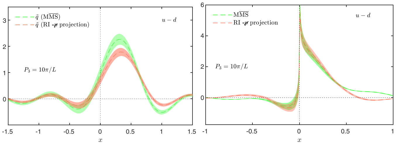
FIG. 26. Left panel: Comparison of renormalized quasi-PDFs in the RI scheme with \not{x} projection (red band) and the \overline{\text{MS}} scheme (green band). Right panel: Matched PDFs obtained from the same bare matrix elements, but with different scheme conversion, evolution and matching procedures: either one-step (RI \rightarrow \overline{\text{MS}} ) or two-step (RI \rightarrow \overline{\text{MS}} \rightarrow \overline{\text{MS}} ) (see text for details). This is for the unpolarized case, with a nucleon momentum of P_3 = 10\pi/L .
