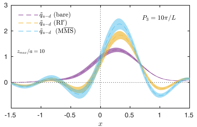
FIG. 29. The unpolarized quasi-PDFs for P_3 = 10\pi/L . We show the bare matrix element (purple), RI' (yellow) and \overline{\text{MMS}} (cyan) quasi-PDFs for z_{\max} = 10a .
