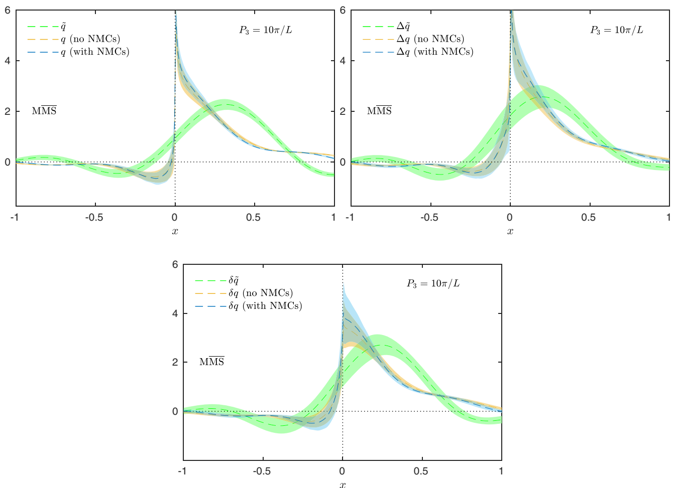
FIG. 31. Effect of matching and nucleon mass corrections in the unpolarized PDF (upper left), helicity PDF (upper right) and transversity PDF (lower). The nucleon momentum is P_3 = 10\pi/L for all plots.
