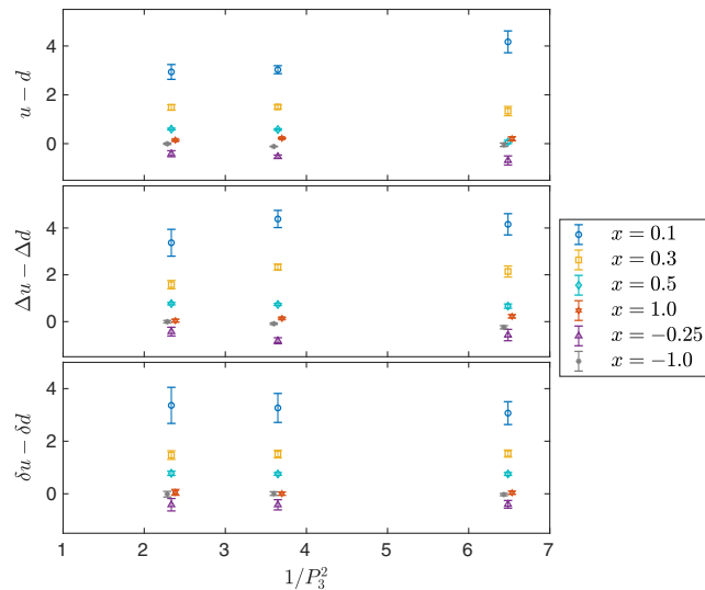
FIG. 33. Dependence of the unpolarized PDF (upper), helicity PDF (middle) and transversity PDF (lower) on the nucleon momentum for six selected values of x .
